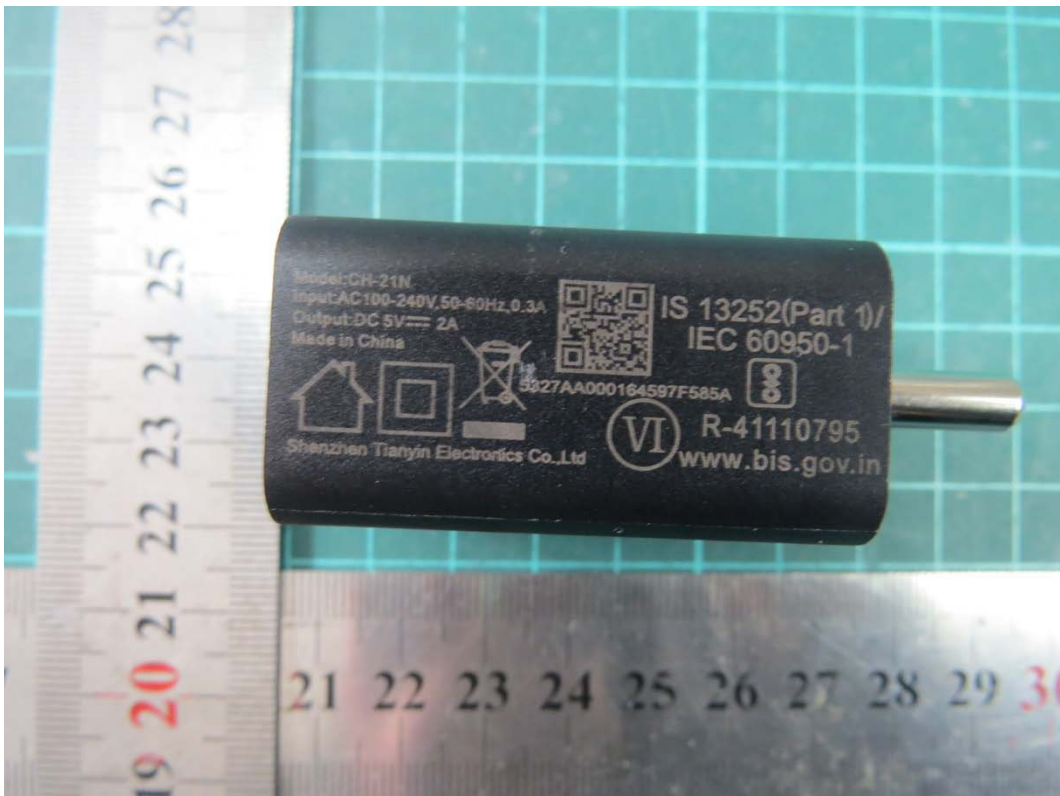
Adapter 4
