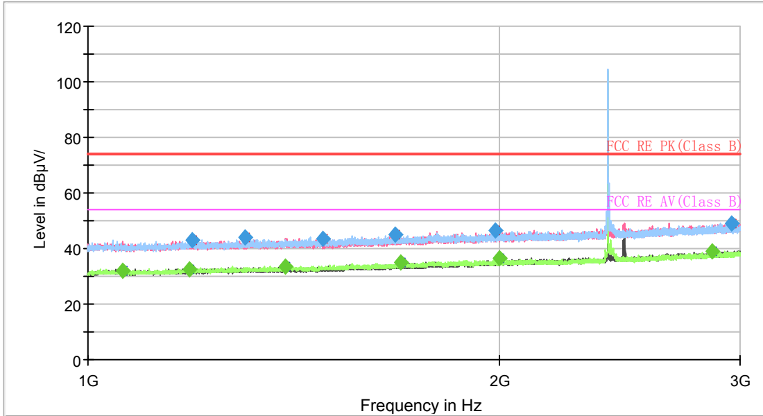
Note: The signal beyond the limit is carrier. Radiates Emission from 1GHz to 3GHz
