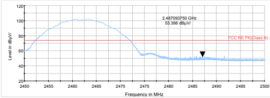
802.11b-Channel 11 Peak
