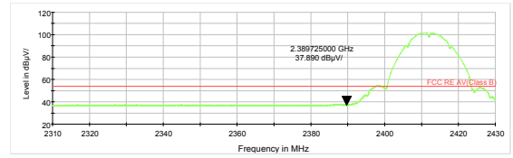
802.11b-Channel 1 Average
