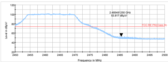
802.11g-Channel 11 Peak
