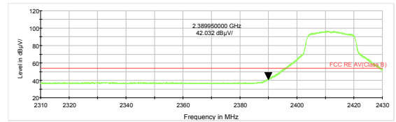
802.11g-Channel 1 Average
