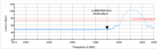
802.11b-Channel 1 Peak
