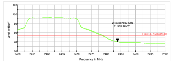
802.11g-Channel 11 Average
