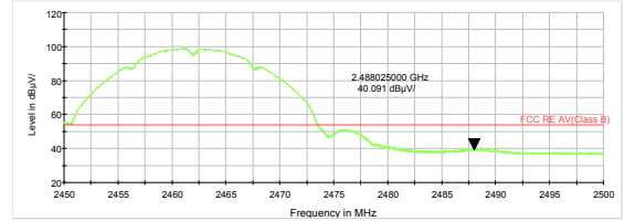
802.11b-Channel 11 Average
