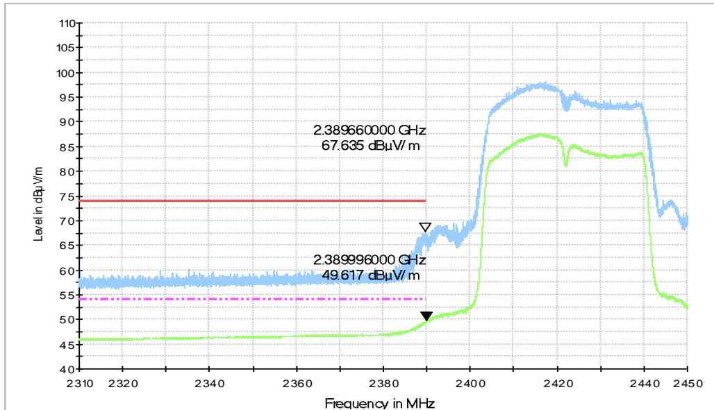
RE - Power-2.31GHz-2.45GHz
