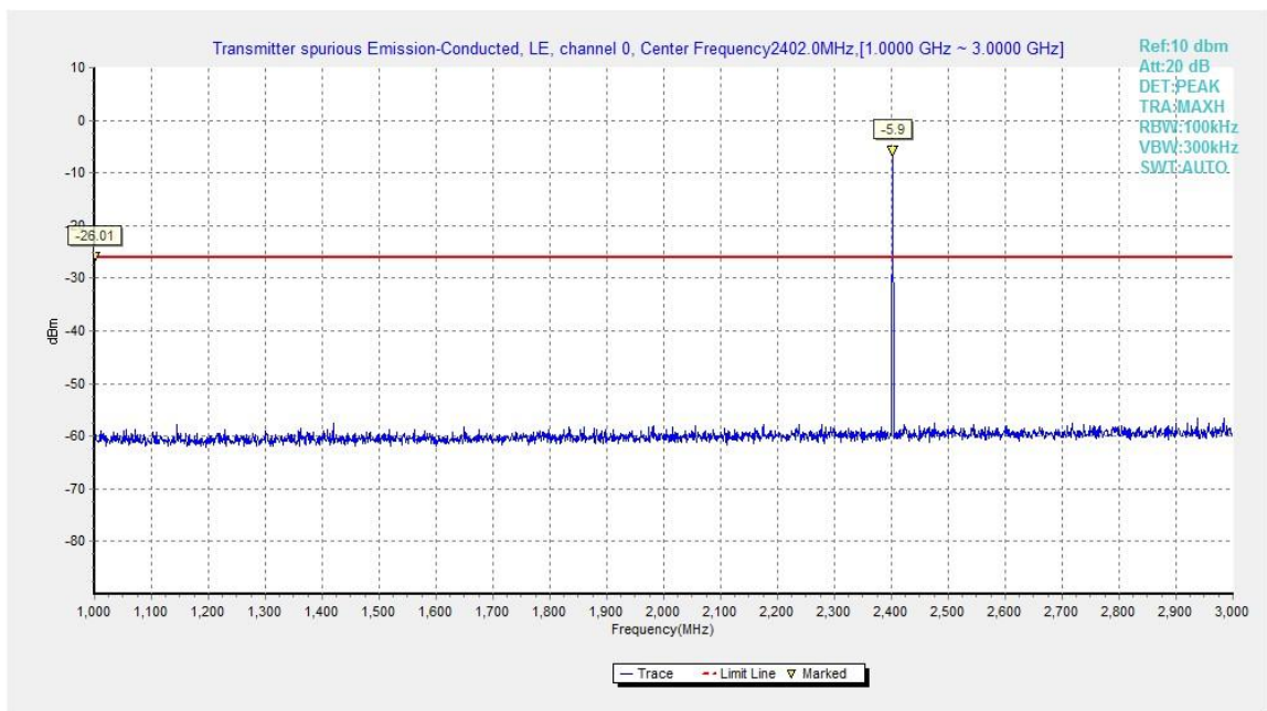
Fig.5. Transmitter Spurious Emission - Conducted: GFSK, 2402 MHz,1GHz - 3GHz
