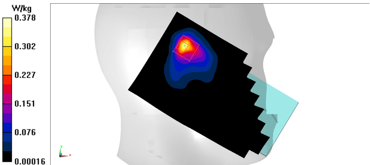
Fig.23 2450 MHz
