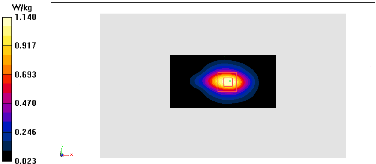
Fig.22 LTE Band66
