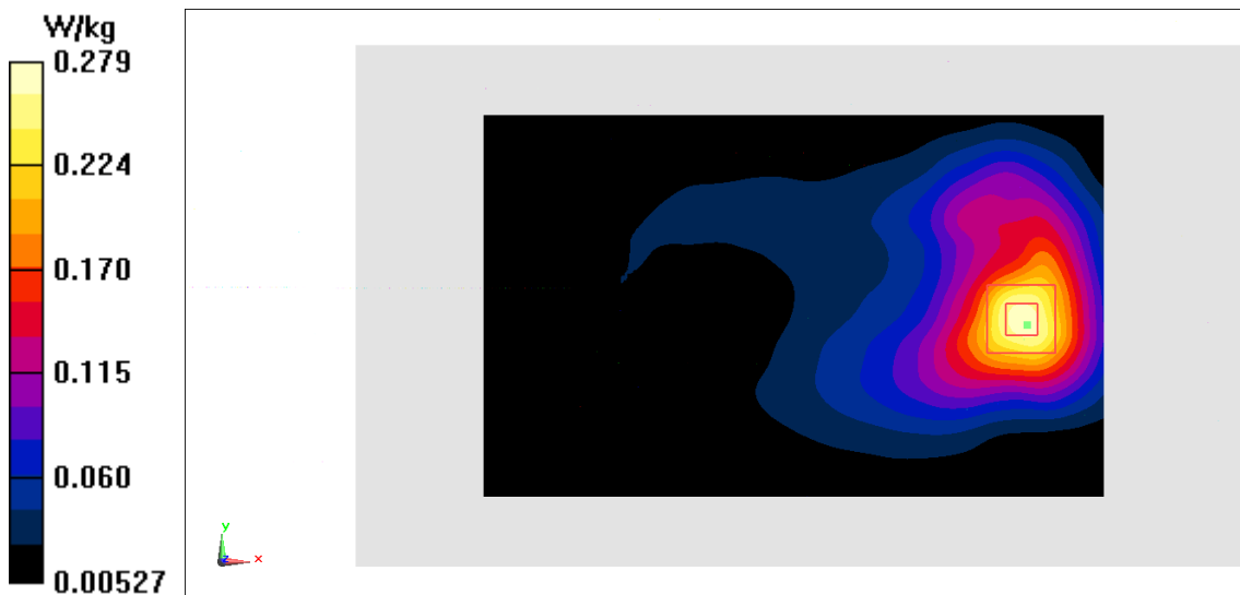
Fig.4 1900 MHz
