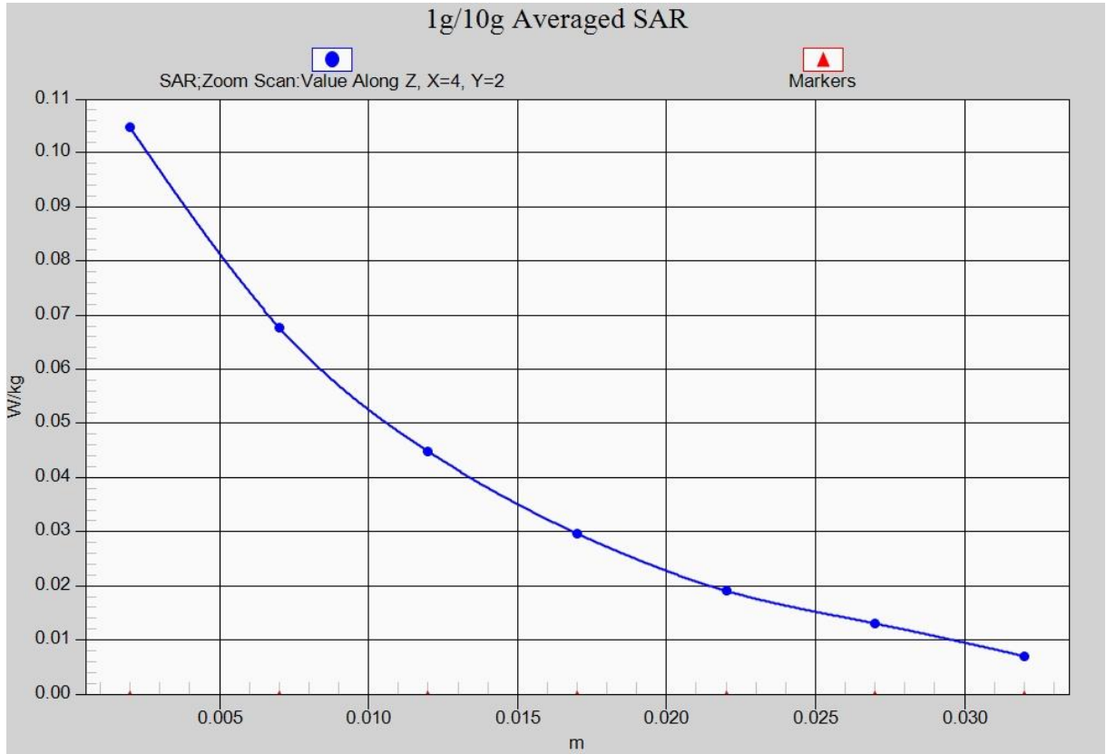
Fig. 21-1 Z-Scan at power reference point (LTE Band66)
