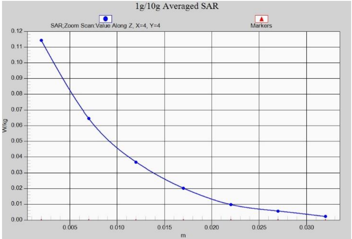
Fig. 19-1 Z-Scan at power reference point (LTE Band 38)
