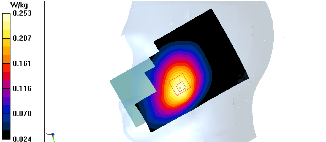
Fig.1 850MHz
