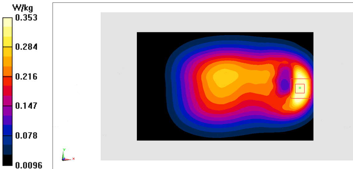
Fig.2 850 MHz
