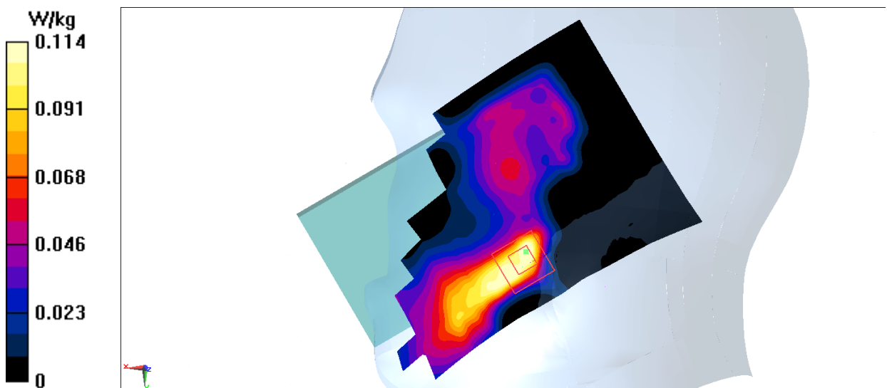
Fig.19 LTE Band 38
