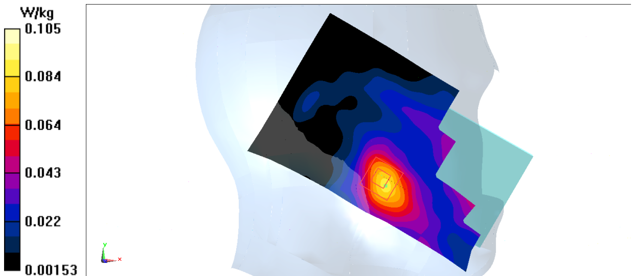
Fig.21 LTE Band66
