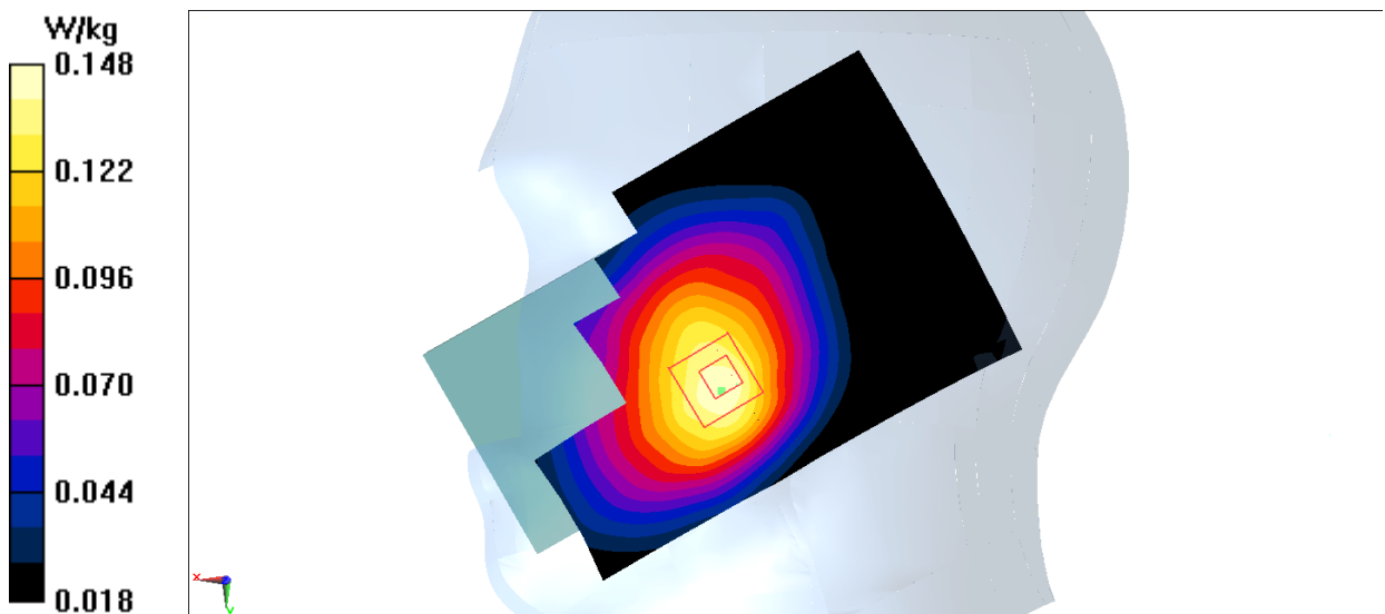
Fig.17 LTE Band12
