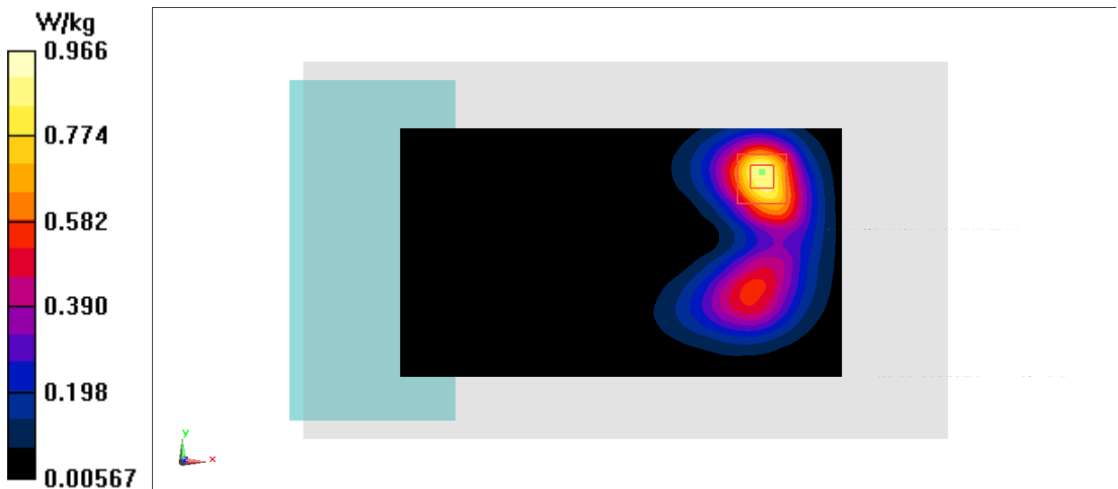
Fig.20 LTE Band 38
