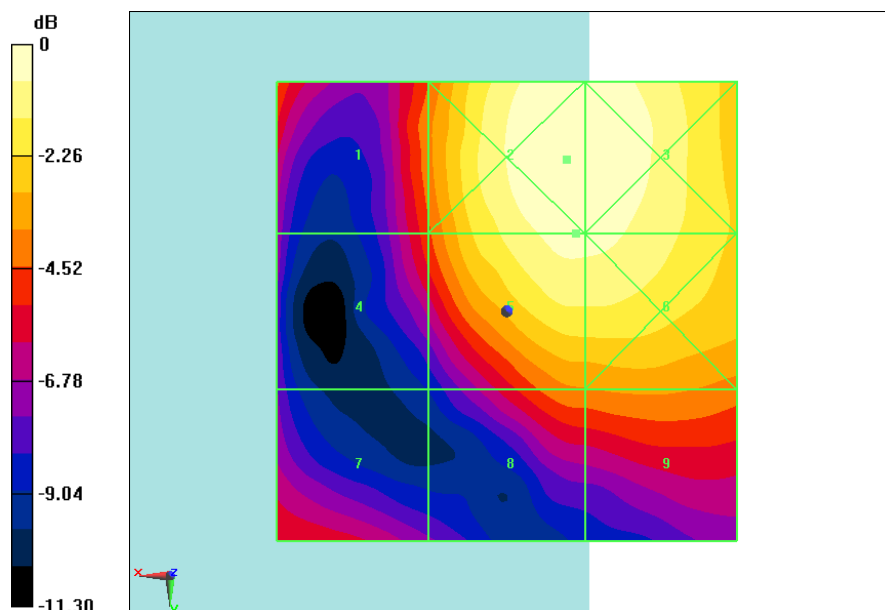
Fig B.15 HAC RF E-Field LTE Band38 64QAM CH38750
