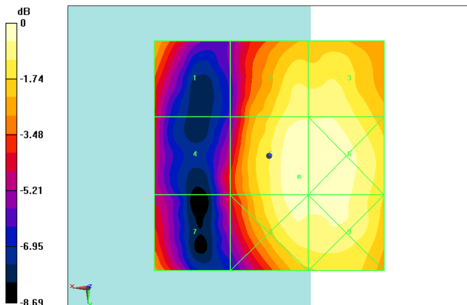
Fig B.8 HAC RF E-Field LTE Band38 QPSK CH38000
