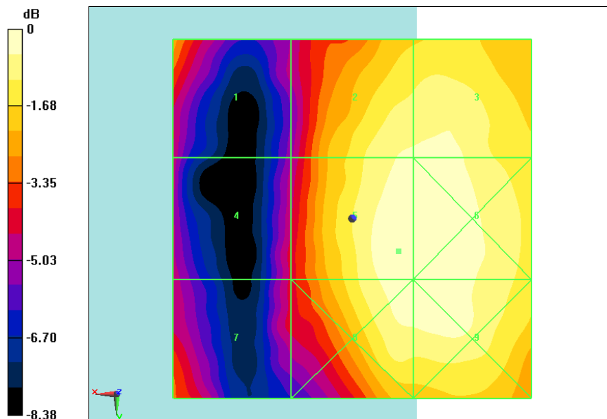
Fig B.12 HAC RF E-Field LTE Band38 16QAM CH37850
