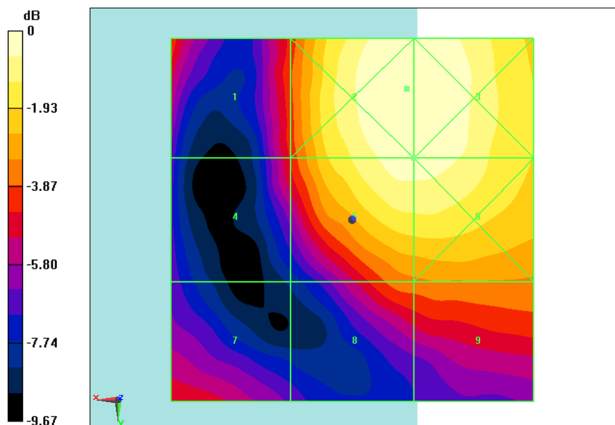
Fig B.14 HAC RF E-Field LTE Band38 64QAM CH38000
