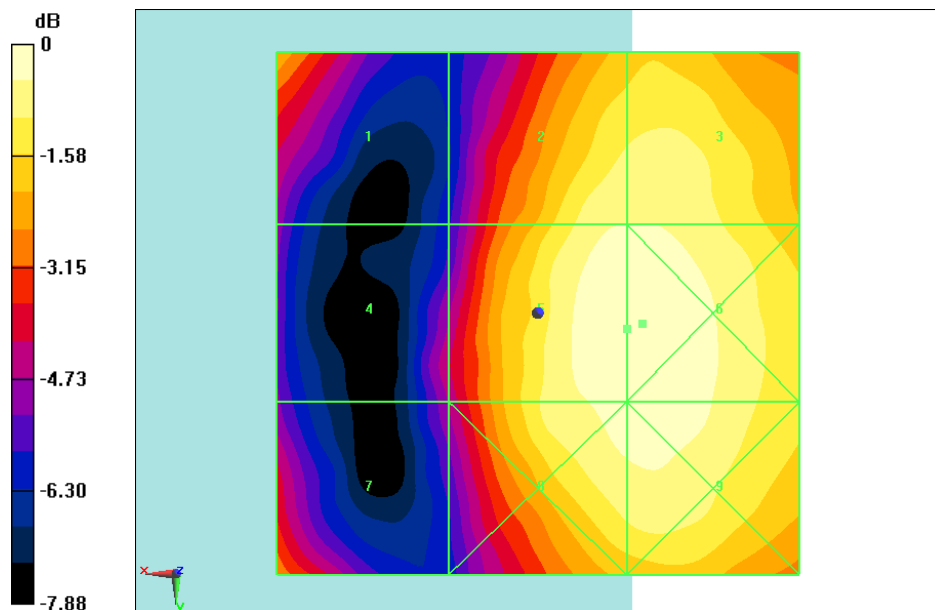
Fig B.7 HAC RF E-Field LTE Band38 QPSK CH38150
