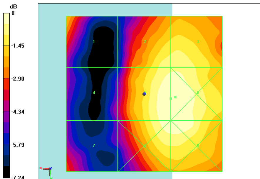
Fig B.10 HAC RF E-Field LTE Band38 16QAM CH38150
