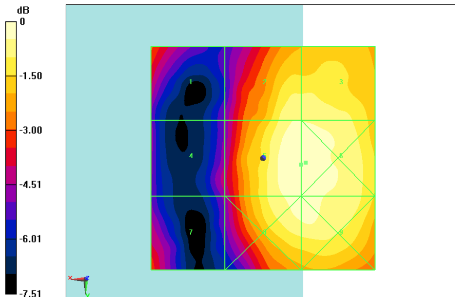
Fig B.9 HAC RF E-Field LTE Band38 QPSK CH37850
