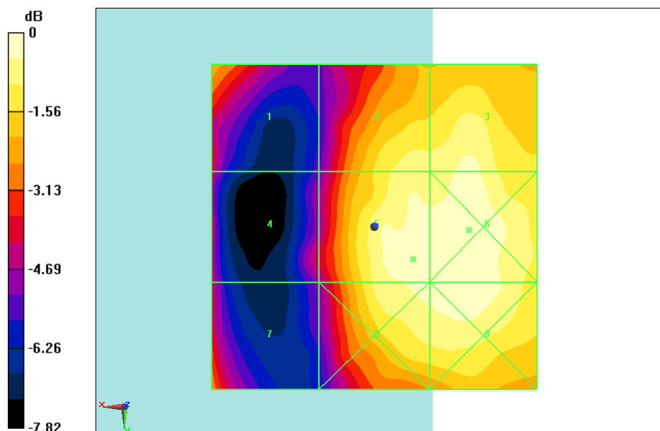
Fig B.11 HAC RF E-Field LTE Band38 16QAM CH38000
