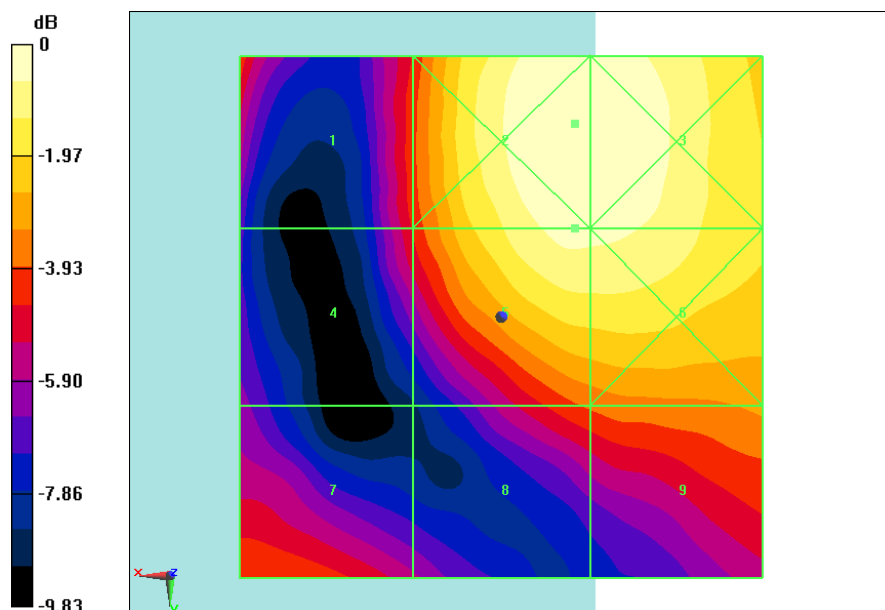
Fig B.13 HAC RF E-Field LTE Band38 64QAM CH38150
