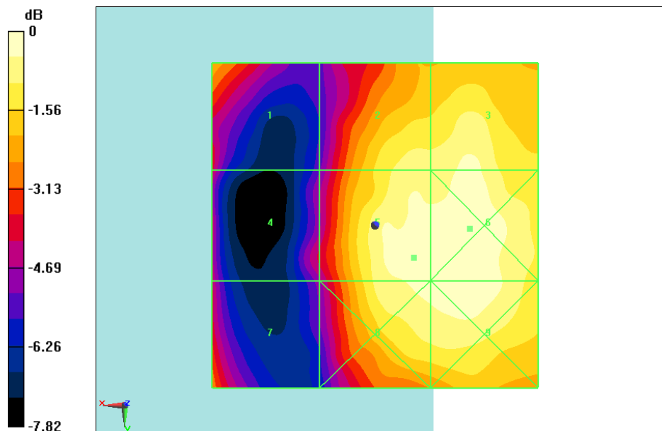
Fig B.11 HAC RF E-Field LTE Band38 16QAM CH38000
