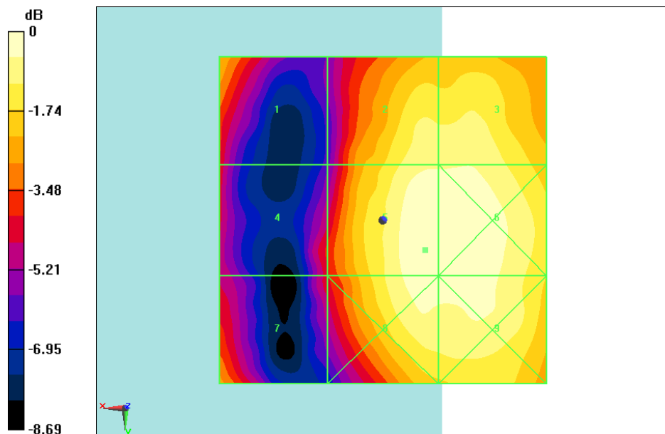
Fig B.8 HAC RF E-Field LTE Band38 QPSK CH38000
