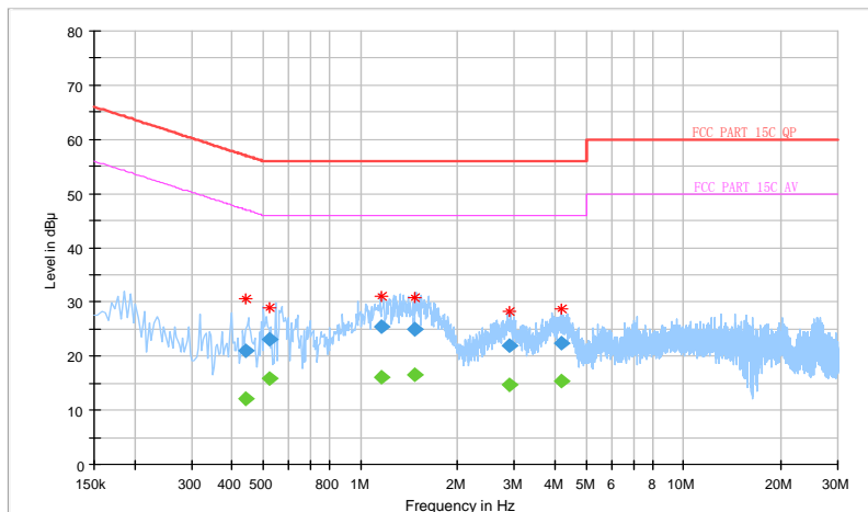
Full Spectrum
