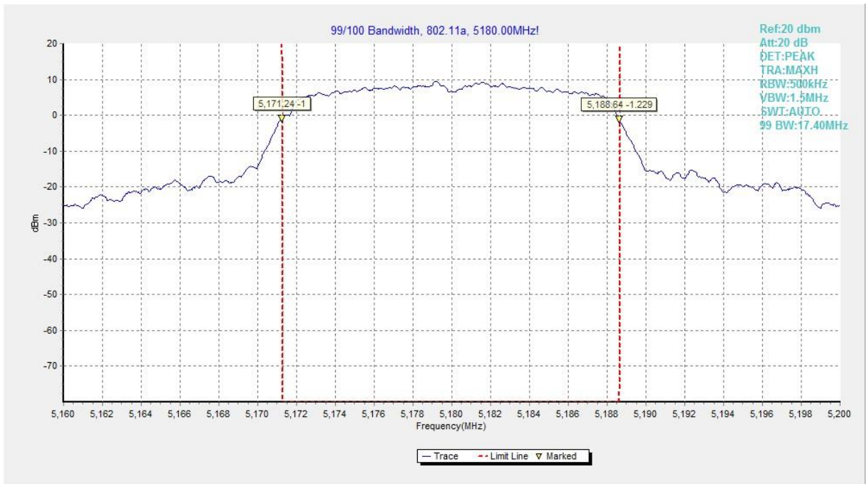
Fig. 40 99% Occupied bandwidth (802.11a, 5180MHz)
