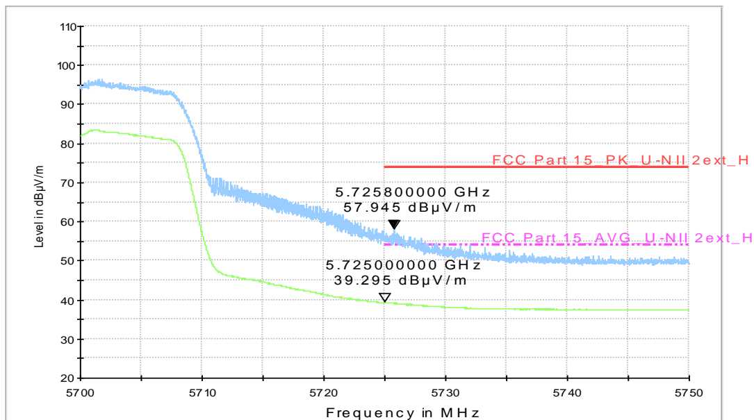
RE - Power-5.7GHz-5.75GHz
