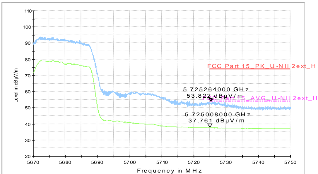
RE - Power-5.7GHz-5.75GHz
