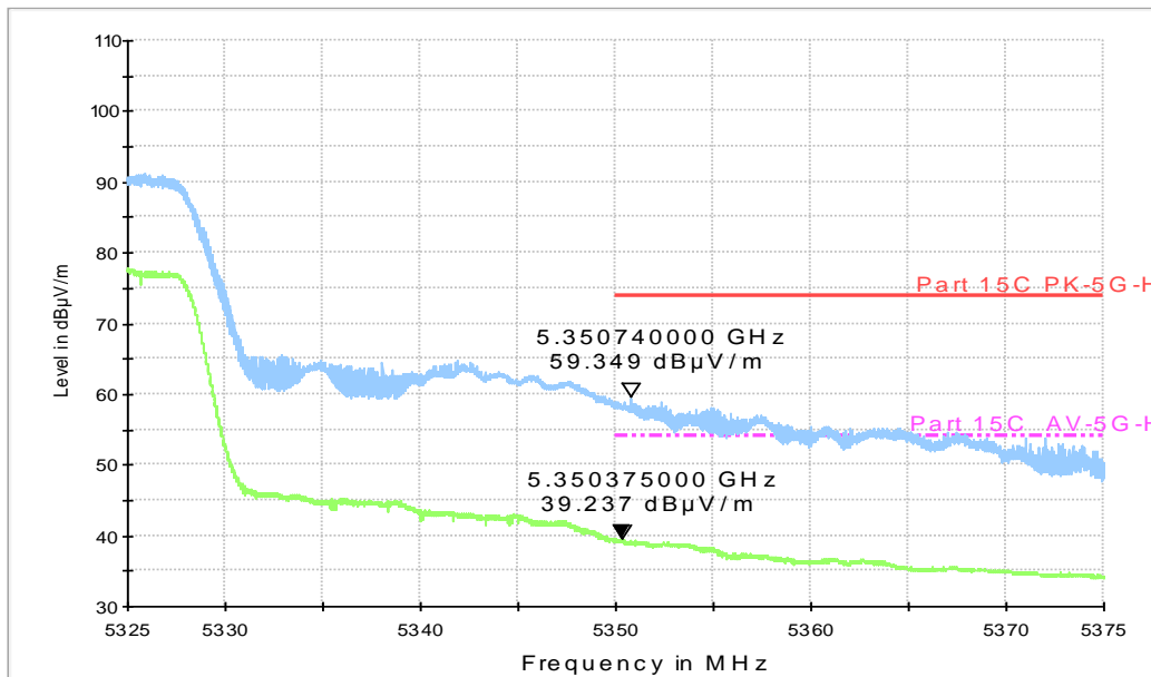
RE - Power-5.325GHz-5.375GHz
