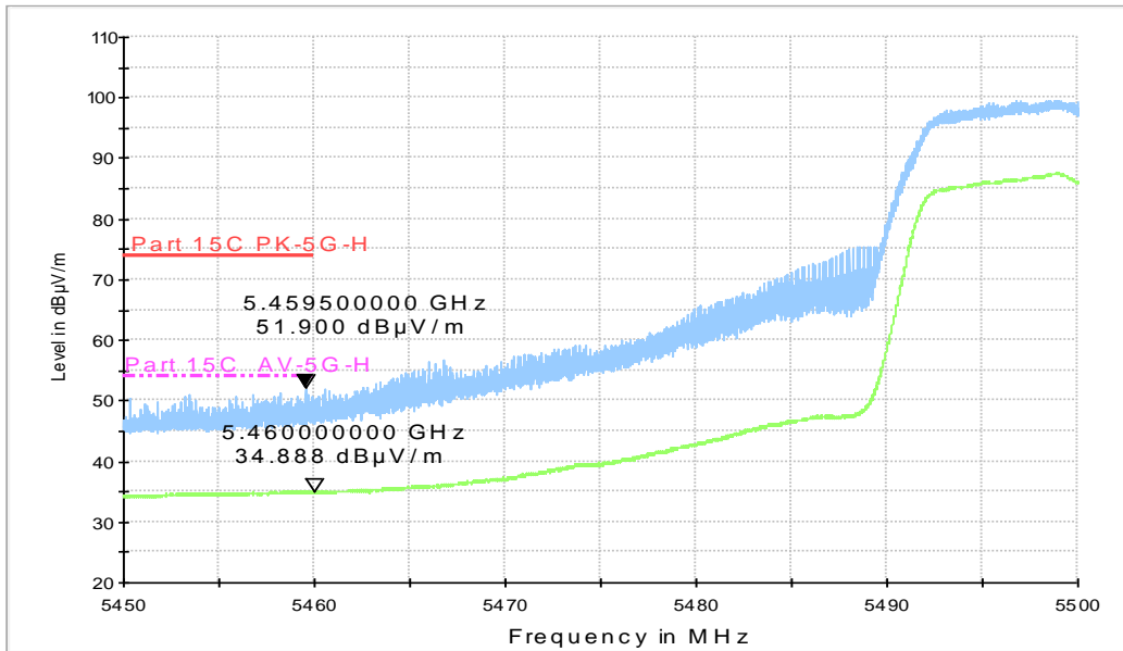
RE - Power-5.45GHz-5.50GHz
