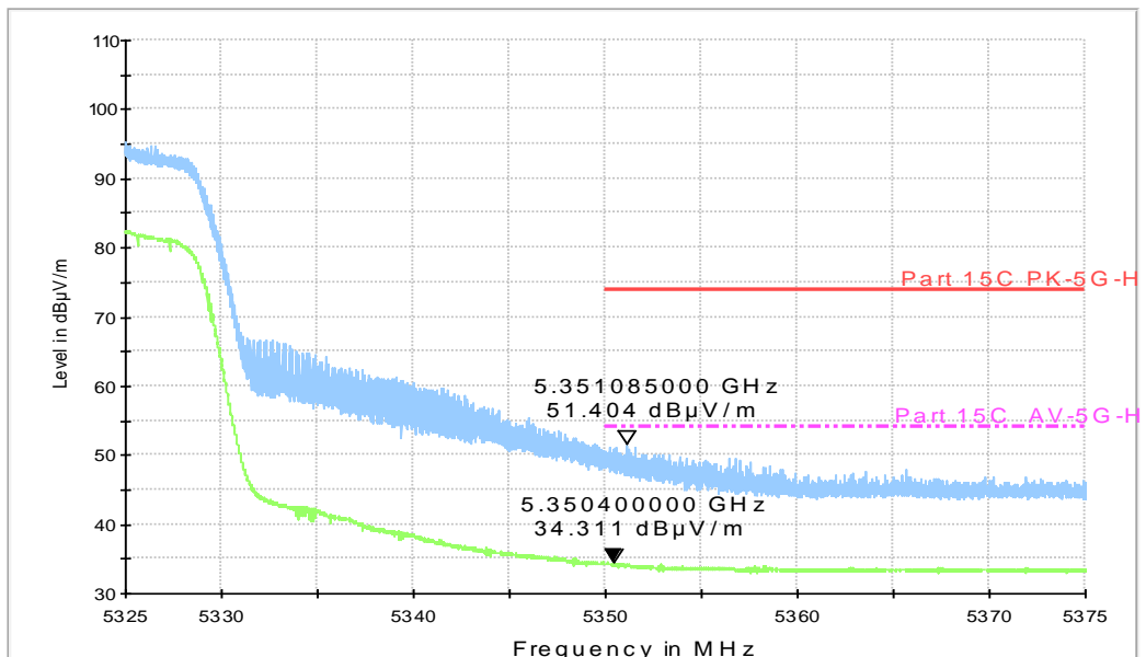
RE - Power-5.325GHz-5.375GHz
