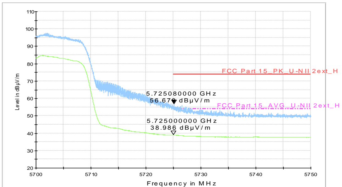
RE - Power-5.7GHz-5.75GHz
