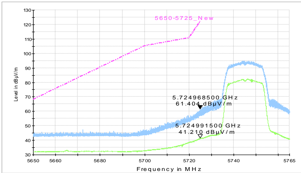
RE - Power-5.650GHz-5.765GHz
