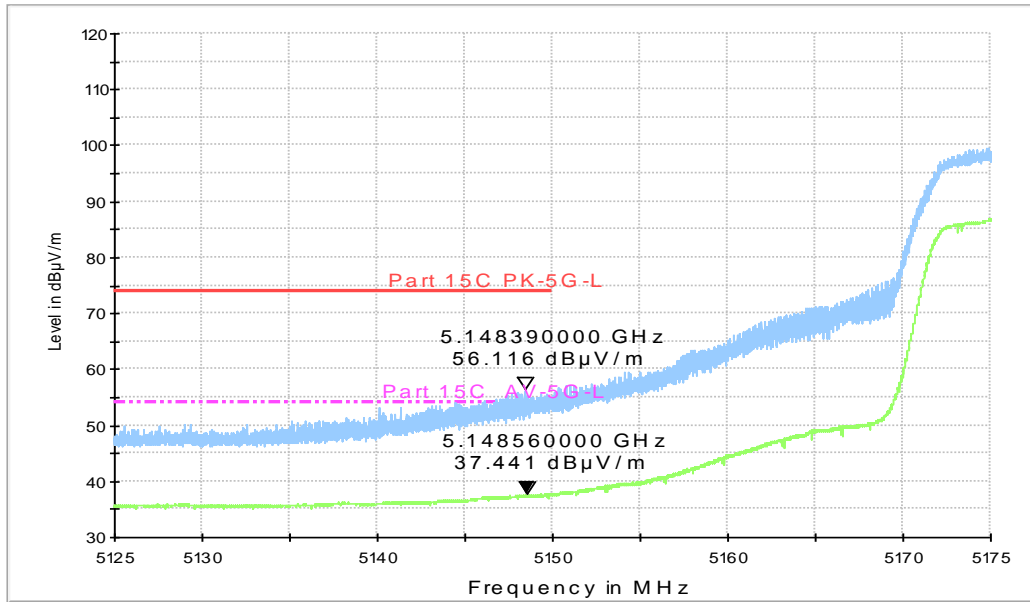
RE - Power-5.125GHz-5.175GHz
