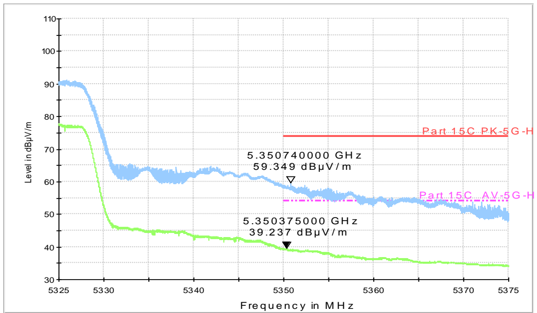
RE - Power-5.325GHz-5.375GHz
