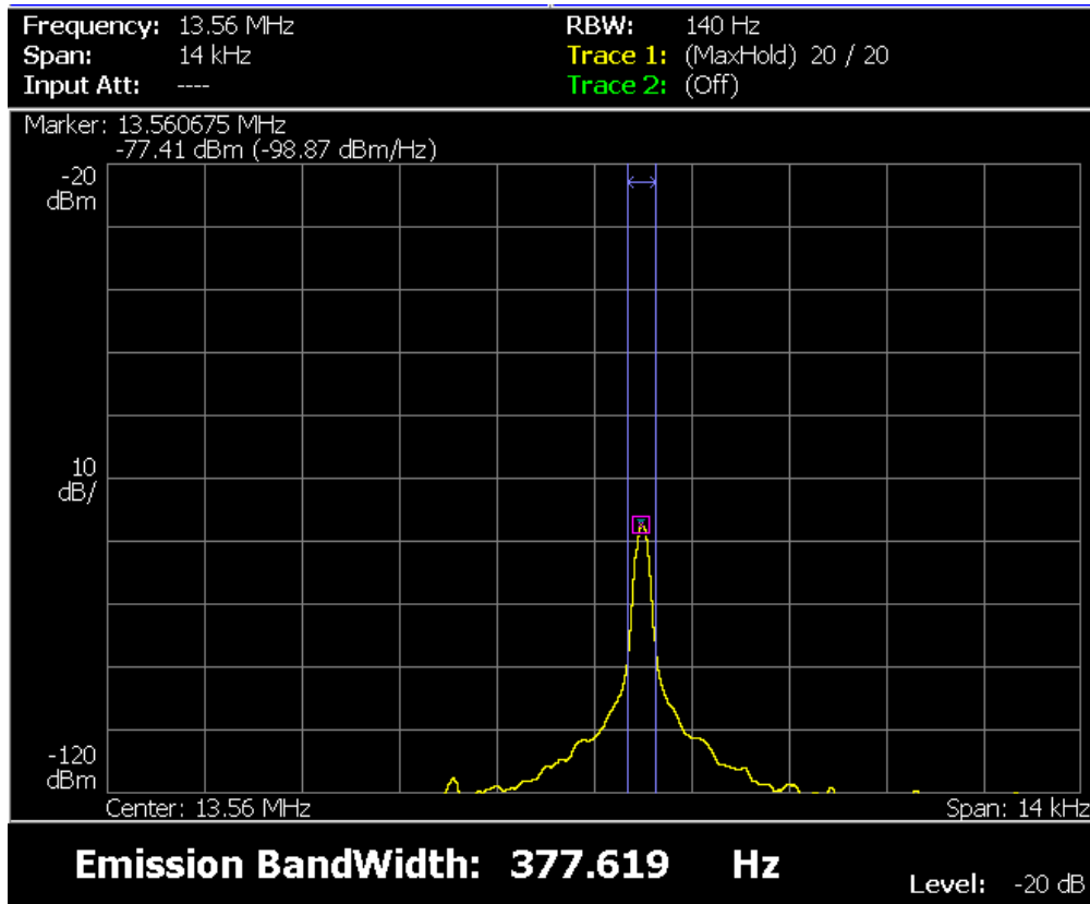
Figure A-4: Test result of EUT2 at test set. NFC02
