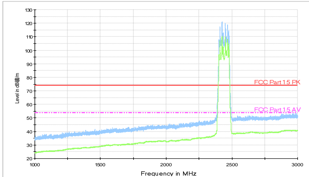
Fig.18. Transmitter Spurious Emission - Radiated: GFSK, 2402MHz, 1 GHz - 3GHz
