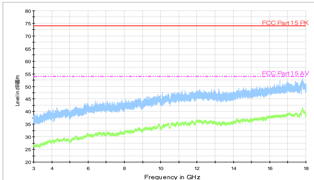
Fig.19. Transmitter Spurious Emission - Radiated: GFSK, 2402MHz, 3 GHz - 18 GHz
