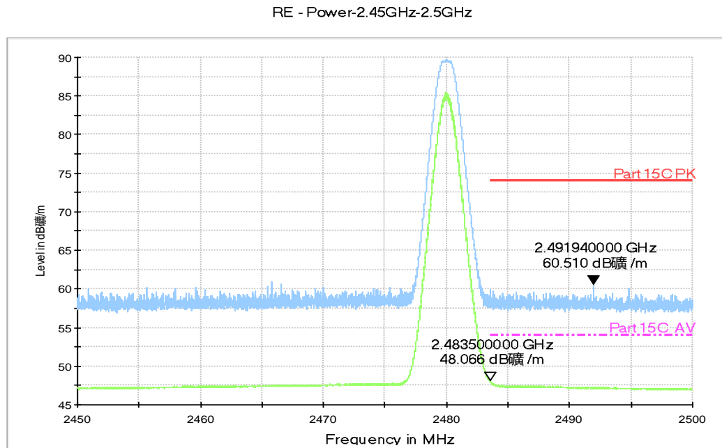
Fig.26. Transmitter Spurious Emission - Radiated (Power): GFSK high channel
