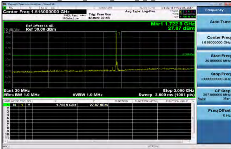
30MHz~3GHz_Band4_20MHz_QPSK_1_0_MidCH20175-1732.5
