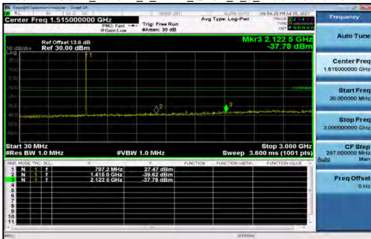
30MHz-3GHz_Band12_1_4MHz_QPSK_1_0_MidCH23095-707.5
