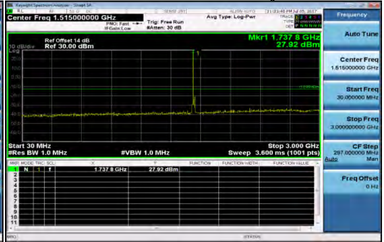
30MHz~3GHz_Band4_20MHz_QPSK_1_0_HighCH20300-1745
