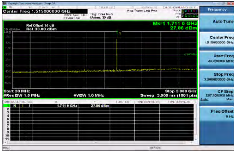
30MHz-3GHz_Band4_3MHz_QPSK_1_0_LowCH19965-1711.5
