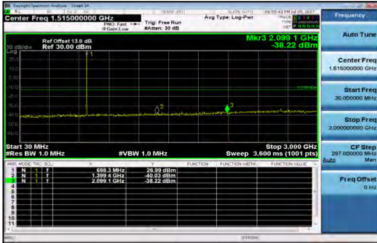
30MHz-3GHz_Band12_1_4MHz_QPSK_1_0_LowCH23017-699.7
