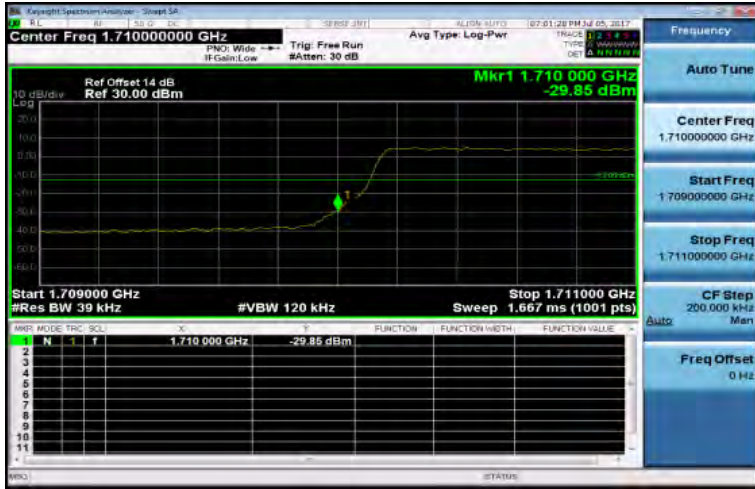
Band4_3MHz_QPSK_15_0_LowCH19965-1711.5
