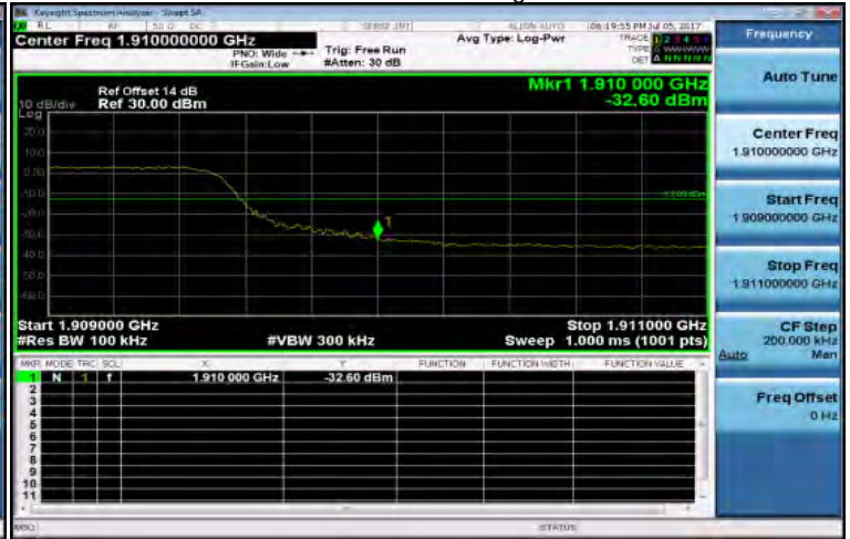
Band2_10MHz_QPSK_50_0_HighCH19150-1905
