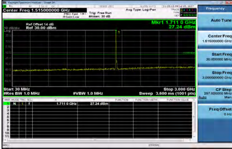
30MHz~3GHz_Band4_15MHz_QPSK_1_0_LowCH20025-1717.5
