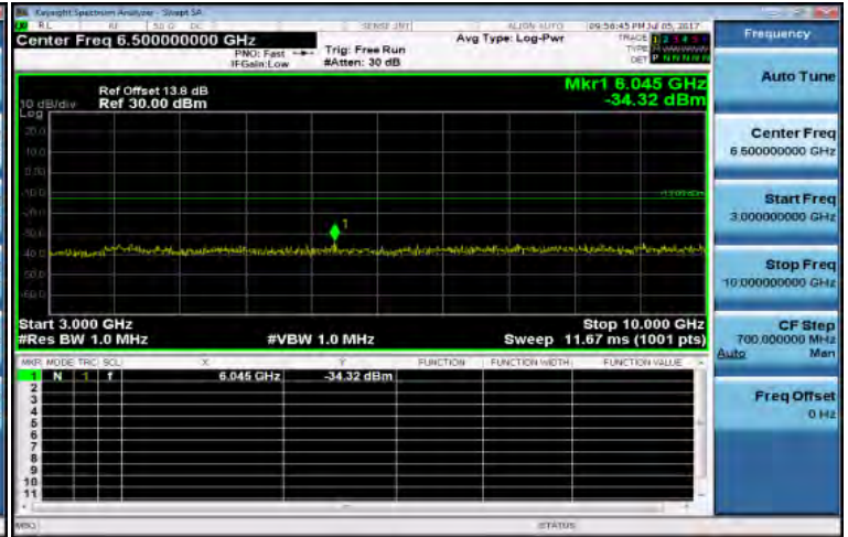
3GHz-10GHz_Band12_1_4MHz_QPSK_1_0_MidCH23095-707.5
