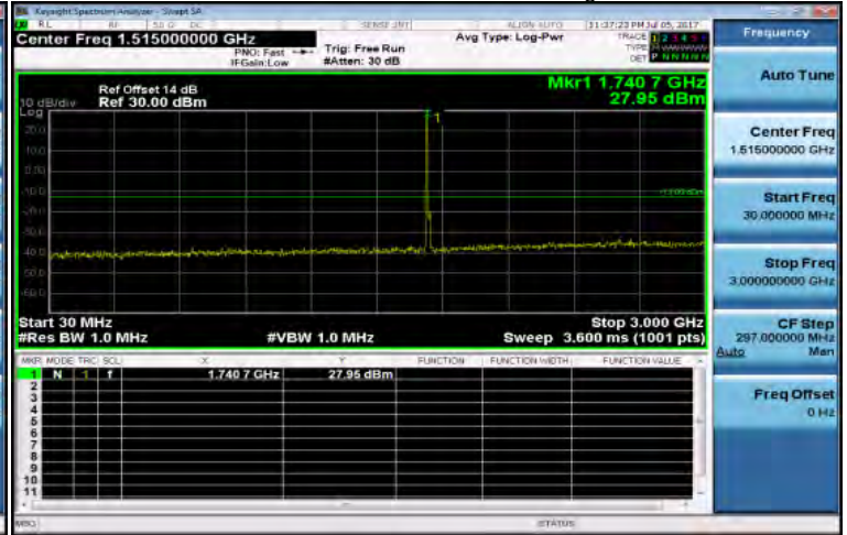
30MHz~3GHz_Band4_15MHz_QPSK_1_0_HighCH20325-1747.5
