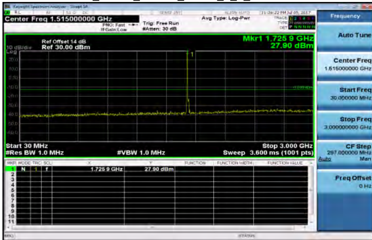
30MHz~3GHz_Band4_15MHz_QPSK_1_0_MidCH20175-1732.5
