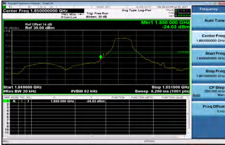
Band2_1_4MHz_QPSK_1_0_LowCH18607-1850.7
