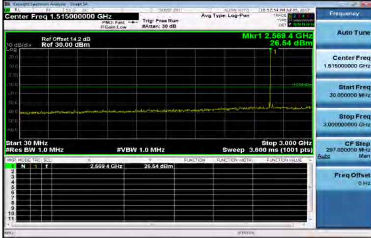
30MHz~3GHz_Band38_5MHz_QPSK_1_0_LowCH37775-2572.5
