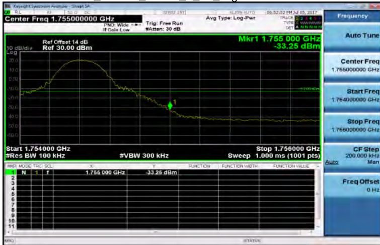
Band4_10MHz_QPSK_1_49_HighCH20350-1750
