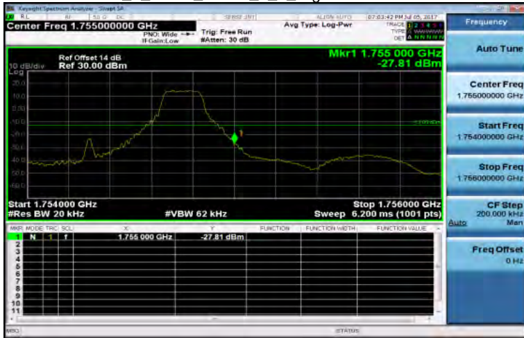
Band4_1_4MHz_QPSK_1_5_HighCH20393-1754.3
