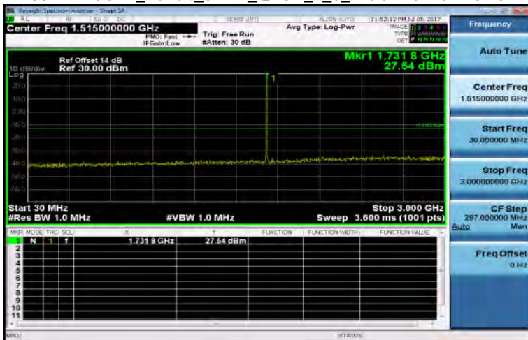
30MHz-3GHz_Band4_3MHz_QPSK_1_0_MidCH20175-1732.5
