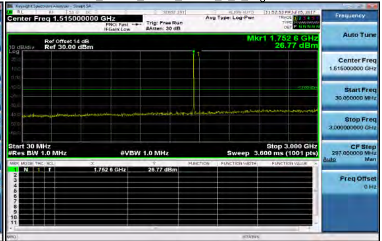
30MHz-3GHz_Band4_3MHz_QPSK_1_0_HighCH20385-1753.5
