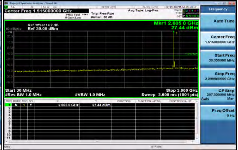
30MHz-3GHz_Band38_15MHz_QPSK_1_0_HighCH38175-2612.5
