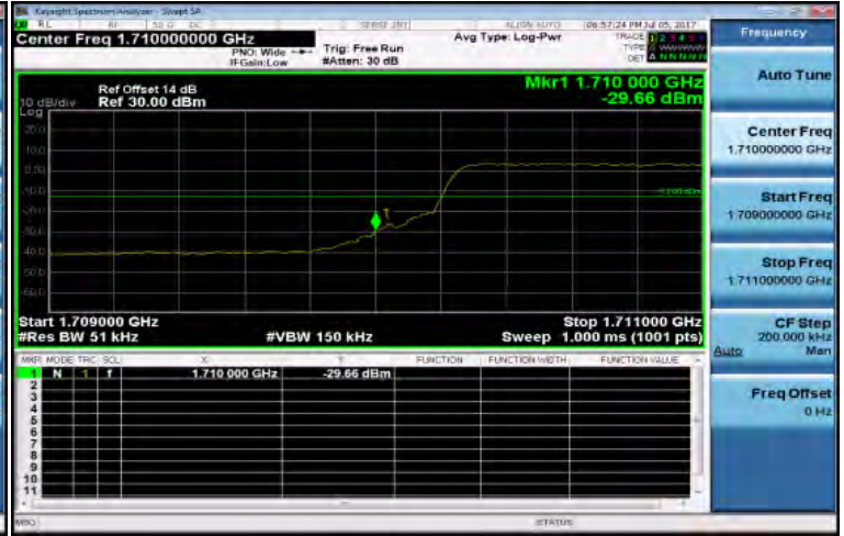
Band4_5MHz_QPSK_25_0_LowCH19975-1712.5
