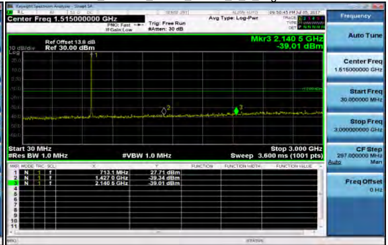
30MHz~3GHz_Band12_5MHz_QPSK_1_0_HighCH23155-713.5
