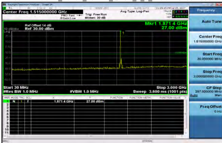
30MHz-3GHz_Band2_20MHz_QPSK_1_0_MidCH18900-1880
