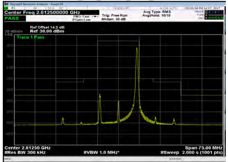
Band 38_15M_16QAM_HIGH_RB75,0
