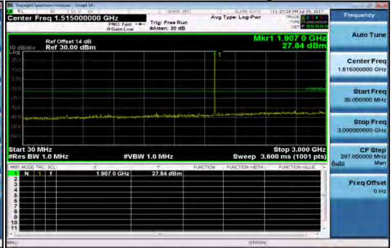
30MHz~3GHz_Band2_3MHz_QPSK_1_0_HighCH19185-1908.5
