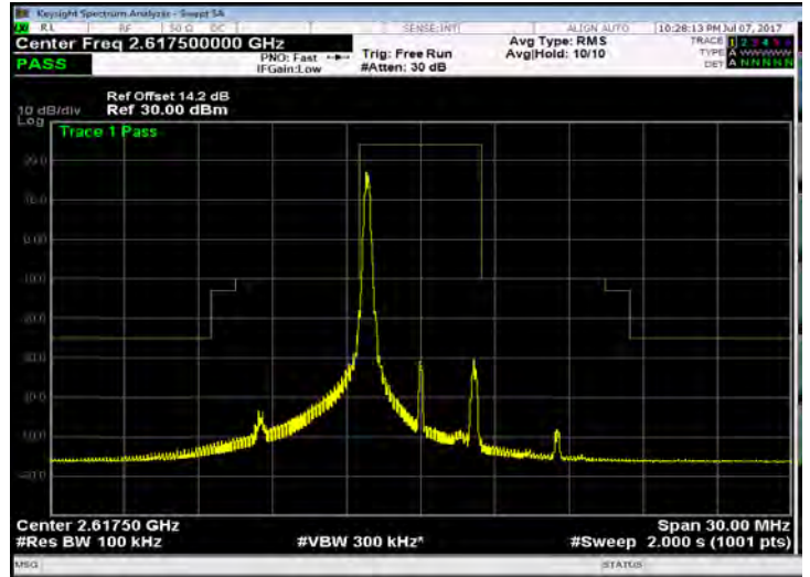
Band 38_5M_16QAM_HIGH_RB1,24
