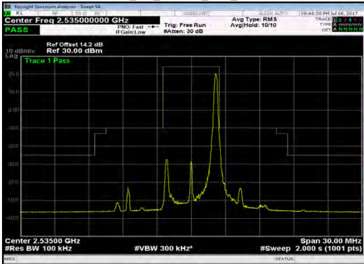
Band 7_5M_16QAM_MID_RB25,0
