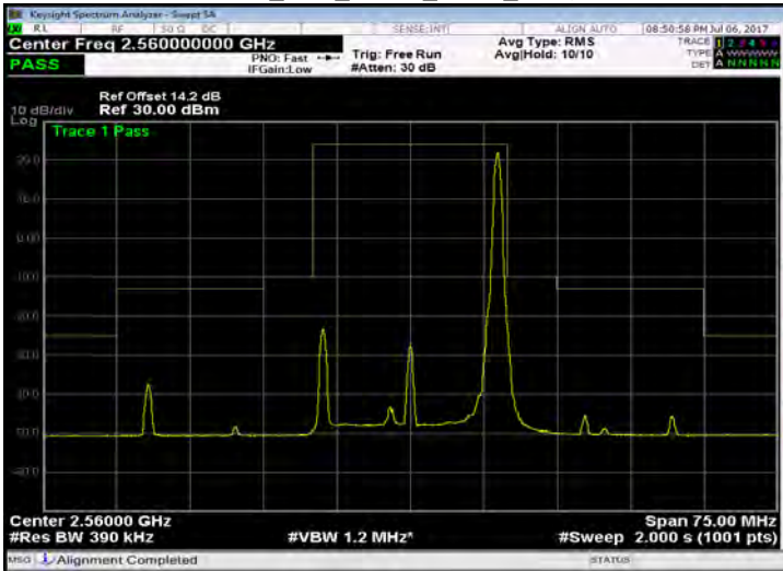
Band 7_20M_QPSK_HIGH_RB100,0
