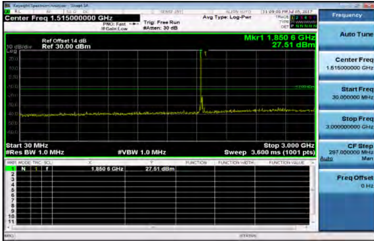
30MHz-3GHz_Band2_20MHz_QPSK_1_0_LowCH18700-1860
