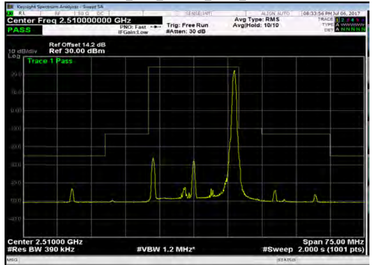
Band 7_20M_16QAM_LOW_RB100,0
