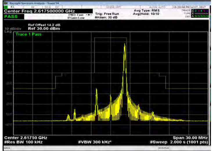
Band 38_5M_16QAM_HIGH_RB25,0
