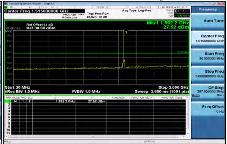
30MHz-3GHz_Band2_20MHz_QPSK_1_0_HighCH19100-1900
