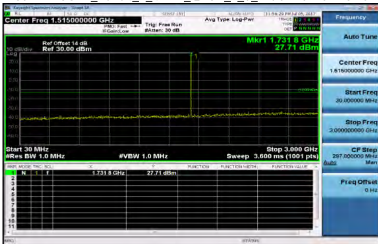
30MHz-3GHz_Band4_1_4MHz_QPSK_1_0_MidCH20175-1732.5
