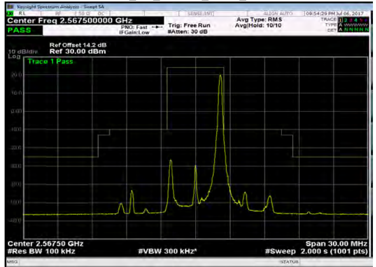
Band 7_5M_16QAM_HIGH_RB25,0
