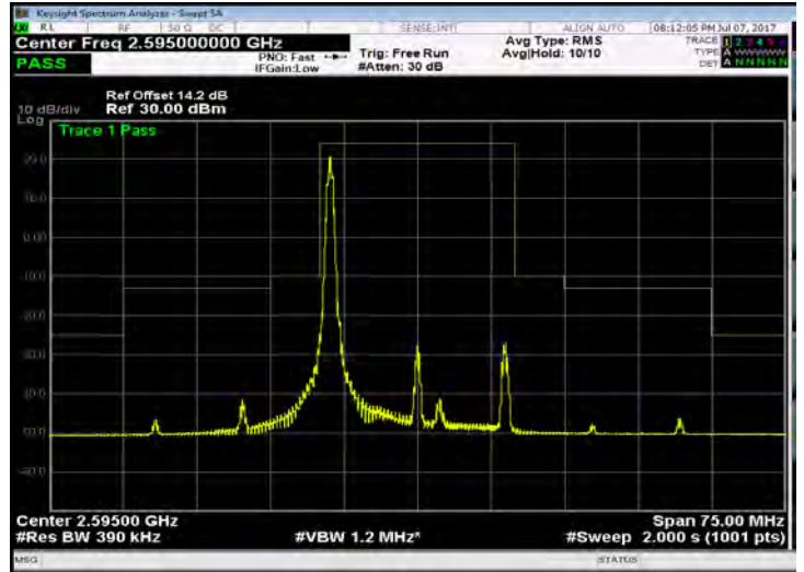
Band 38_20M_QPSK_MID_RB1,99
