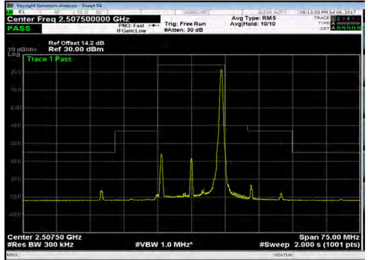
Band 7_15M_16QAM_LOW_RB75,0
