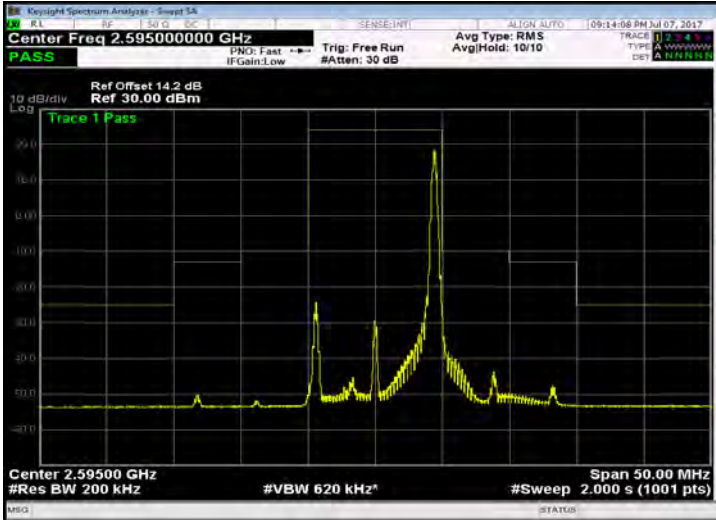
Band 38_10M_16QAM_MID_RB50,0
