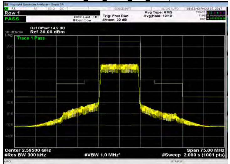
Band 38_15M_QPSK_MID_RB75,0
