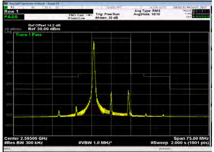
Band 38_15M_QPSK_MID_RB1,74
