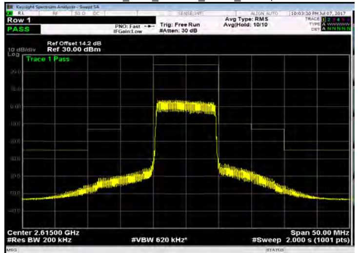
Band 38_10M_16QAM_HIGH_RB50,0
