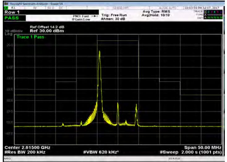
Band 38_10M_16QAM_HIGH_RB1,49
