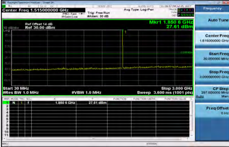
30MHz-3GHz_Band2_1_4MHz_QPSK_1_0_LowCH18607-1850.7
