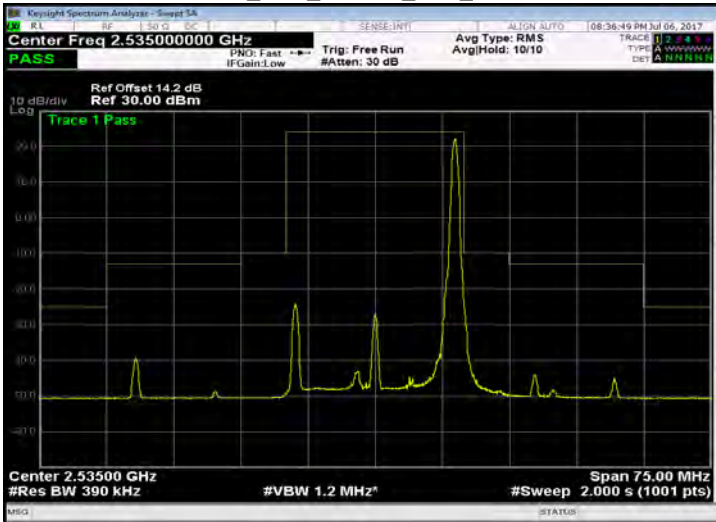
Band 7_20M_16QAM_MID_RB100,0
