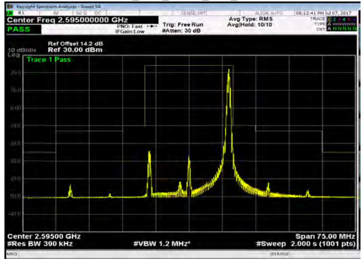
Band 38_20M_QPSK_MID_RB100,0
