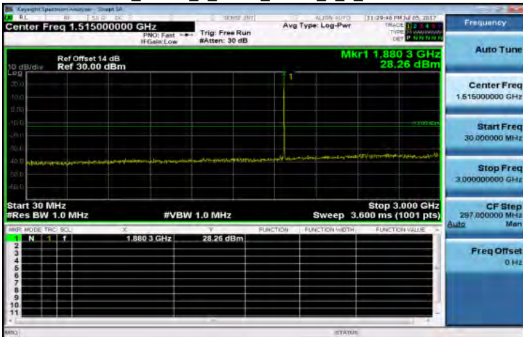
30MHz-3GHz_Band2_1_4MHz_QPSK_1_0_MidCH18900-1880
