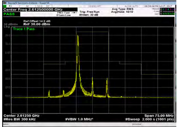
Band 38_15M_16QAM_HIGH_RB1,74
