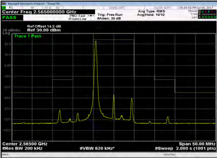
Band 7_10M_QPSK_HIGH_RB1,49
