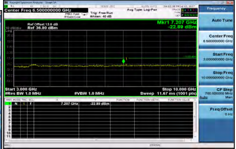
3GHz-10GHz_GSM_850MHz_MidCH190-836.6
