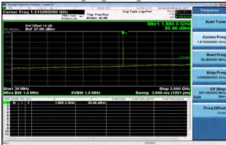
30MHz~3GHz_GSM_1900MHz_MidCH661-1880
