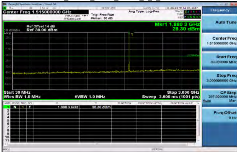
30MHz~3GHz_Band2_3MHz_QPSK_1_0_MidCH18900-1880
