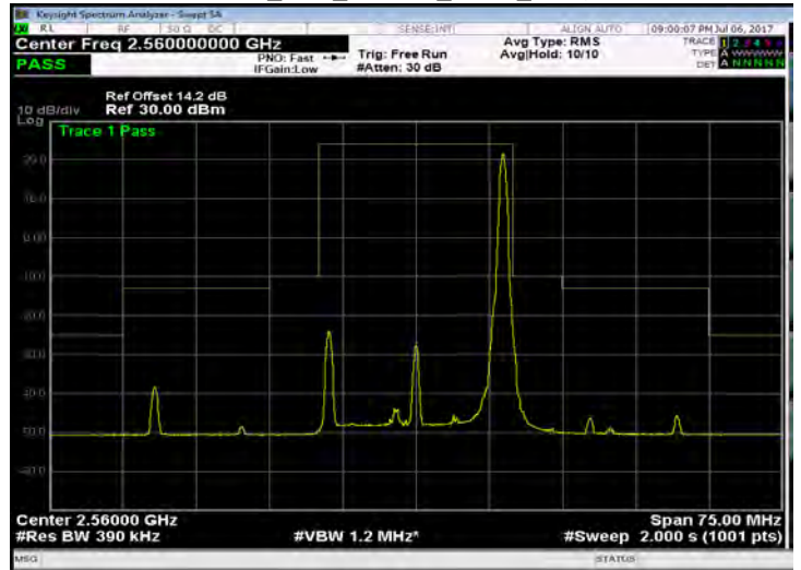
Band 7_20M_16QAM_HIGH_RB100,0
