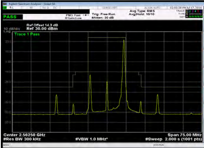
Band 7_15M_QPSK_HIGH_RB75,0
