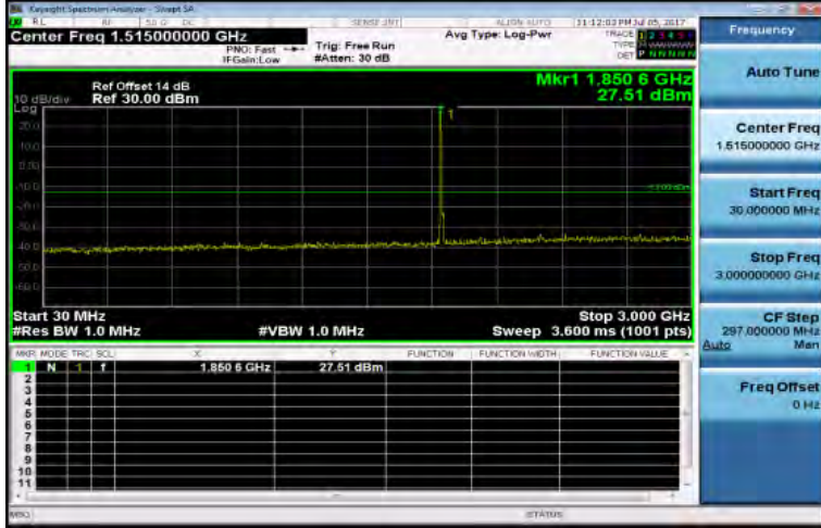
30MHz~3GHz_Band2_15MHz_QPSK_1_0_LowCH18675-1857.5
