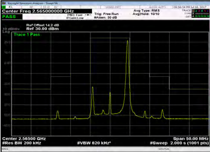
Band 7_10M_QPSK_HIGH_RB50,0
