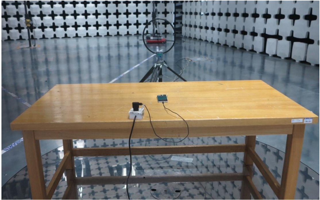
Field Strength Measurements (Below 30MHz)
