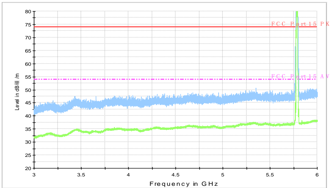
RE - 3GHz-6GHz
