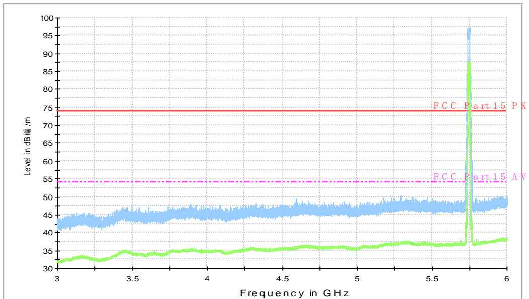
RE - 3GHz-6GHz
