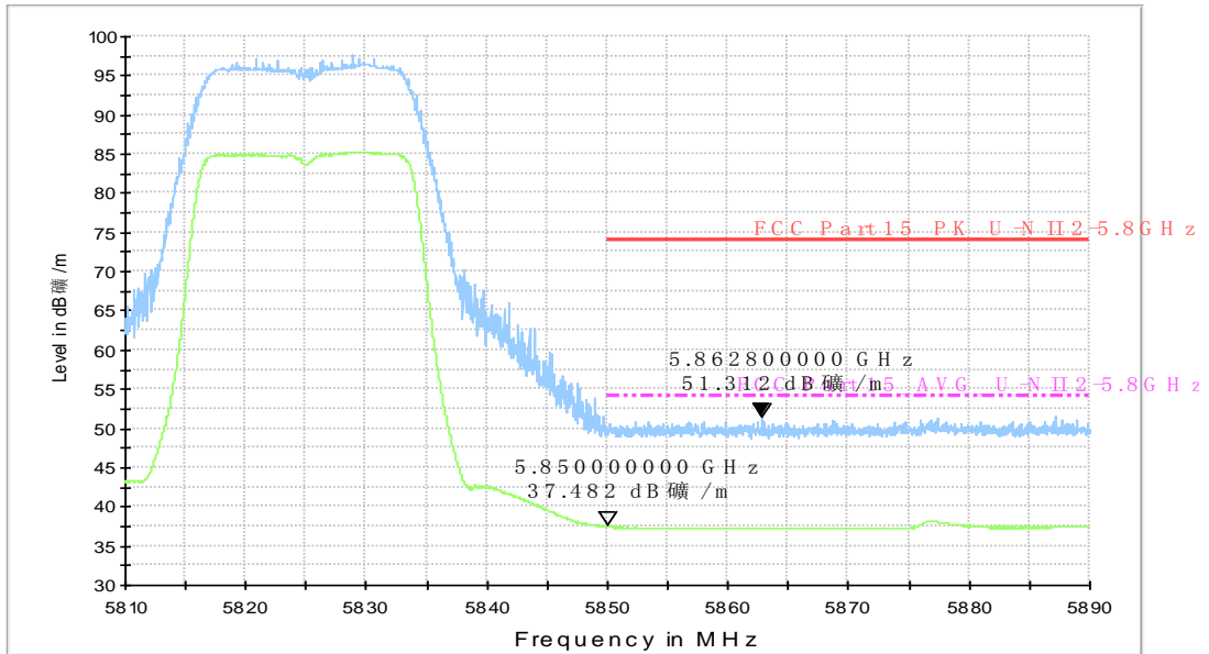
RE - Power-5.810GHz-5.890GHz
