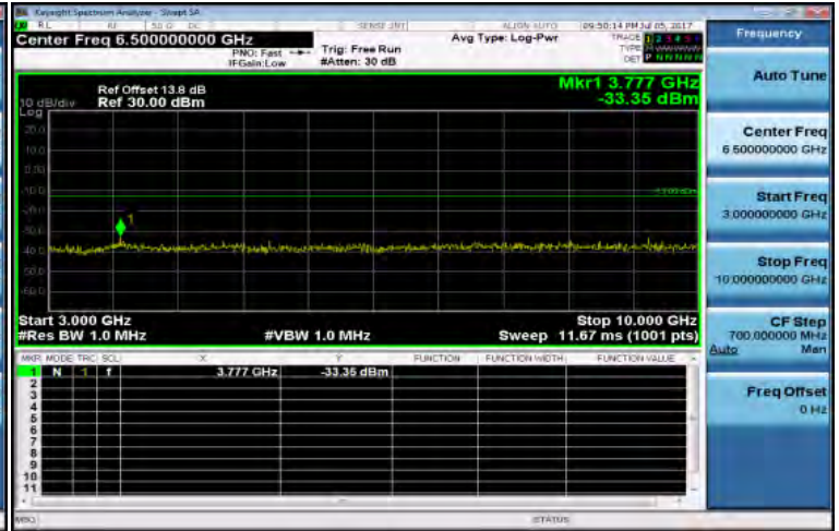
3GHz~10GHz_Band12_5MHz_QPSK_1_0_MidCH23095-707.5
