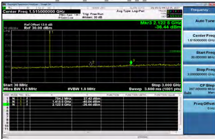
30MHz~3GHz_Band12_5MHz_QPSK_1_0_MidCH23095-707.5
