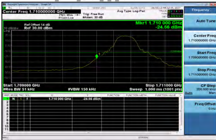
Band4_5MHz_QPSK_1_0_LowCH19975-1712.5
