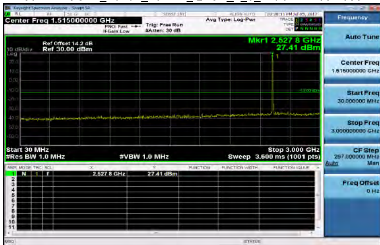
30MHz~3GHz_Band7_15MHz_QPSK_1_0_MidCH21100-2535
