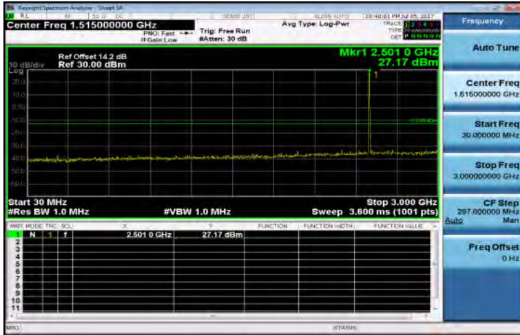
30MHz-3GHz_Band7_10MHz_QPSK_1_0_LowCH20800-2505
