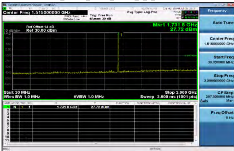
30MHz-3GHz_Band4_5MHz_QPSK_1_0_MidCH20175-1732.5
