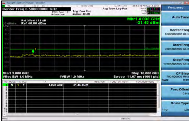
3GHz~10GHz_Band5_3MHz_QPSK_1_0_LowCH20415-825.5
