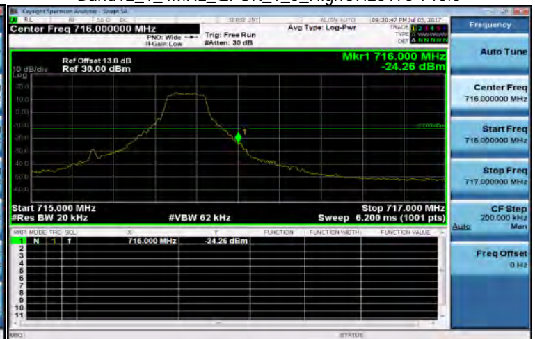
Band12_1_4MHz_QPSK_1_5_HighCH23173-715.3
