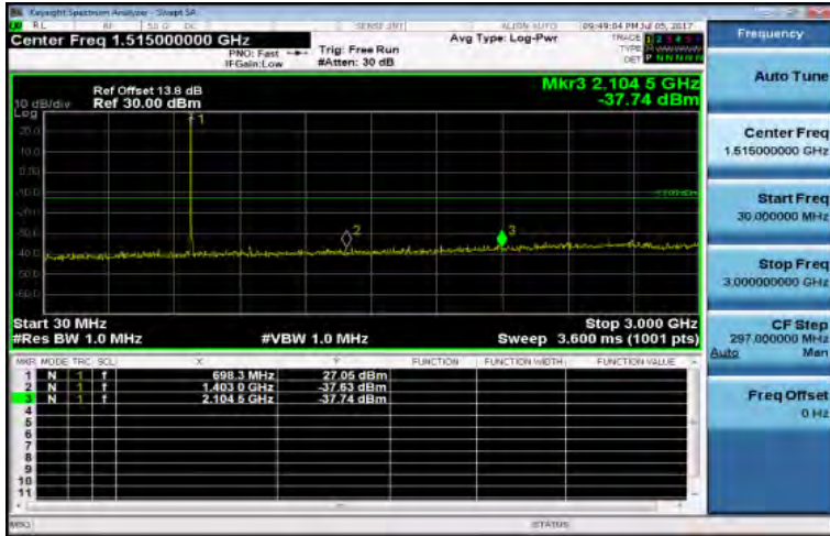
30MHz~3GHz_Band12_5MHz_QPSK_1_0_LowCH23035-701.5
