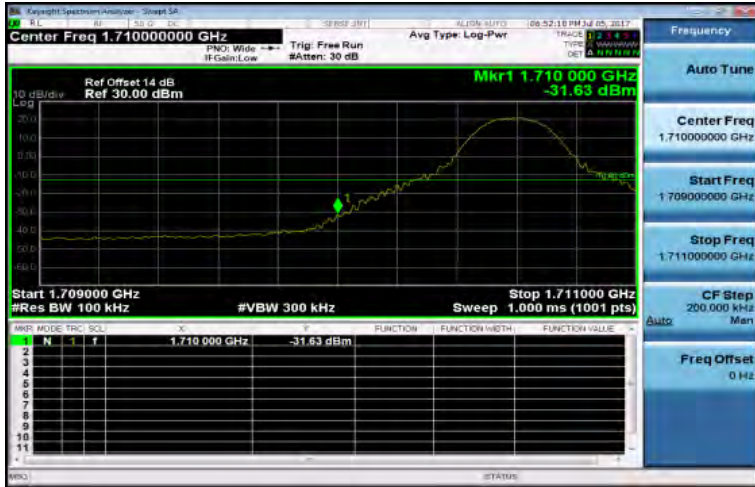
Band4_10MHz_QPSK_1_0_LowCH2000-1715
