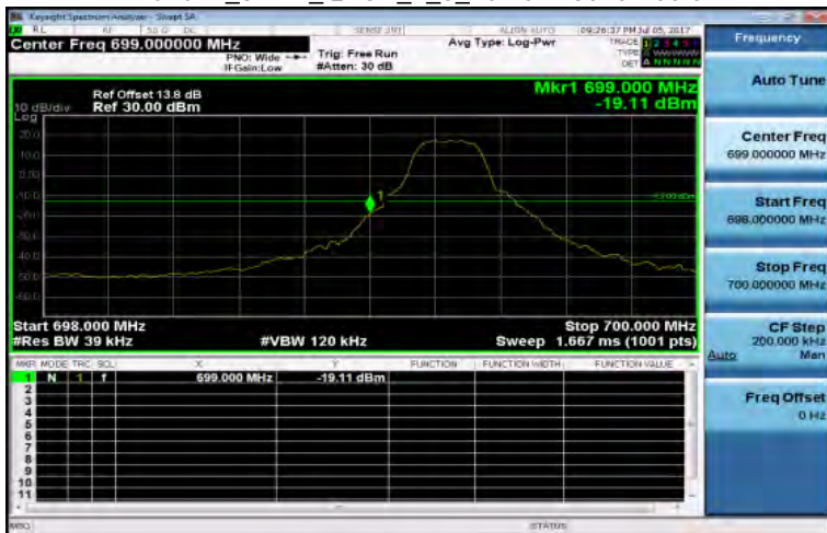
Band12_3MHz_QPSK_1_0_LowCH23025-700.5
