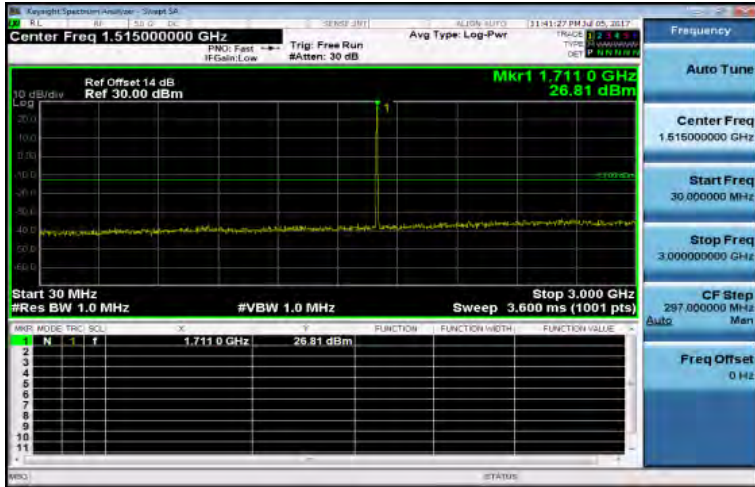
30MHz-3GHz_Band4_5MHz_QPSK_1_0_LowCH19975-1712.5
