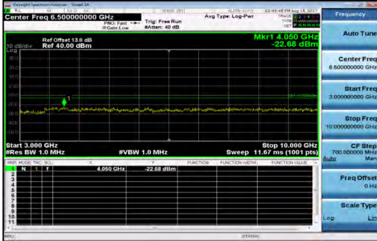
3GHz-10GHz_Band5_10MHz_QPSK_1_0_LowCH20450-829
