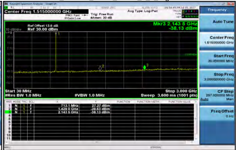
30MHz-3GHz_Band12_3MHz_QPSK_1_0_HighCH23165-714.5
