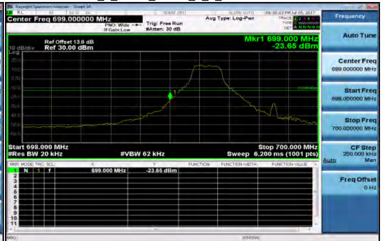
Band12_1_4MHz_QPSK_1_0_LowCH23017-699.7
