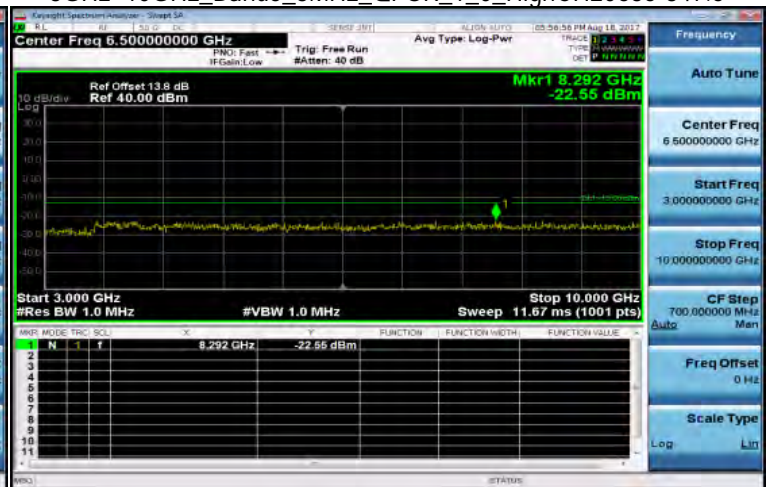
3GHz~10GHz_Band5_3MHz_QPSK_1_0_HighCH20635-847.5
