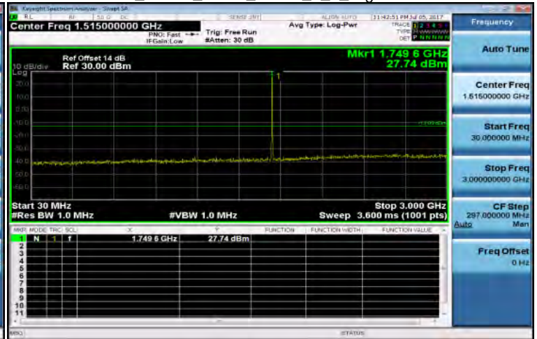
30MHz-3GHz_Band4_5MHz_QPSK_1_0_HighCH20375-1752.5
