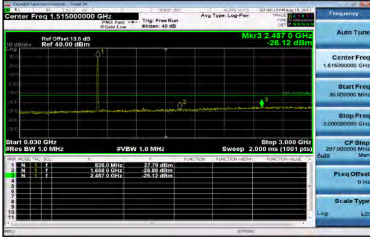
30MHz-3GHz_Band5_10MHz_QPSK_1_0_LowCH20450-829
