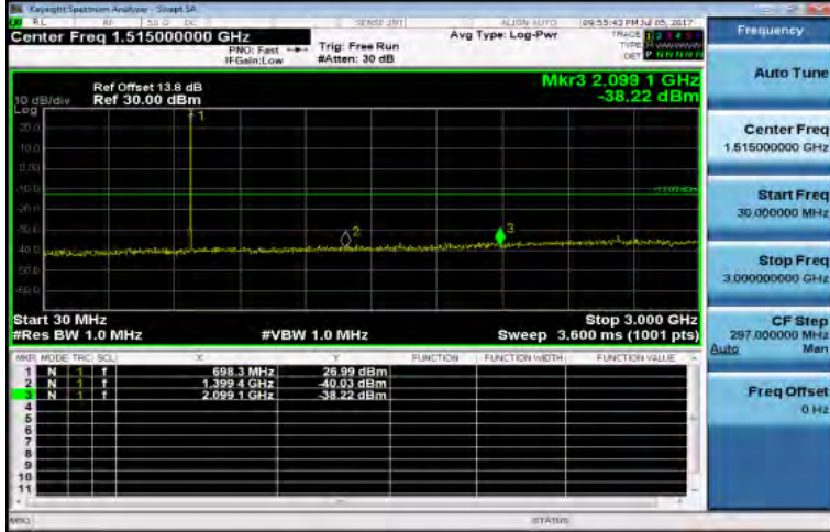
30MHz-3GHz_Band12_1_4MHz_QPSK_1_0_LowCH23017-699.7
