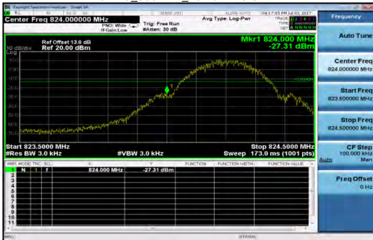
GRS_850MHz_LowCH128-824.2
