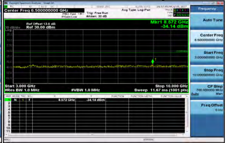
3GHz-10GHz_Band12_1_4MHz_QPSK_1_0_HighCH23173-715.3
