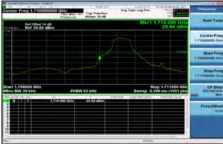
Band4_1_4MHz_QPSK_1_0_LowCH19957-1710.7
