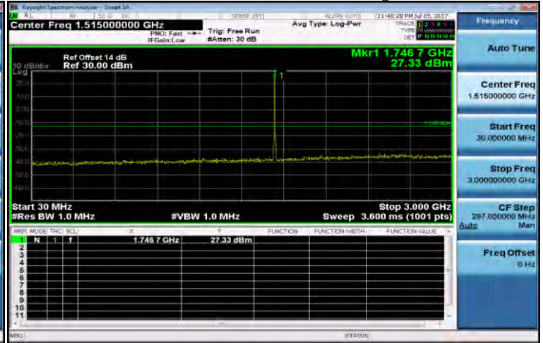
30MHz~3GHz_Band4_10MHz_QPSK_1_0_HighCH20350-1750
