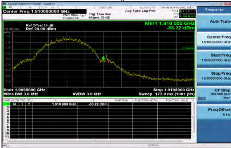
GSM_1900MHz_HighCH810-1909.8
