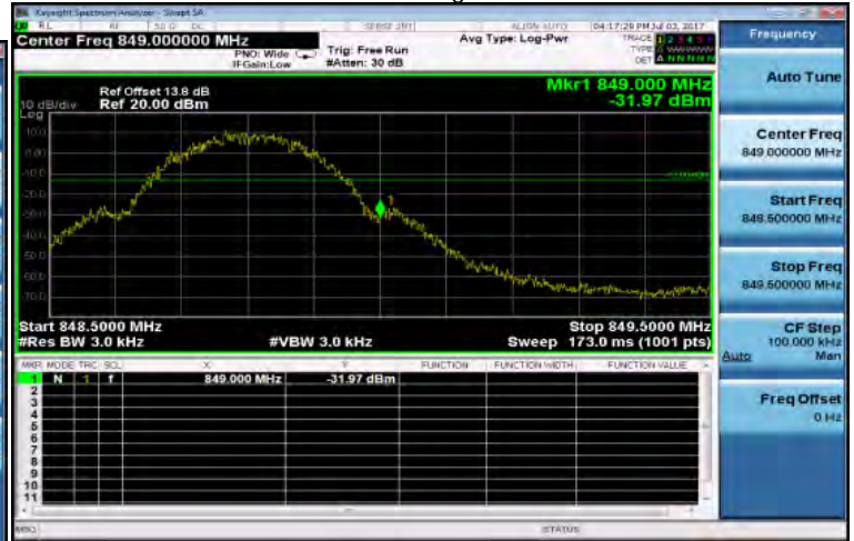
GRS_850MHz_HighCH251-848.8
