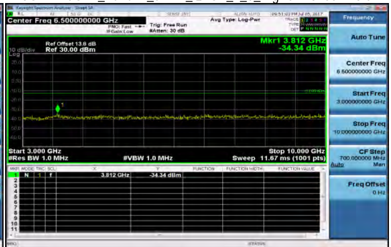
3GHz~10GHz_Band12_5MHz_QPSK_1_0_HighCH23155-713.5
