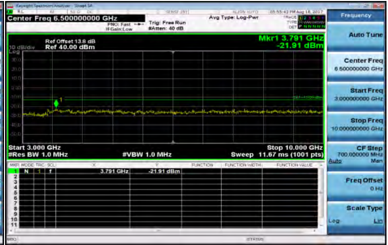
3GHz~10GHz_Band5_3MHz_QPSK_1_0_MidCH20525-836.5
