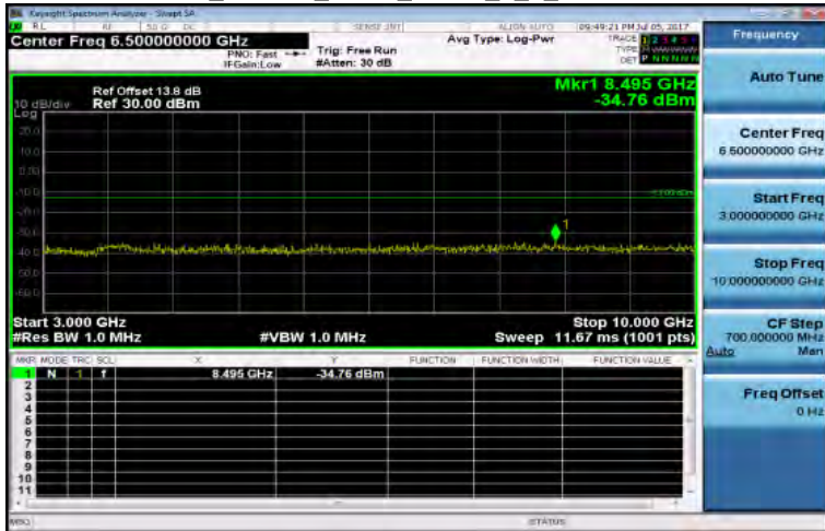
3GHz~10GHz_Band12_5MHz_QPSK_1_0_LowCH23035-701.5
