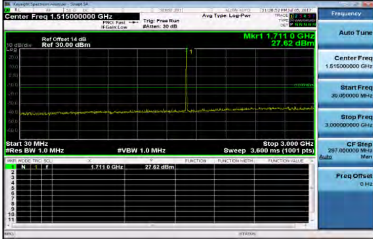
30MHz~3GHz_Band4_10MHz_QPSK_1_0_LowCH20000-1715
