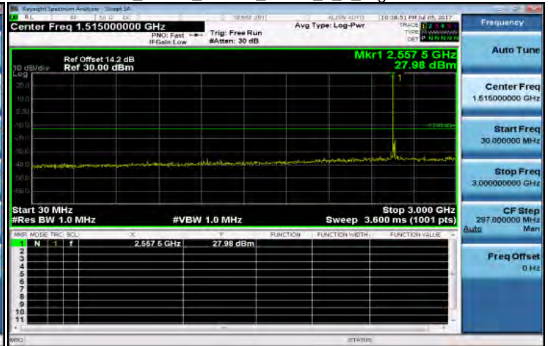
30MHz~3GHz_Band7_15MHz_QPSK_1_0_HighCH21375-2562.5
