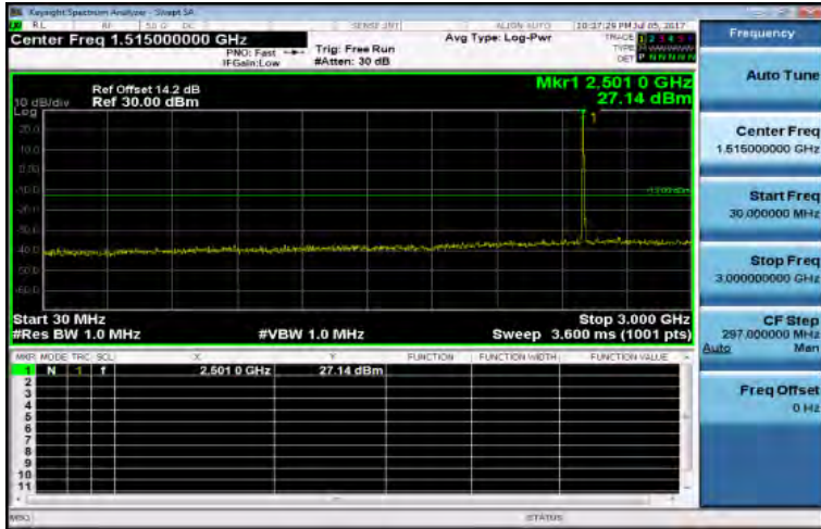
30MHz~3GHz_Band7_15MHz_QPSK_1_0_LowCH20825-2507.5
