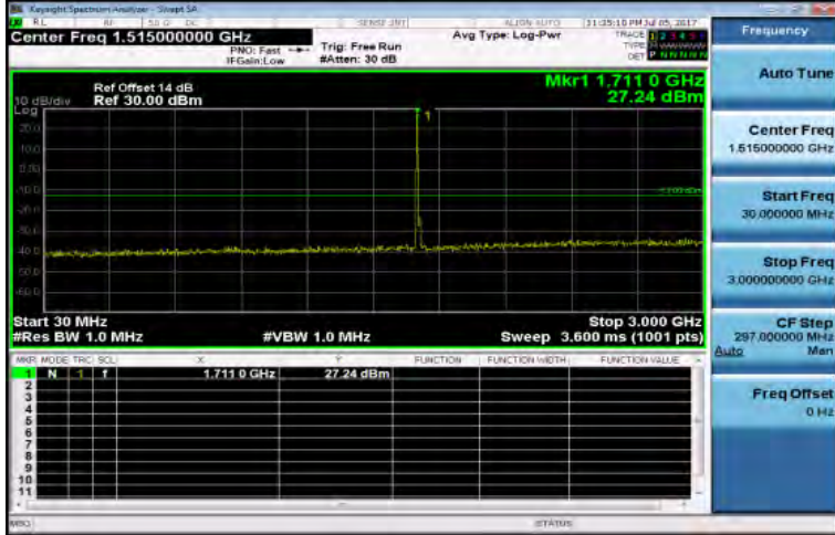
30MHz~3GHz_Band4_15MHz_QPSK_1_0_LowCH20025-1717.5
