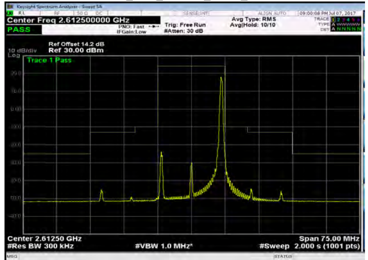
Band 38_15M_16QAM_HIGH_RB75,0
