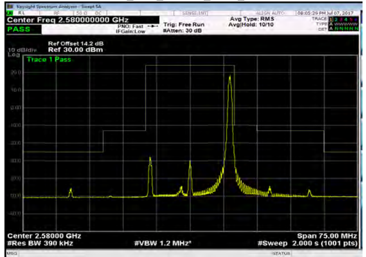
Band 38_20M_16QAM_LOW_RB100,0
