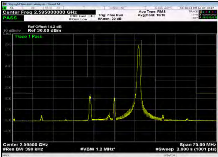
Band 38_20M_16QAM_MID_RB100,0
