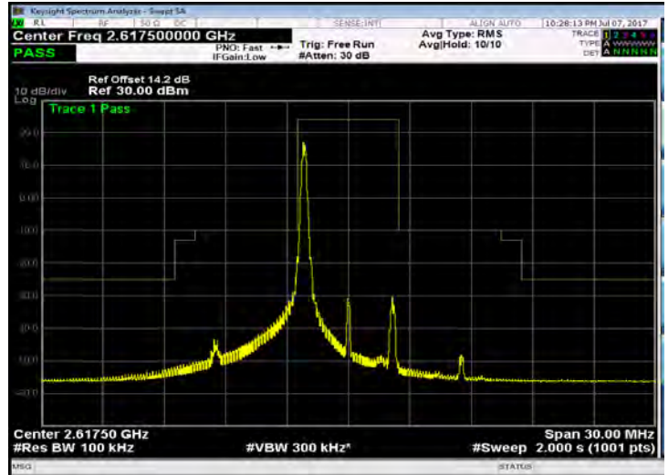
Band 38_5M_16QAM_HIGH_RB1,24
