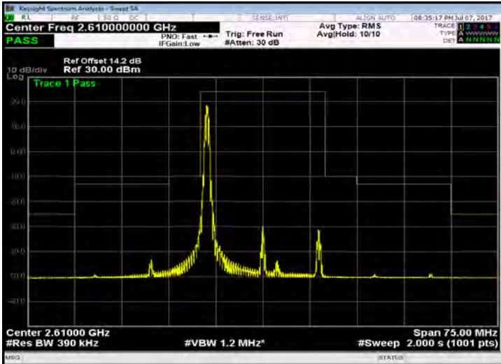
Band 38_20M_QPSK_HIGH_RB1,99
