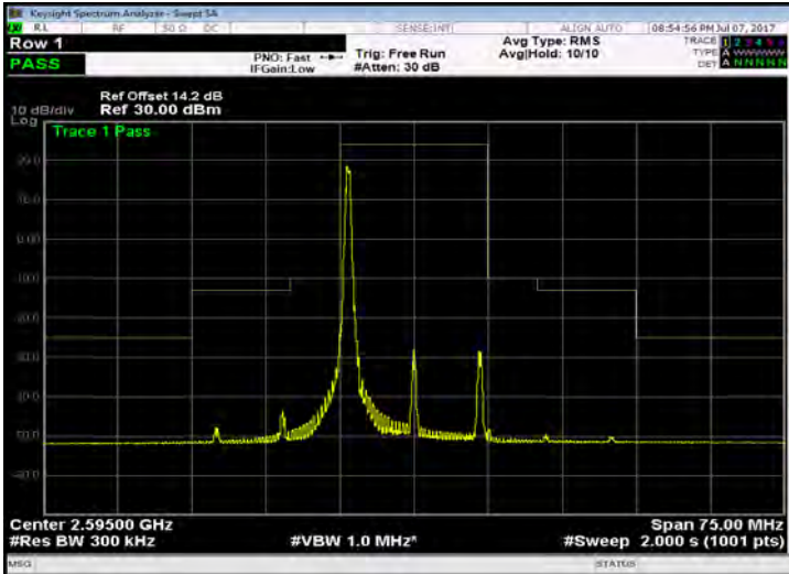
Band 38_15M_16QAM_MID_RB1,74
