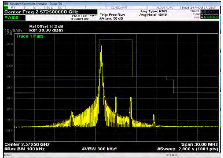
Band 38_5M_16QAM_LOW_RB1,24
