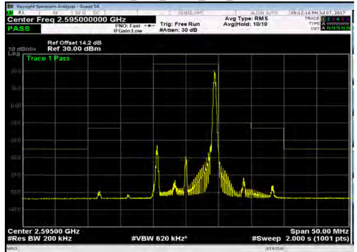
Band 38_10M_QPSK_MID_RB50,0
