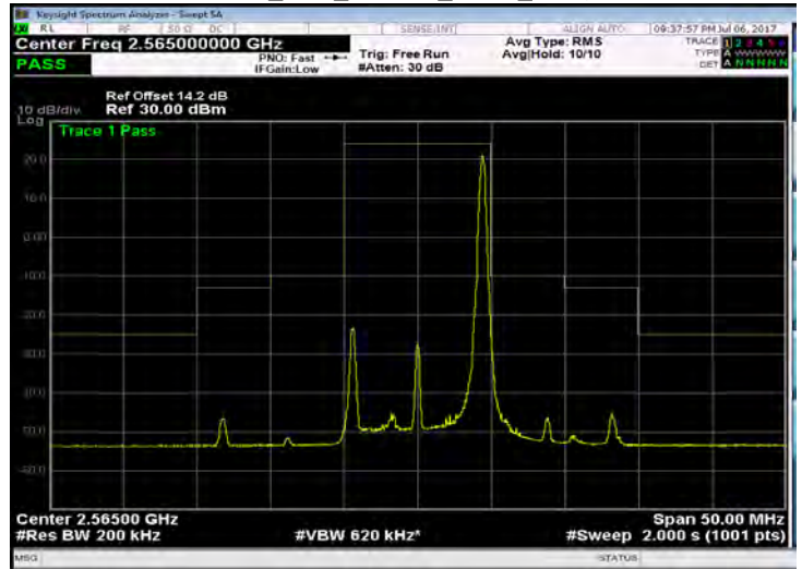
Band 7_10M_16QAM_HIGH_RB50,0
