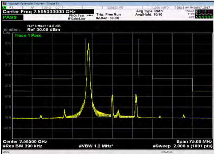
Band 38_20M_16QAM_MID_RB1,99
