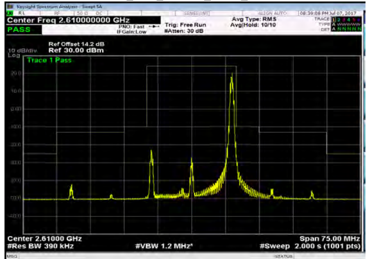
Band 38_20M_16QAM_HIGH_RB100,0
