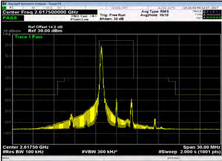
Band 38_5M_QPSK_HIGH_RB1,24
