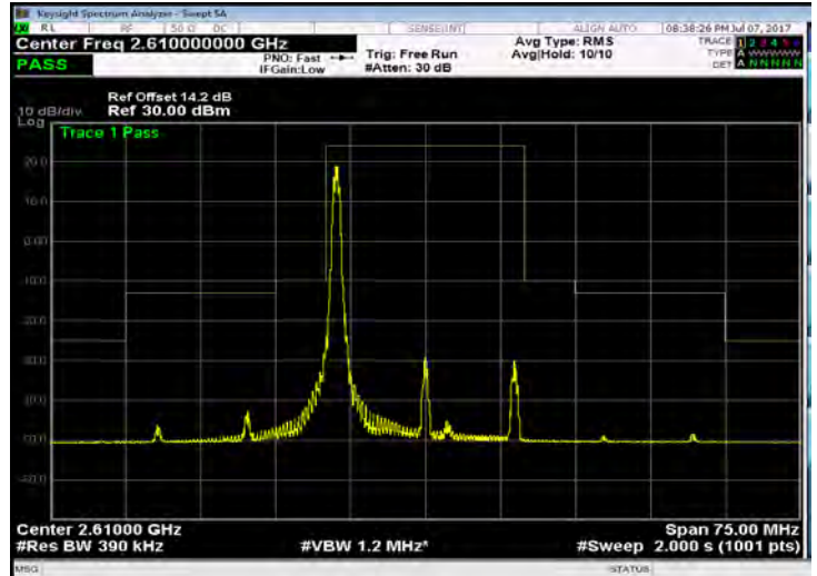
Band 38_20M_16QAM_HIGH_RB1,99
