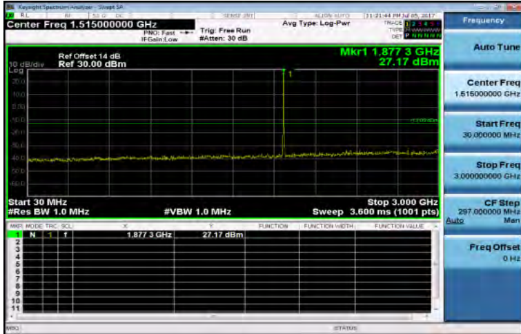
30MHz~3GHz_Band2_5MHz_QPSK_1_0_MidCH18900-1880
