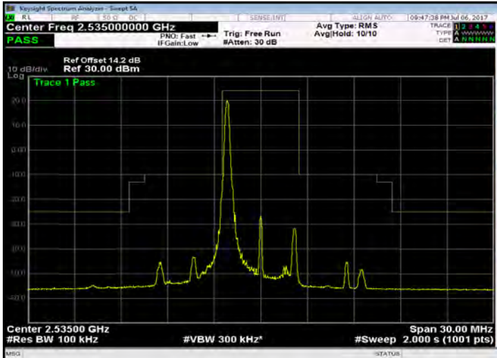
Band 7_5M_16QAM_MID_RB1,24
