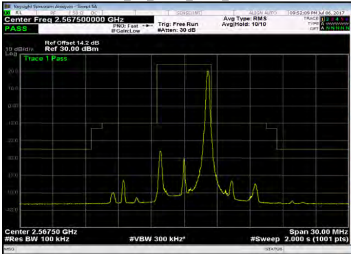
Band 7_5M_QPSK_HIGH_RB25,0
