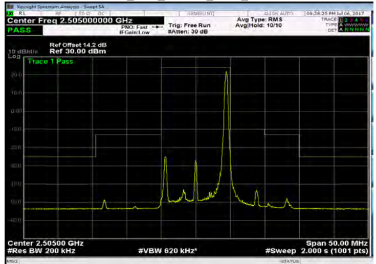
Band 7_10M_16QAM_LOW_RB50,0
