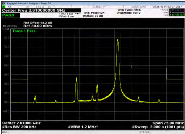
Band 38_20M_QPSK_HIGH_RB100,0
