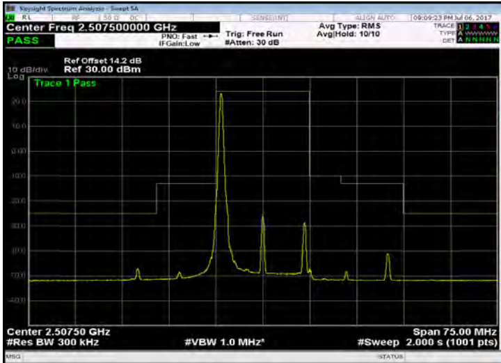
Band 7_15M_QPSK_LOW_RB1,74
