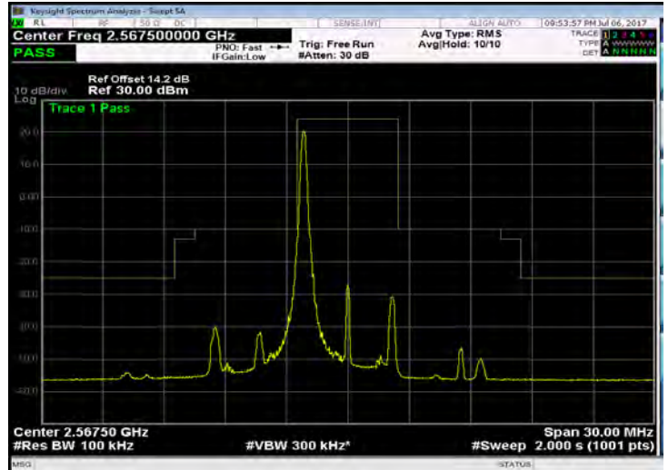
Band 7_5M_16QAM_HIGH_RB1,24
