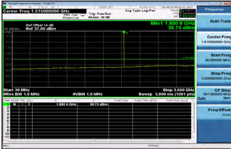
30MHz~3GHz_GSM_1900MHz_LowCH512-1850.2
