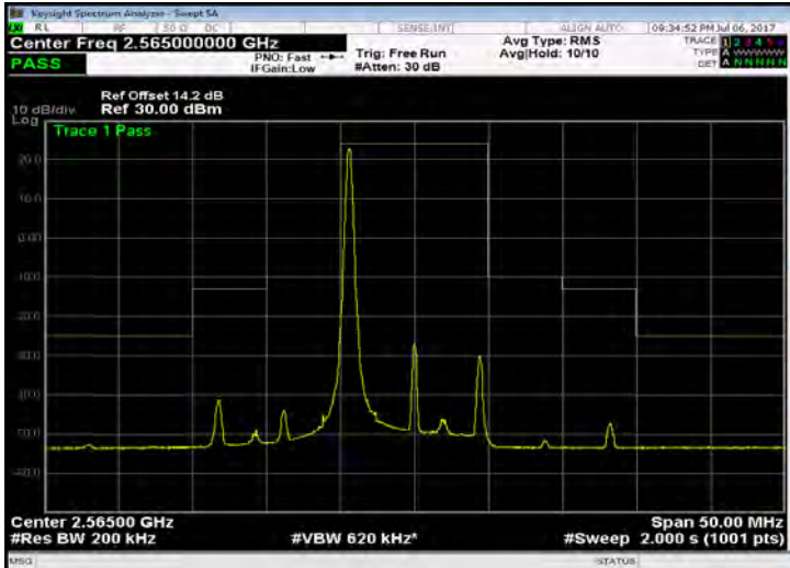
Band 7_10M_QPSK_HIGH_RB1,49
