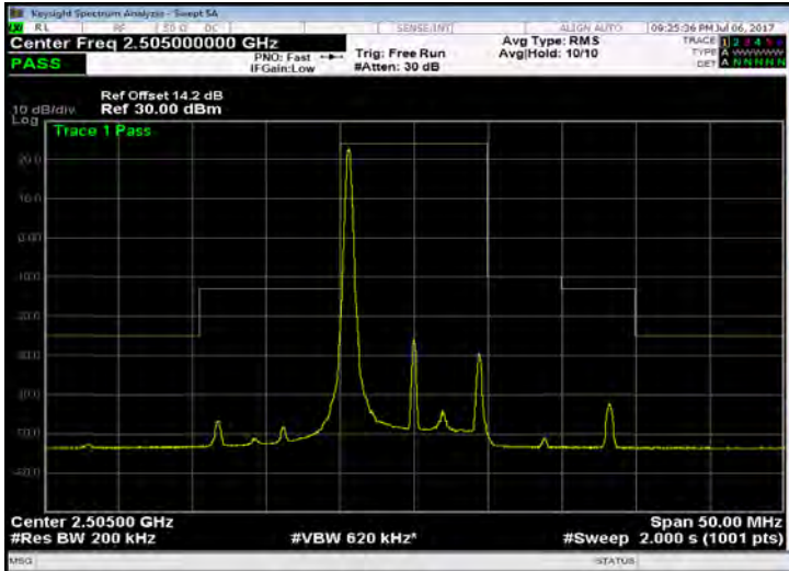
Band 7_10M_QPSK_LOW_RB1,49
