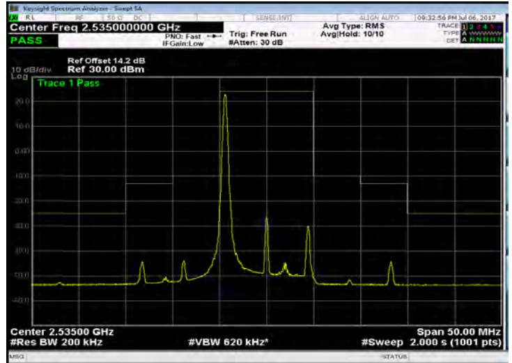
Band 7_10M_QPSK_MID_RB1,49
