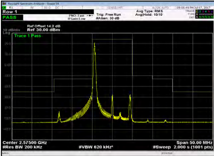
Band 38_10M_QPSK_LOW_RB1,49
