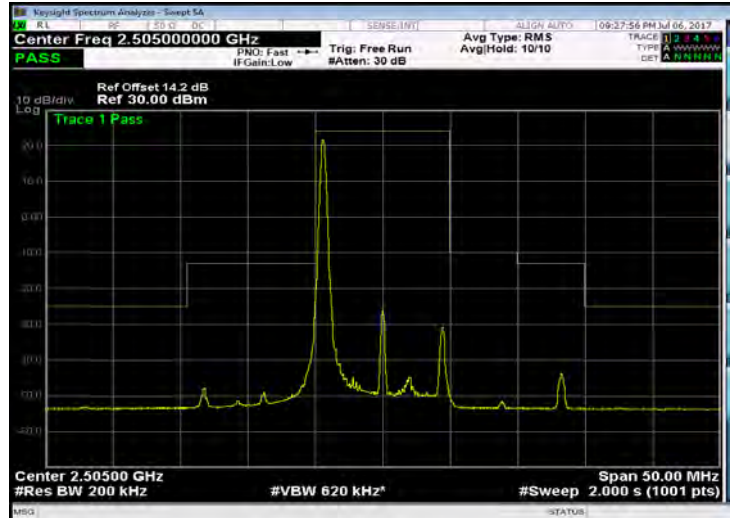
Band 7_10M_16QAM_LOW_RB1,49
