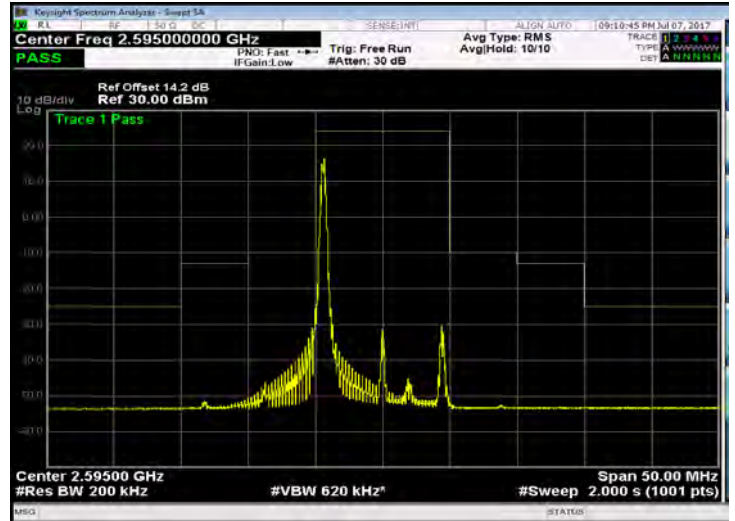
Band 38_10M_QPSK_MID_RB1,49
