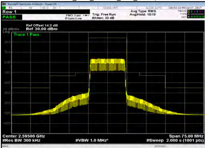
Band 38_15M_16QAM_MID_RB75,0
