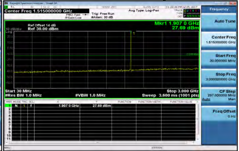
30MHz~3GHz_Band2_5MHz_QPSK_1_0_HighCH19175-1907.5
