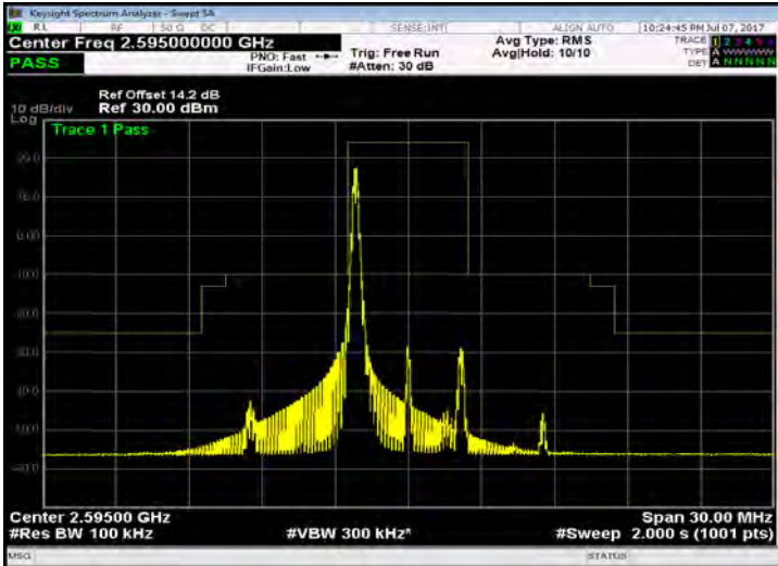
Band 38_5M_16QAM_MID_RB1,24
