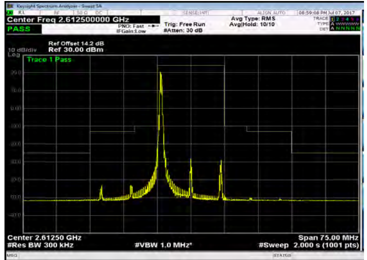
Band 38_15M_16QAM_HIGH_RB1,74
