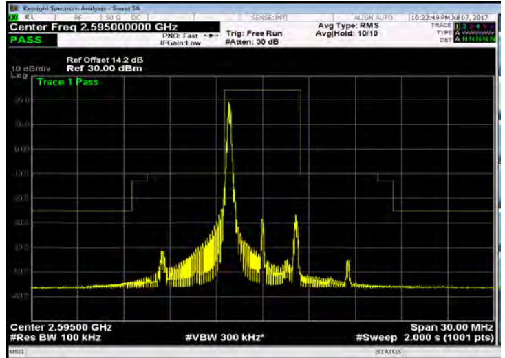
Band 38_5M_QPSK_MID_RB1,24
