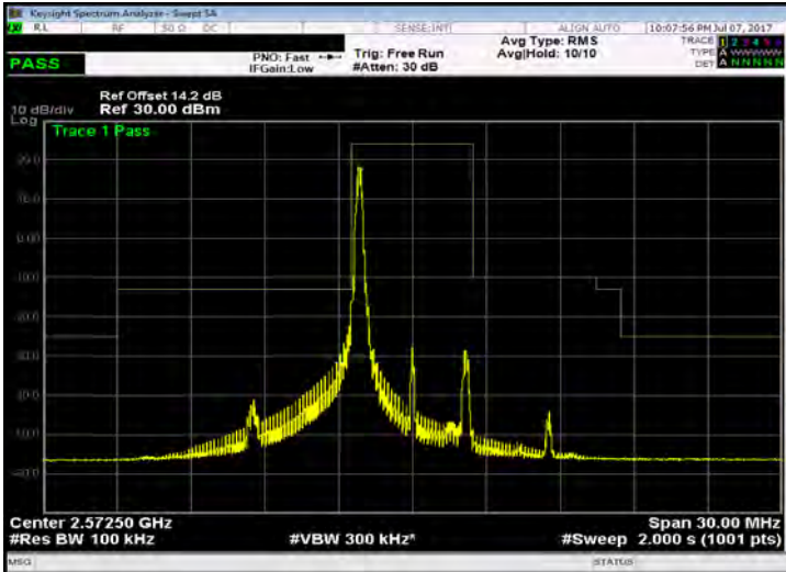
Band 38_5M_QPSK_LOW_RB1,24
