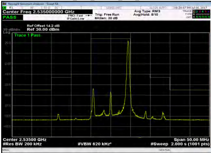
Band 7_10M_16QAM_MID_RB50,0
