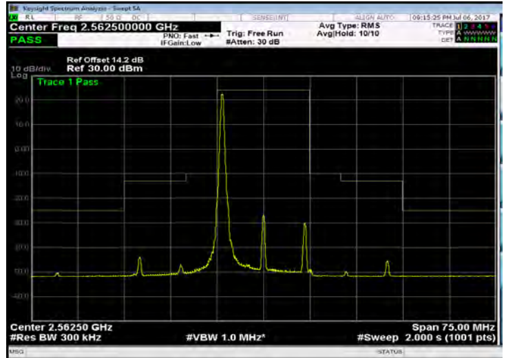
Band 7_15M_16QAM_HIGH_RB1,74
