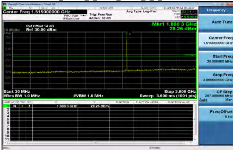
30MHz-3GHz_Band2_1_4MHz_QPSK_1_0_MidCH18900-1880
