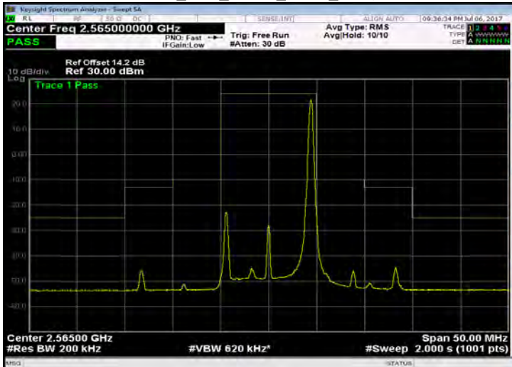
Band 7_10M_QPSK_HIGH_RB50,0
