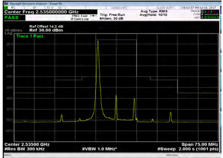
Band 7_15M_QPSK_MID_RB1,74
