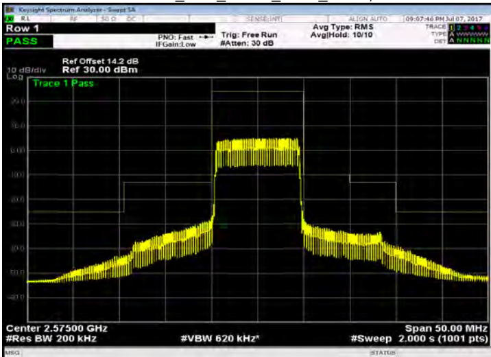
Band 38_10M_QPSK_LOW_RB50,0
