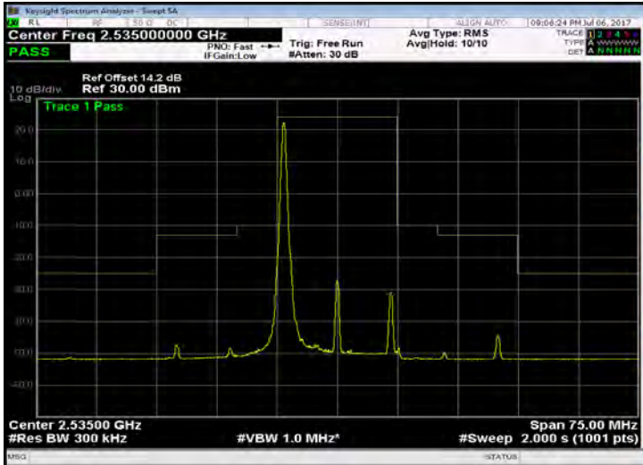
Band 7_15M_16QAM_MID_RB1,74
