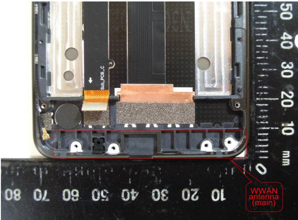
WWAN Antenna (Main)
