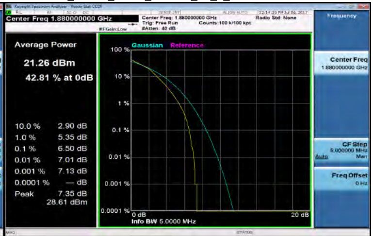
LTE_Band2_5MHz_16QAM_25_0_MidCH18900-1880
