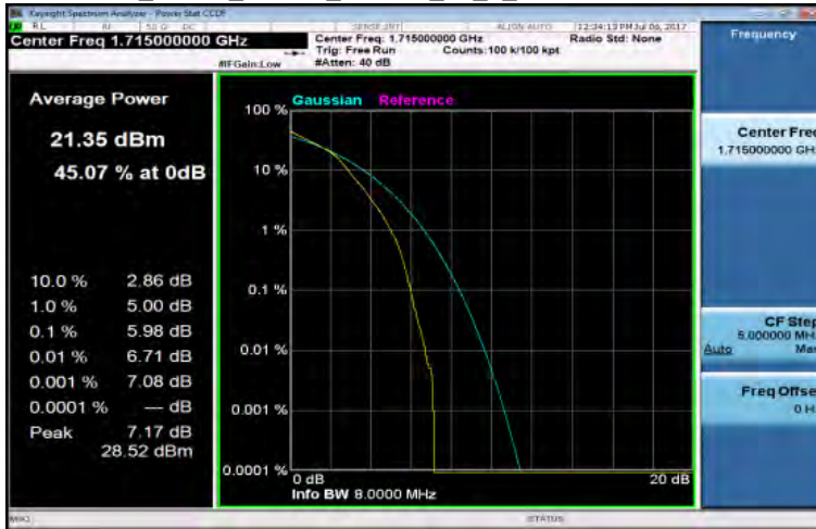
LTE_Band4_10MHz_16QAM_50_0_LowCH20000-1715
