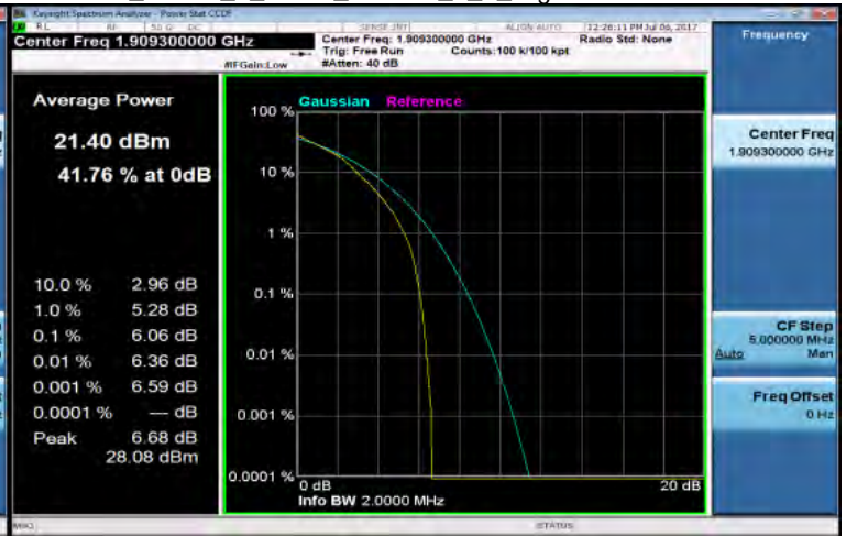
LTE_Band2_1_4MHz_16QAM_6_0_HighCH19193-1909.3
