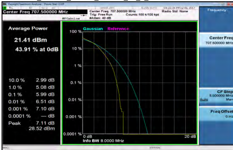
LTE_Band12_10MHz_16QAM_50_0_MidCH23095-707.5
