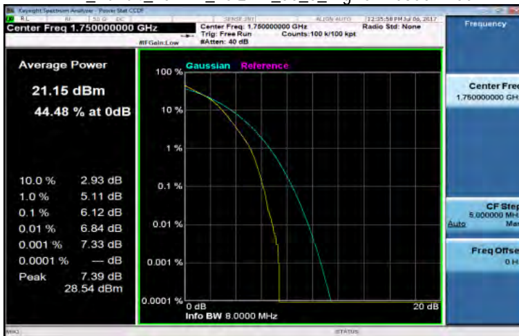
LTE_Band4_10MHz_16QAM_50_0_HighCH20350-1750
