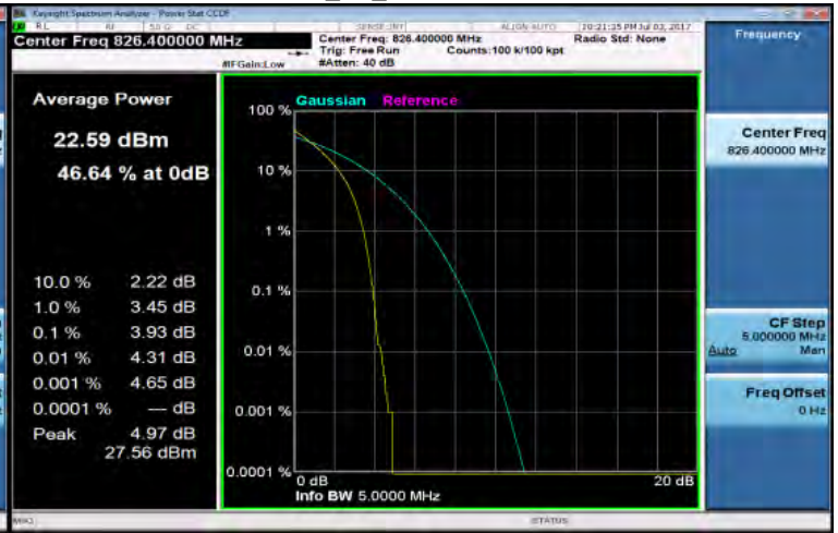
HSDPA_B5_LowCH4132-826.4
