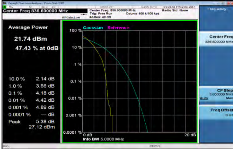
HSUPA_B5_MidCH4183-836.6
