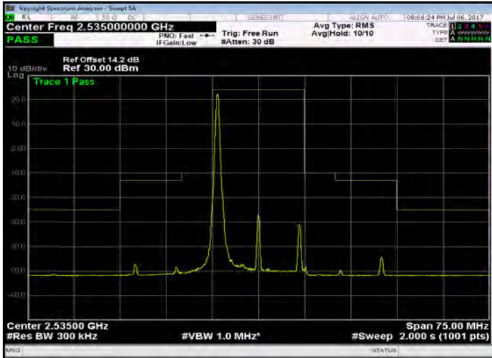
Band 7_15M_16QAM_MID_RB1,74
