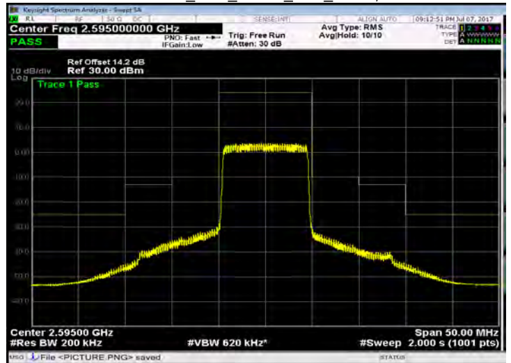
Band 38_10M_QPSK_MID_RB50,0
