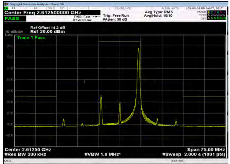
Band 38_15M_16QAM_HIGH_RB75,0
