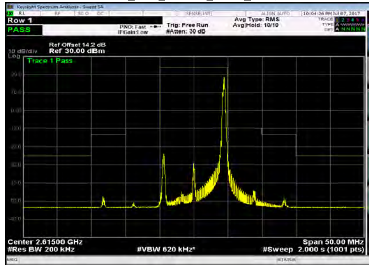
Band 38_10M_16QAM_HIGH_RB50,0
