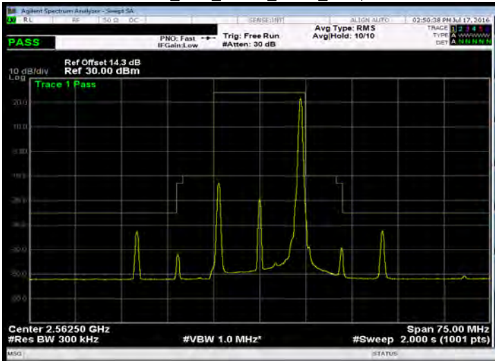
Band 7_15M_QPSK_HIGH_RB75,0
