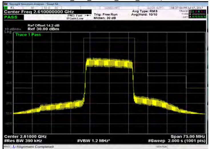
Band 38_20M_16QAM_HIGH_RB100,0
