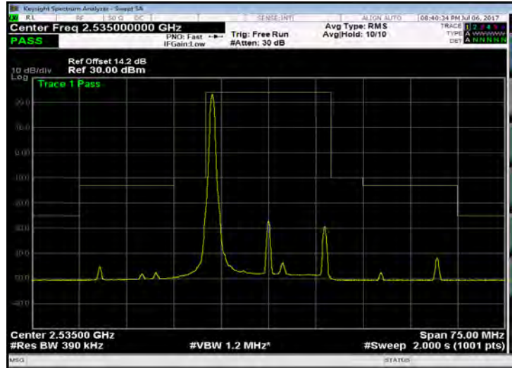
Band 7_20M_QPSK_MID_RB1,99
