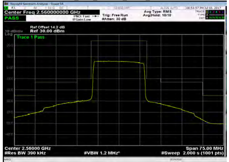
Band 7_20M_16QAM_HIGH_RB100,0
