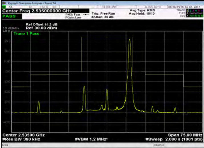
Band 7_20M_16QAM_MID_RB100,0
