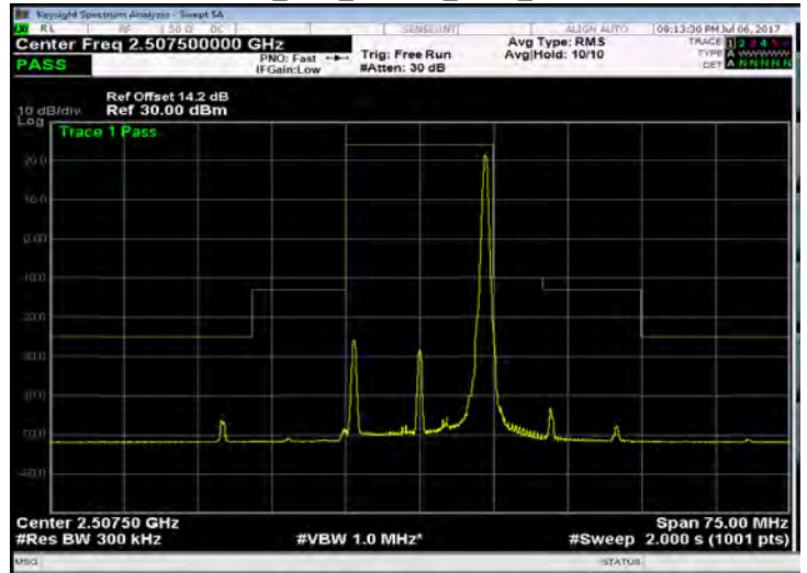
Band 7_15M_16QAM_LOW_RB75,0
