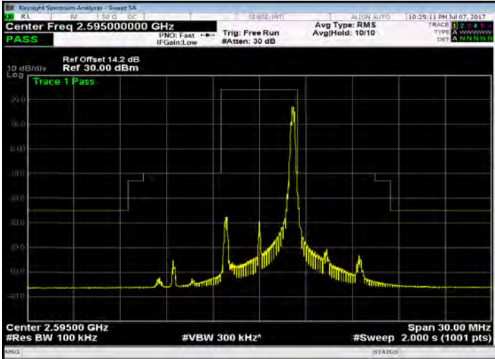
Band 38_5M_16QAM_MID_RB25,0
