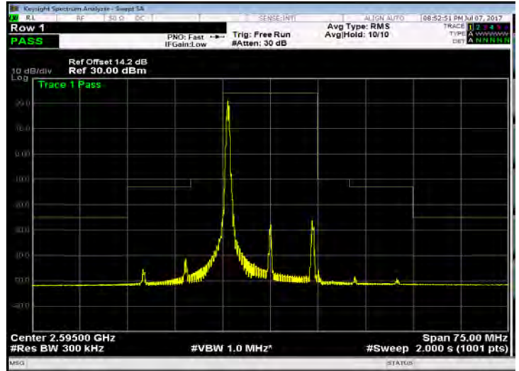
Band 38_15M_QPSK_MID_RB1,74
