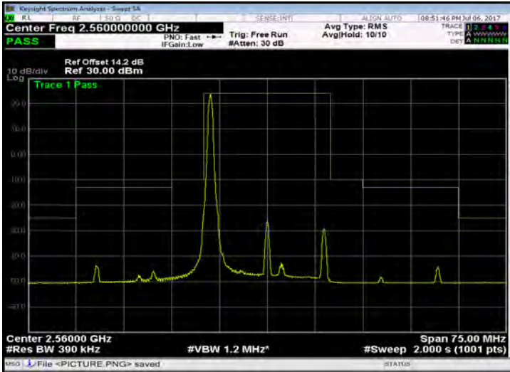
Band 7_20M_QPSK_HIGH_RB1,99
