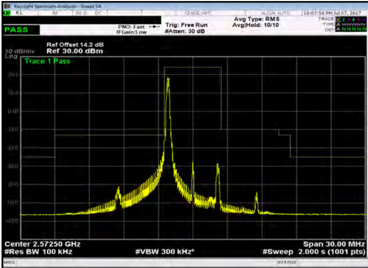
Band 38_5M_QPSK_LOW_RB1,24
