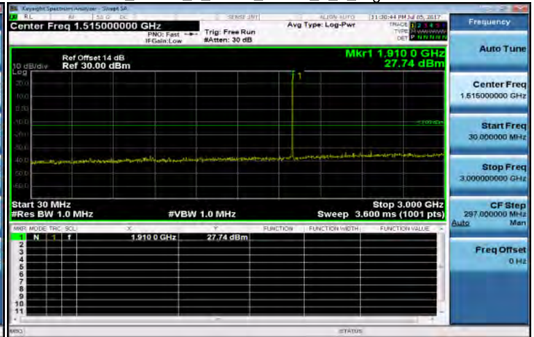
30MHz-3GHz_Band2_1_4MHz_QPSK_1_0_HighCH19193-1909.3
