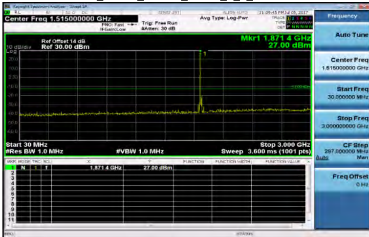
30MHz-3GHz_Band2_20MHz_QPSK_1_0_MidCH18900-1880
