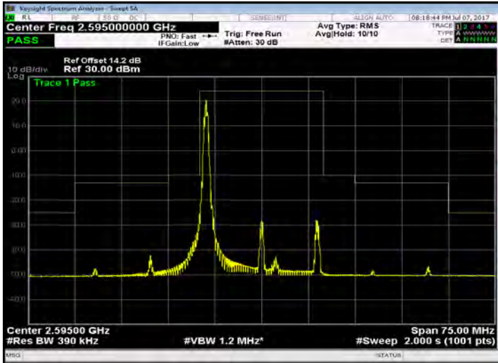
Band 38_20M_16QAM_MID_RB1,99
