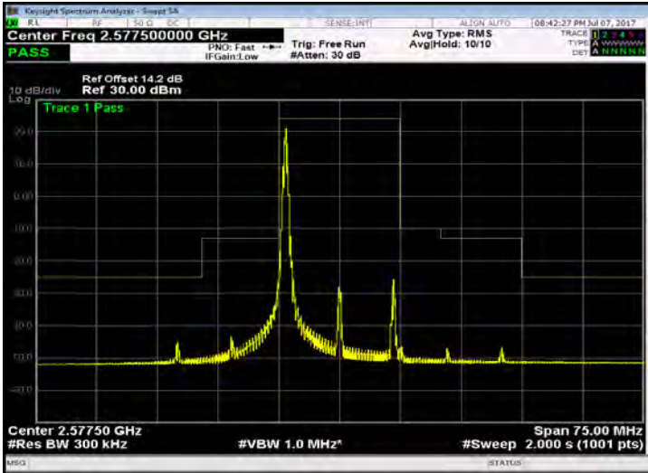
Band 38_15M_QPSK_LOW_RB1,74
