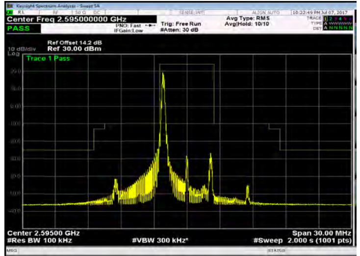
Band 38_5M_QPSK_MID_RB1,24
