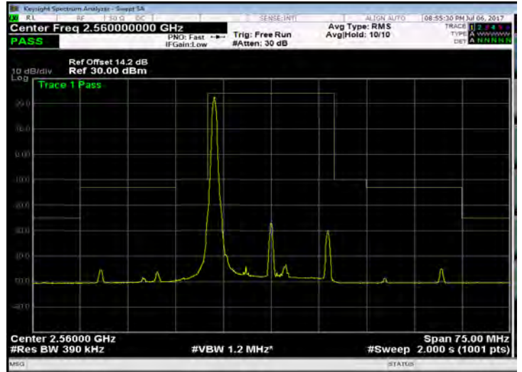
Band 7_20M_16QAM_HIGH_RB1,99
