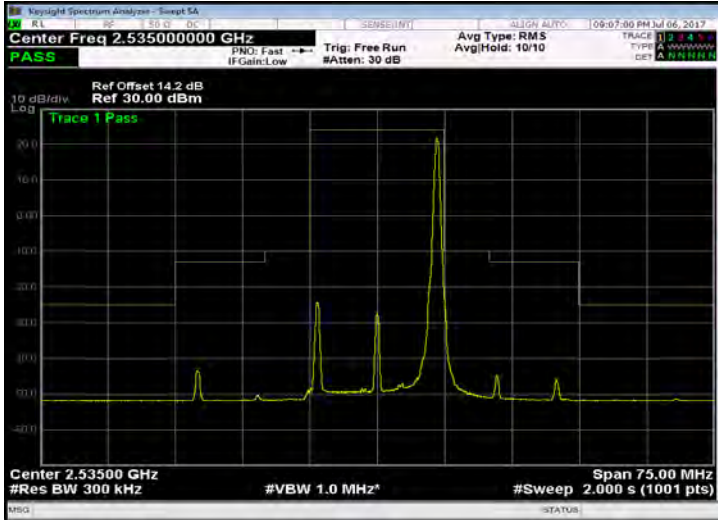
Band 7_15M_16QAM_MID_RB75,0
