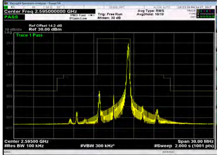
Band 38_5M_QPSK_MID_RB25,0
