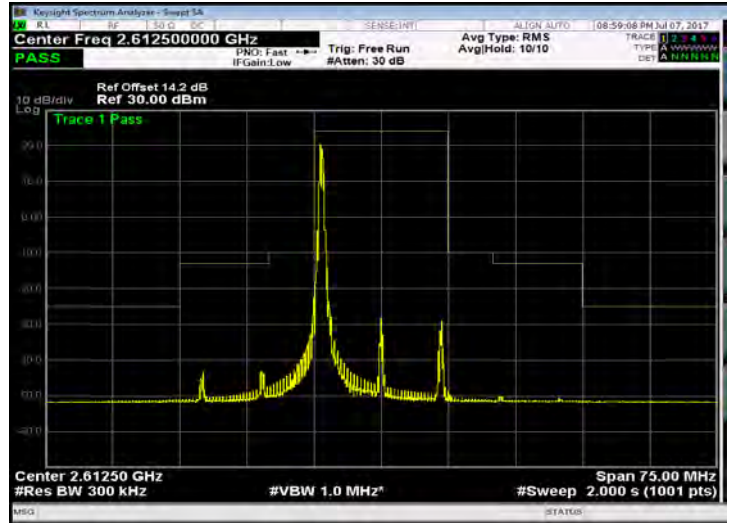
Band 38_15M_16QAM_HIGH_RB1,74
