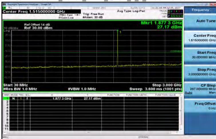
30MHz~3GHz_Band2_5MHz_QPSK_1_0_MidCH18900-1880
