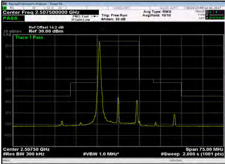
Band 7_15M_QPSK_LOW_RB1,74
