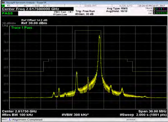
Band 38_5M_QPSK_HIGH_RB25,0
