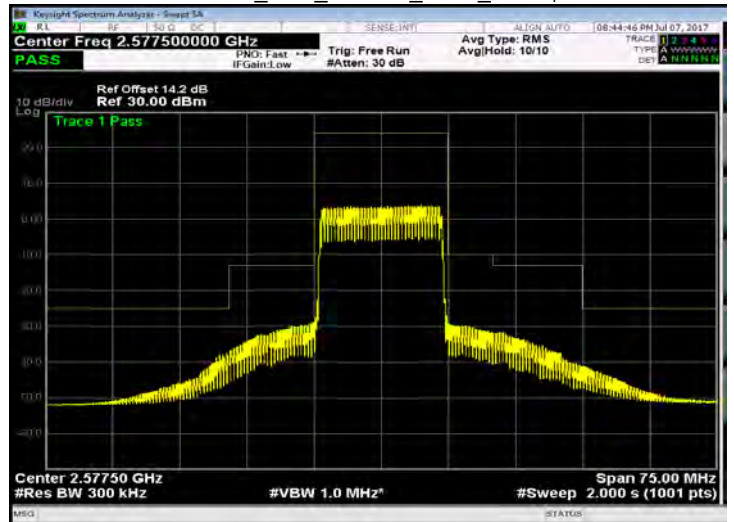
Band 38_15M_16QAM_LOW_RB75,0
