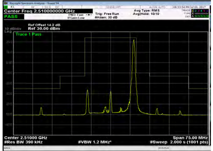
Band 7_20M_16QAM_LOW_RB100,0
