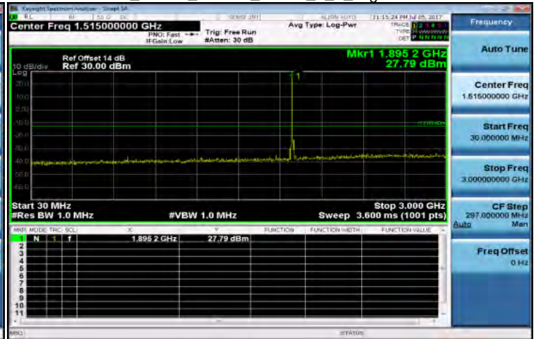
30MHz~3GHz_Band2_15MHz_QPSK_1_0_HighCH19125-1902.5
