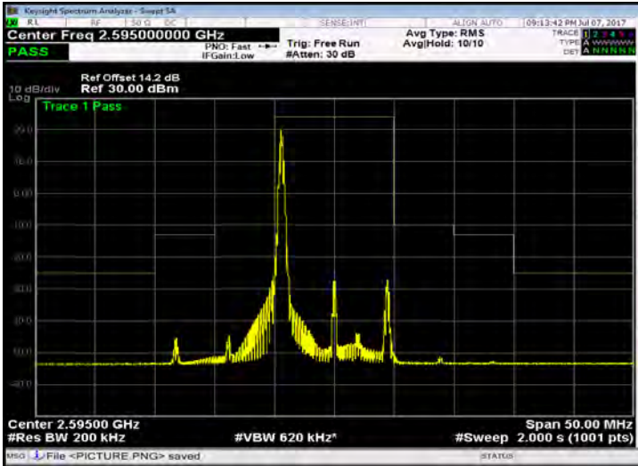
Band 38_10M_16QAM_MID_RB1,49
