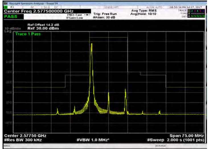
Band 38_15M_16QAM_LOW_RB1,74
