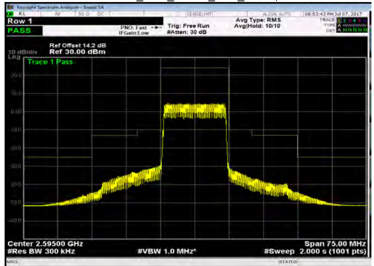
Band 38_15M_QPSK_MID_RB75,0
