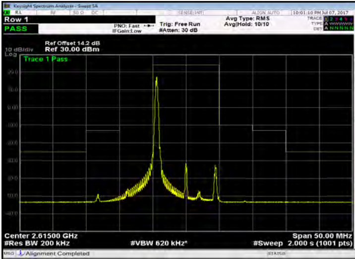
Band 38_10M_QPSK_HIGH_RB1,49
