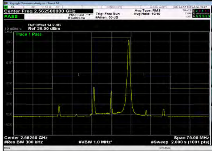
Band 7_15M_16QAM_HIGH_RB75,0
