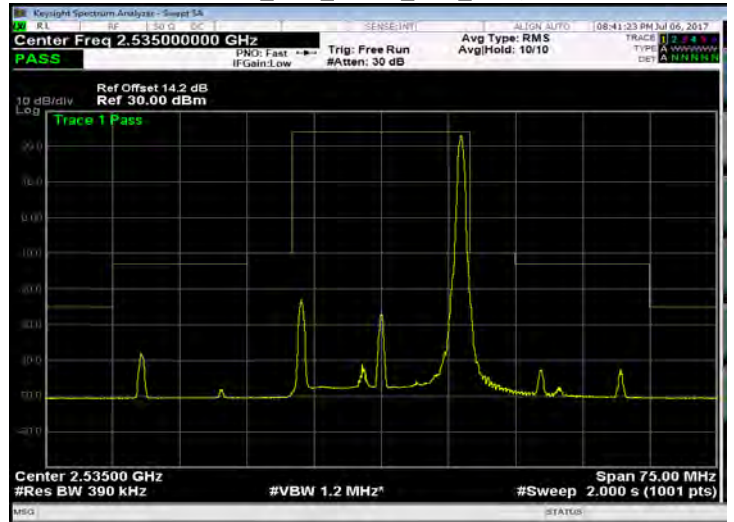
Band 7_20M_QPSK_MID_RB100,0
