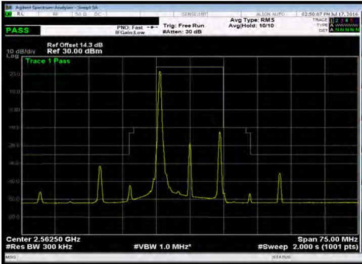
Band 7_15M_QPSK_HIGH_RB1,74
