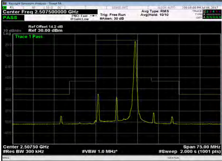
Band 7_15M_QPSK_LOW_RB75,0
