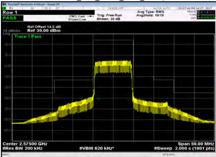
Band 38_10M_QPSK_LOW_RB50,0
