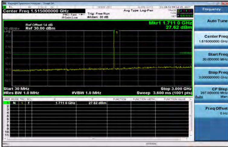
30MHz~3GHz_Band4_10MHz_QPSK_1_0_LowCH20000-1715
