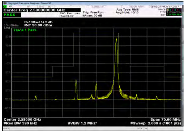
Band 38_20M_16QAM_LOW_RB100,0
