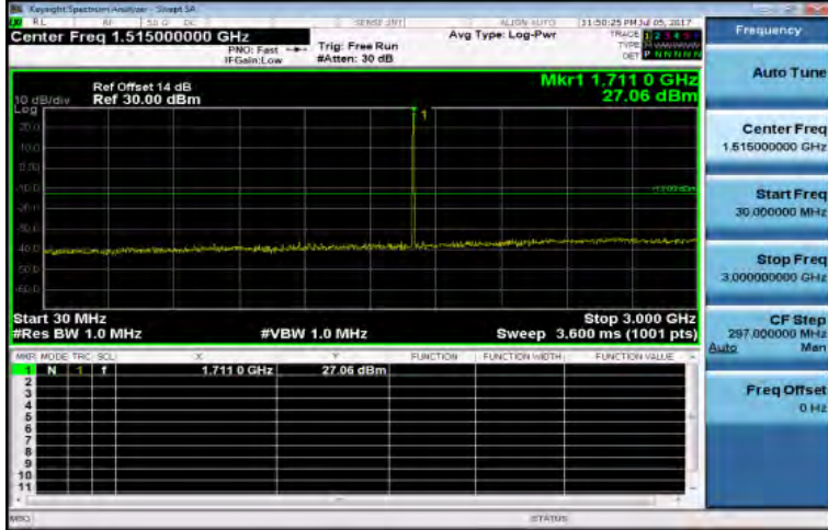
30MHz-3GHz_Band4_3MHz_QPSK_1_0_LowCH19965-1711.5
