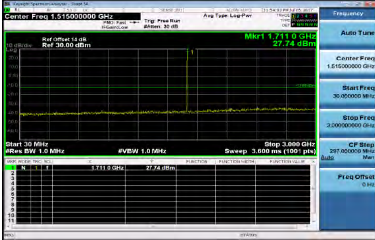
30MHz-3GHz_Band4_1_4MHz_QPSK_1_0_LowCH19957-1710.7
