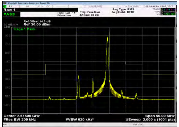
Band 38_10M_16QAM_LOW_RB50,0
