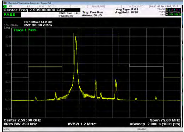
Band 38_20M_QPSK_MID_RB1,99
