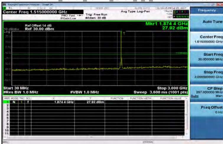
30MHz~3GHz_Band2_15MHz_QPSK_1_0_MidCH1890-1880
