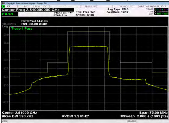
Band 7_20M_QPSK_LOW_RB100,0
