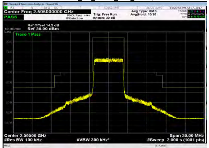
Band 38_5M_QPSK_MID_RB25,0
