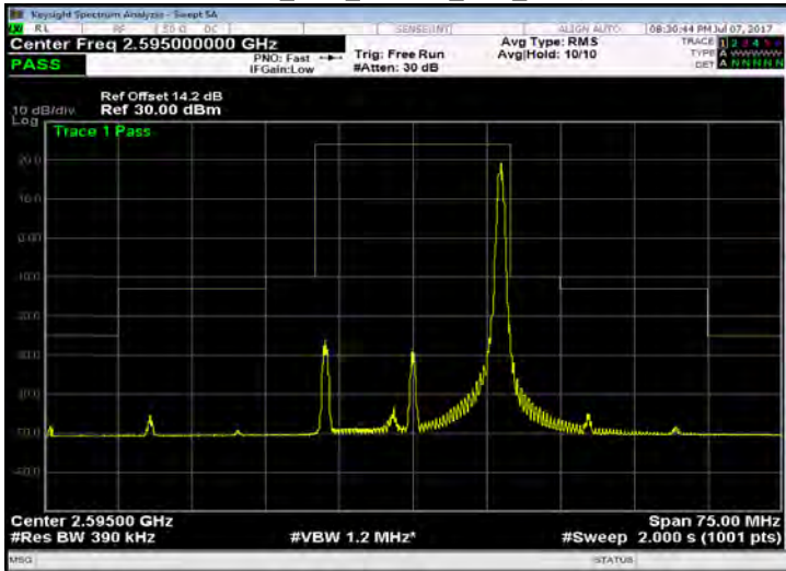
Band 38_20M_16QAM_MID_RB100,0
