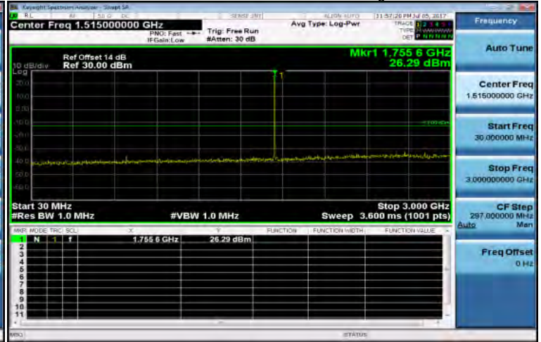
30MHz-3GHz_Band4_1_4MHz_QPSK_1_0_HighCH20393-1754.3
