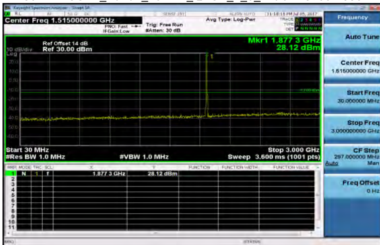
30MHz-3GHz_Band2_10MHz_QPSK_1_0_MidCH18900-1880
