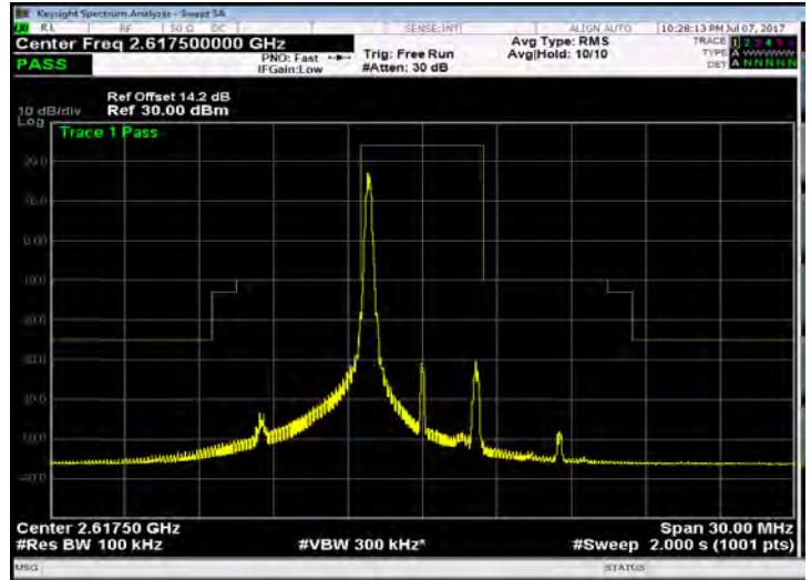
Band 38_5M_16QAM_HIGH_RB1,24
