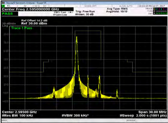
Band 38_5M_16QAM_MID_RB1,24
