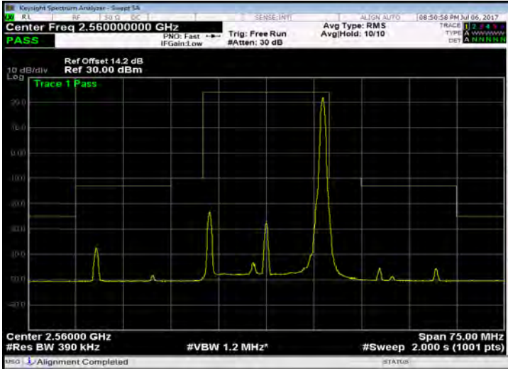
Band 7_20M_QPSK_HIGH_RB100,0
