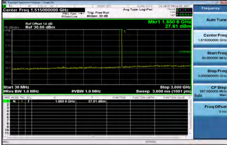
30MHz-3GHz_Band2_1_4MHz_QPSK_1_0_LowCH18607-1850.7
