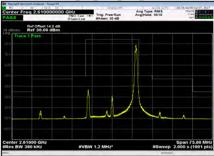
Band 38_20M_QPSK_HIGH_RB100,0
