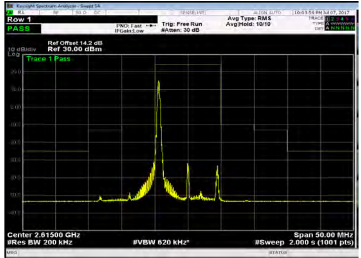
Band 38_10M_16QAM_HIGH_RB1,49
