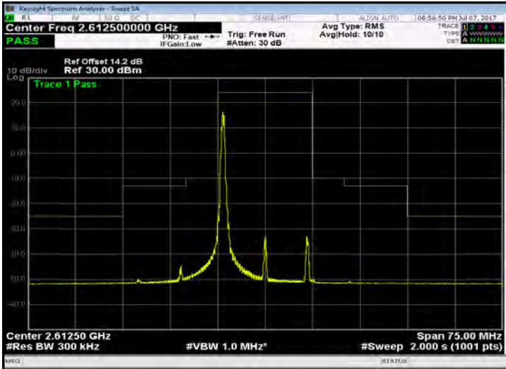
Band 38_15M_QPSK_HIGH_RB1,74
