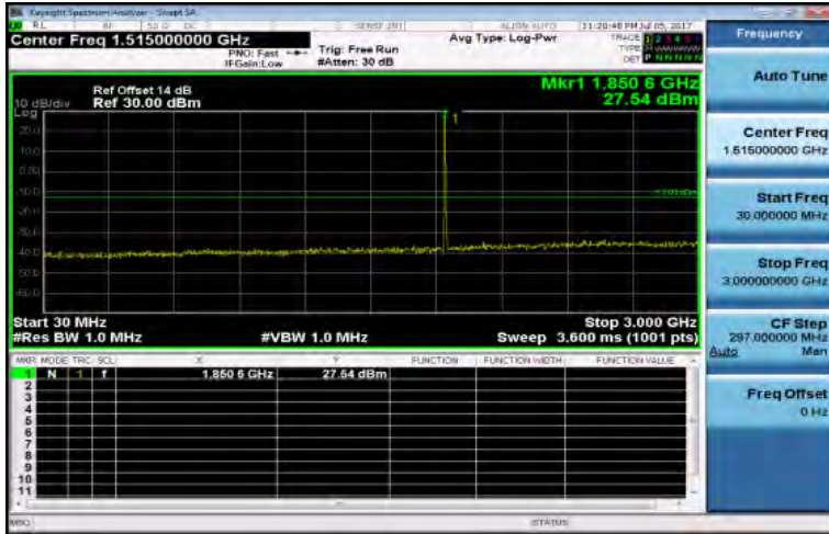
30MHz~3GHz_Band2_5MHz_QPSK_1_0_LowCH18625-1852.5
