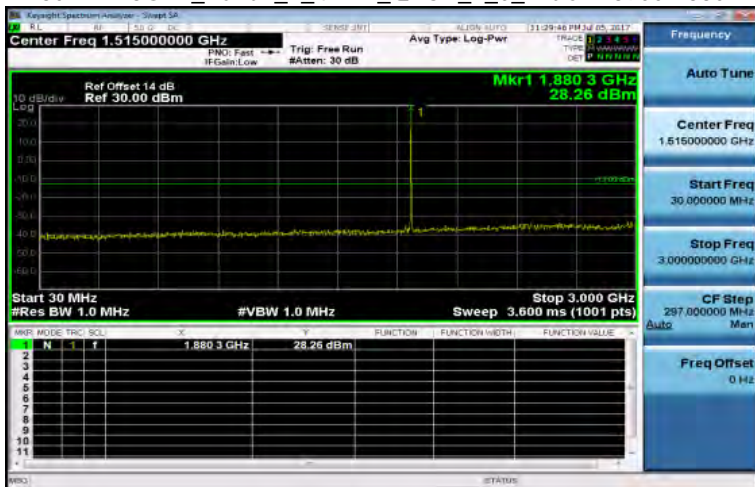
30MHz-3GHz_Band2_1_4MHz_QPSK_1_0_MidCH18900-1880
