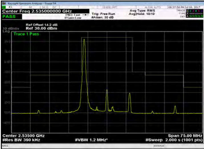
Band 7_20M_16QAM_MID_RB1,99
