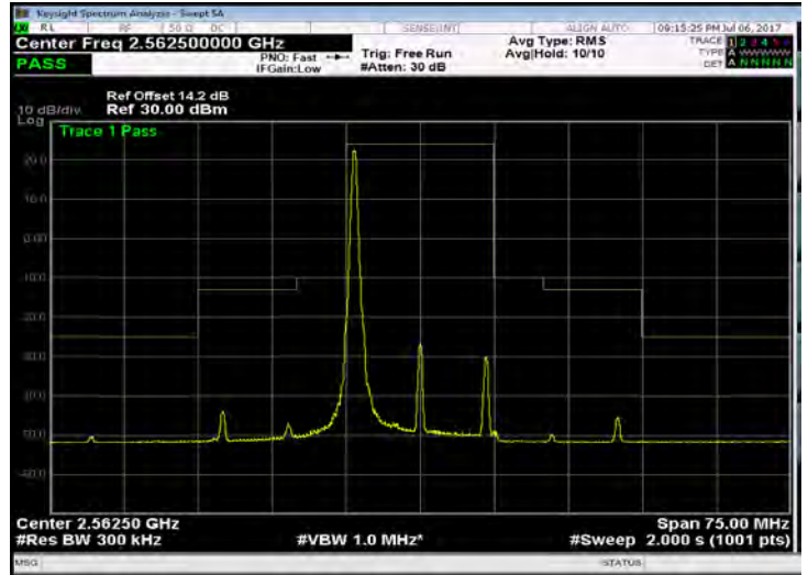
Band 7_15M_16QAM_HIGH_RB1,74
