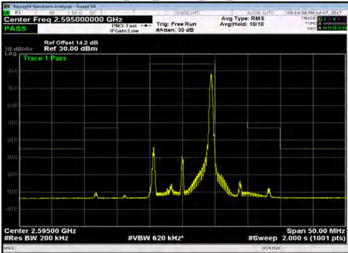
Band 38_10M_16QAM_MID_RB50,0
