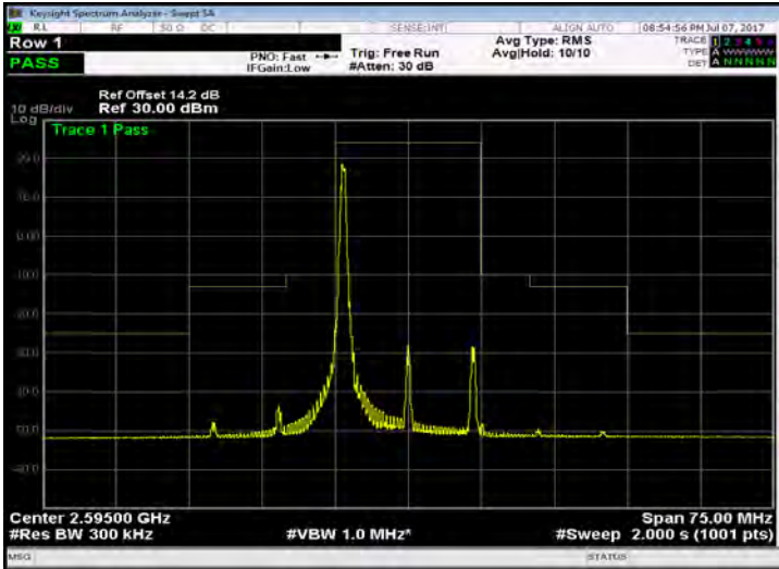
Band 38_15M_16QAM_MID_RB1,74
