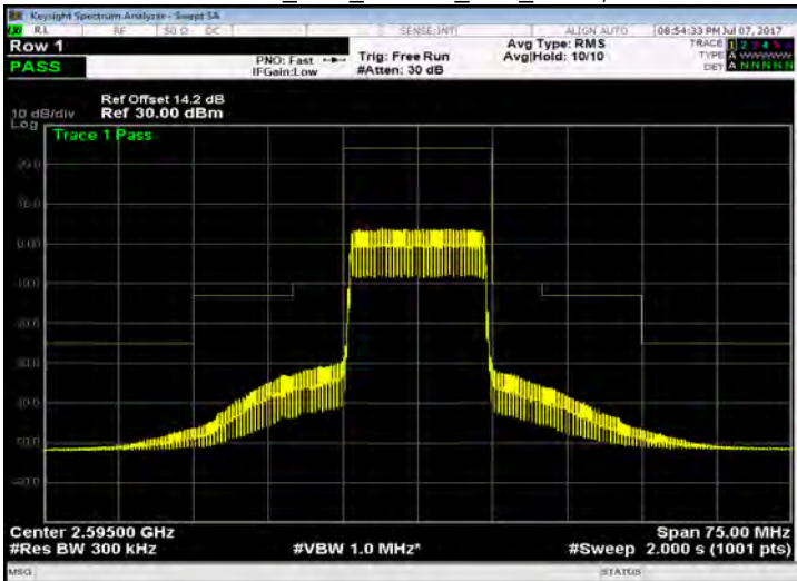
Band 38_15M_16QAM_MID_RB75,0
