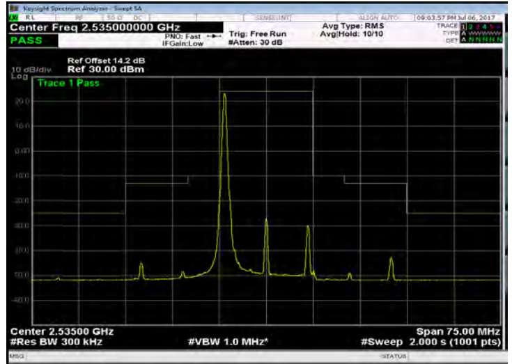
Band 7_15M_QPSK_MID_RB1,74
