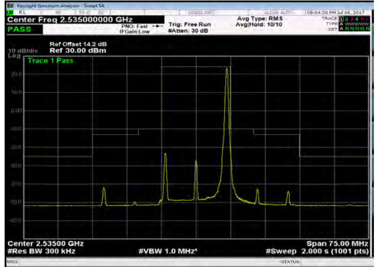
Band 7_15M_QPSK_MID_RB75,0
