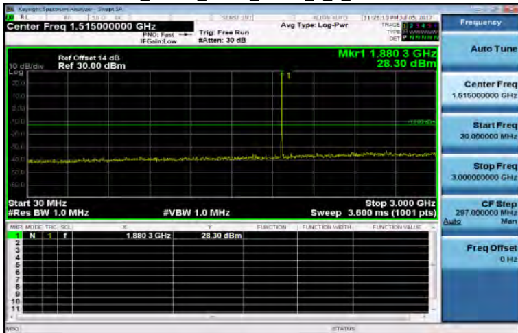
30MHz~3GHz_Band2_3MHz_QPSK_1_0_MidCH18900-1880
