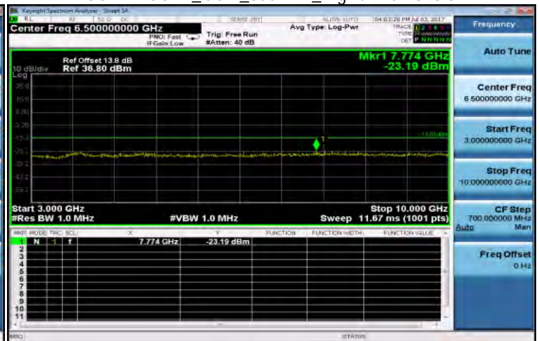
3GHz-10GHz_GSM_850MHz_HighCH251-848.8
