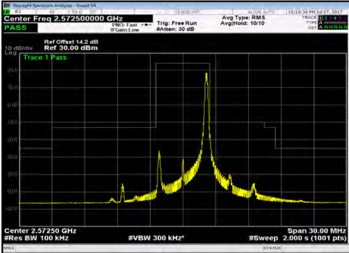
Band 38_5M_QPSK_LOW_RB25,0
