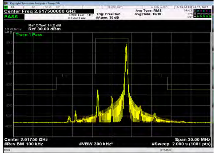
Band 38_5M_16QAM_HIGH_RB25,0
