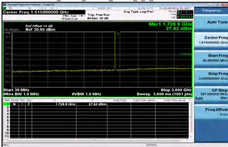
30MHz~3GHz_Band4_10MHz_QPSK_1_0_MidCH20175-1732.5
