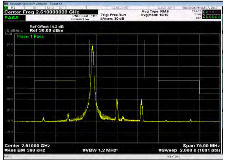
Band 38_20M_16QAM_HIGH_RB1,99
