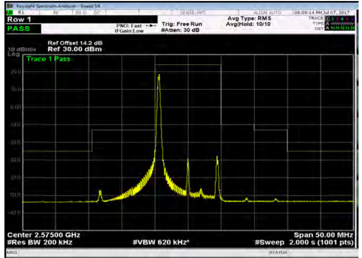
Band 38_10M_16QAM_LOW_RB1,49
