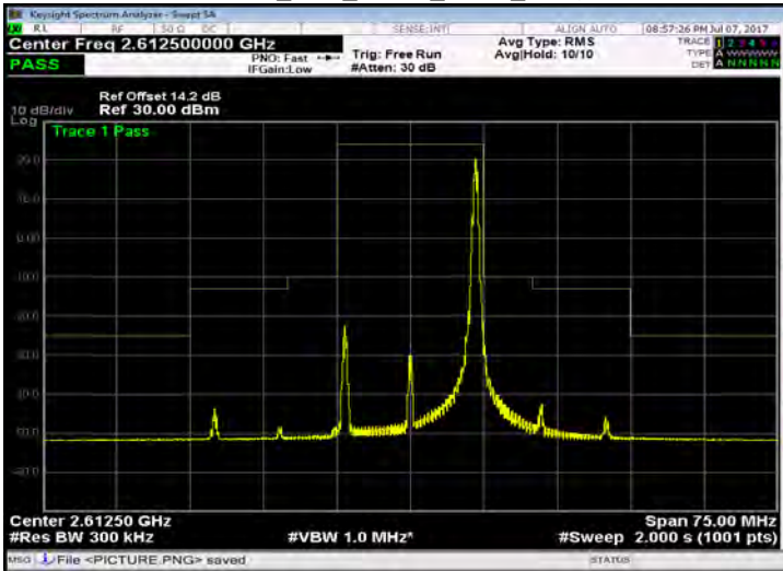
Band 38_15M_QPSK_HIGH_RB75,0
