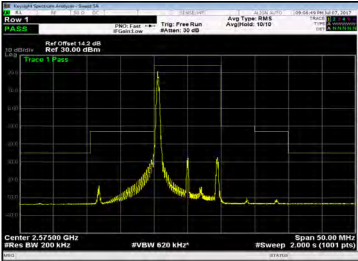
Band 38_10M_QPSK_LOW_RB1,49
