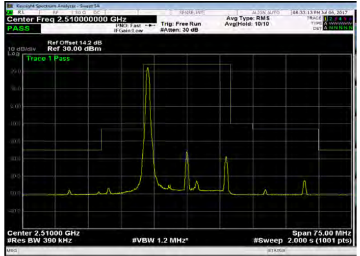
Band 7_20M_16QAM_LOW_RB1,99
