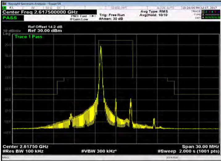
Band 38_5M_QPSK_HIGH_RB1,24
