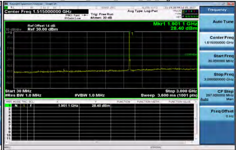
30MHz-3GHz_Band2_10MHz_QPSK_1_0_HighCH19150-1905
