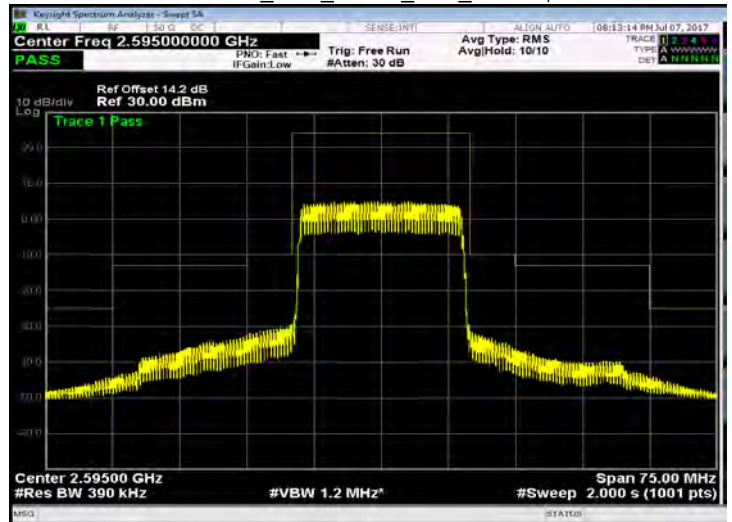
Band 38_20M_QPSK_MID_RB100,0
