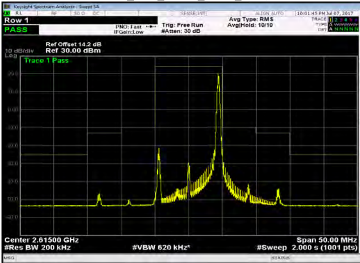
Band 38_10M_QPSK_HIGH_RB50,0
