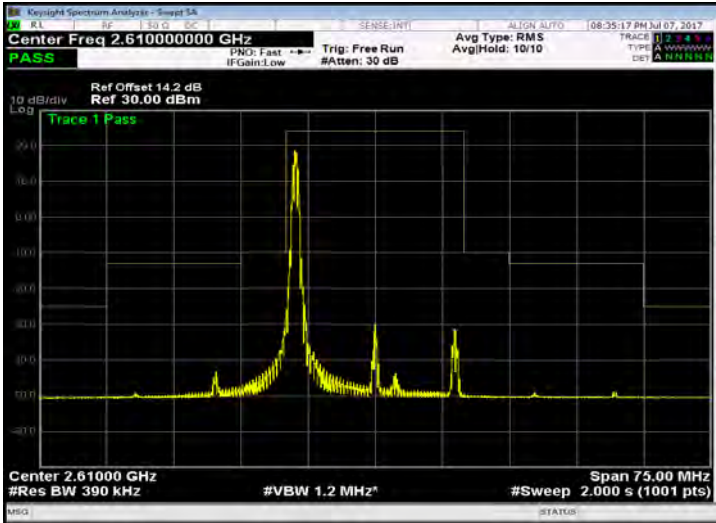
Band 38_20M_QPSK_HIGH_RB1,99
