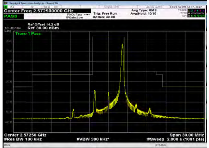
Band 38_5M_16QAM_LOW_RB25,0
