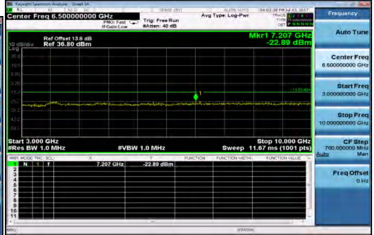
3GHz-10GHz_GSM_850MHz_MidCH190-836.6
