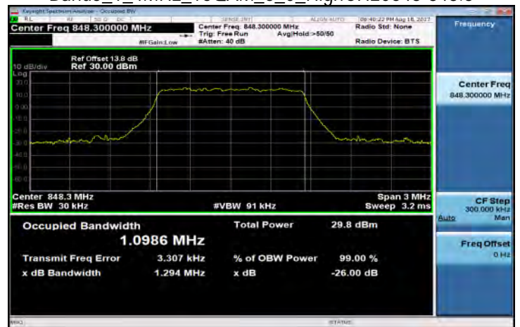
Band5_1_4MHz_16QAM_6_0_HighCH20643-848.3
