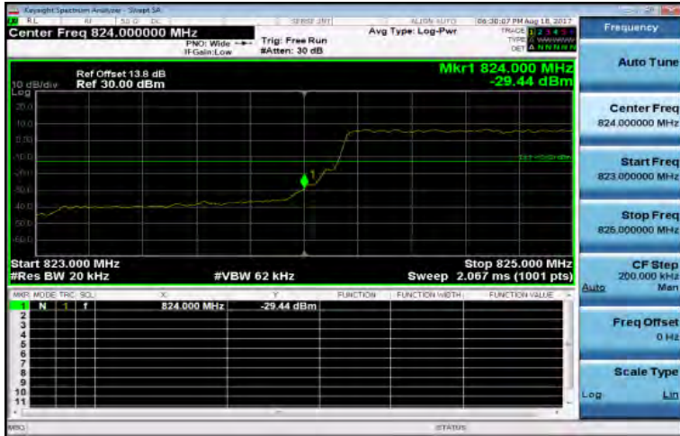
Band5_1_4MHz_QPSK_6_0_LowCH20407-824.7
