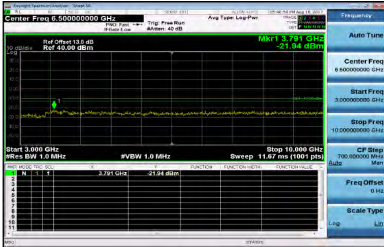
3GHz~10GHz_Band5_5MHz_QPSK_1_0_LowCH20425-826.5
