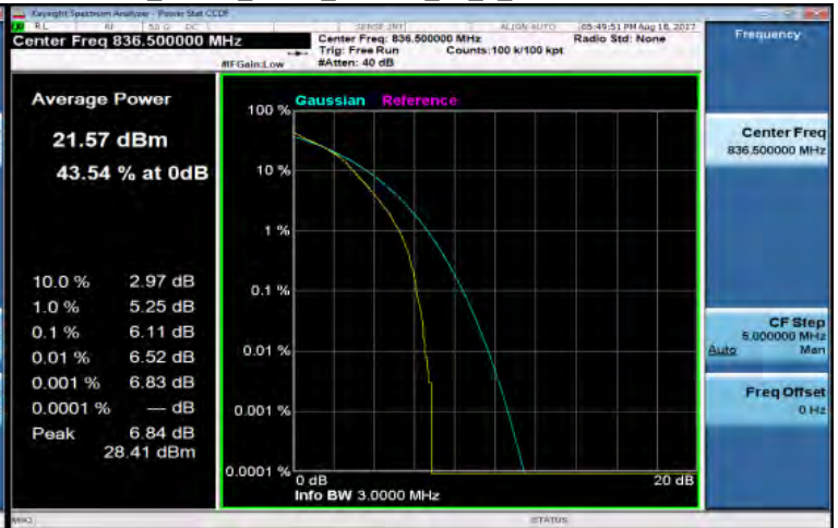
LTE_Band5_3MHz_16QAM_15_0_MidCH20525-836.5
