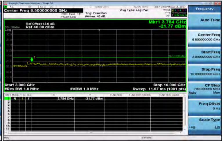
3GHz~10GHz_Band5_5MHz_QPSK_1_0_MidCH20525-836.5
