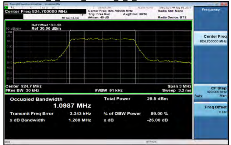
Band5_1_4MHz_16QAM_6_0_LowCH20407-824.7
