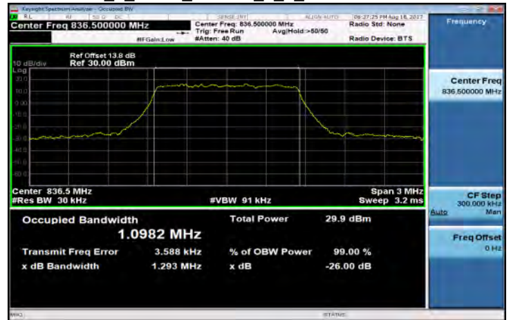
Band5_1_4MHz_16QAM_6_0_MidCH20525-836.5
