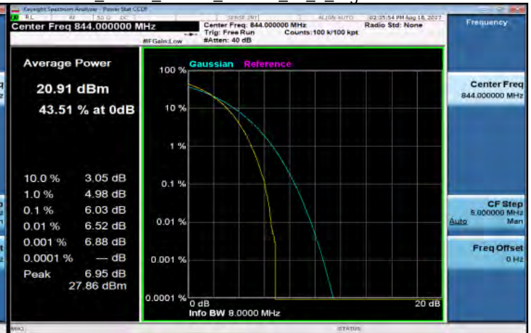
LTE_Band5_10MHz_16QAM_50_0_HighCH20600-844
