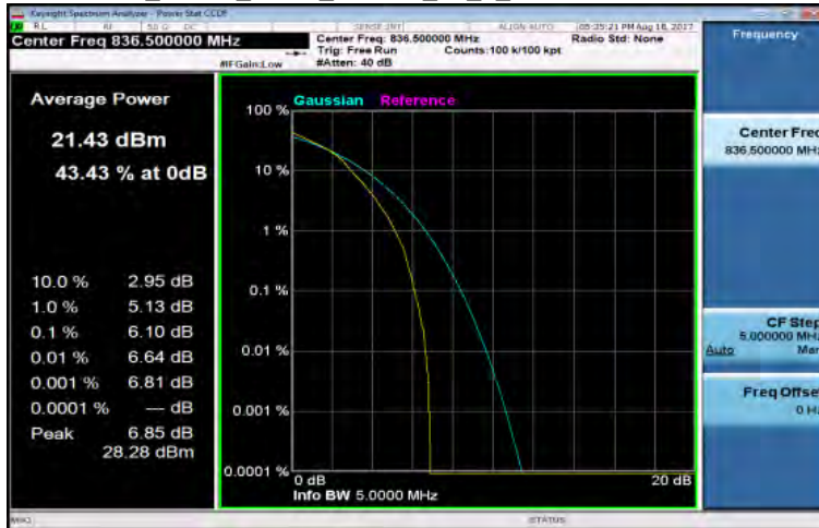
LTE_Band5_5MHz_16QAM_25_0_MidCH20525-836.5
