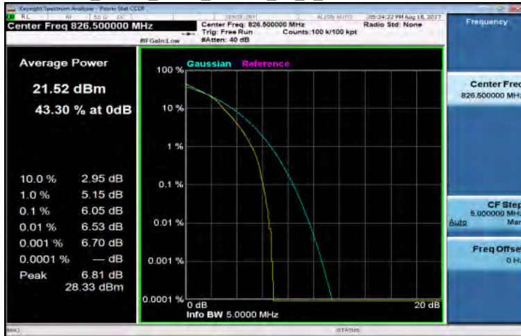
LTE_Band5_5MHz_16QAM_25_0_LowCH20425-826.5
