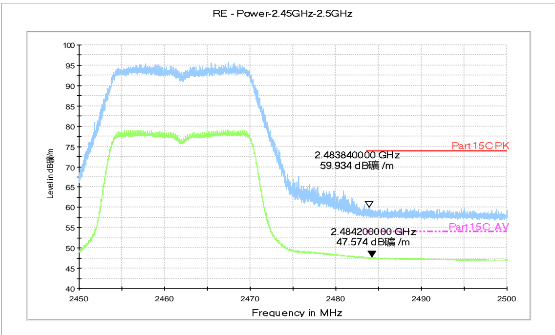
Fig.A.6.2.18 Transmitter Spurious Emission - Radiated (Power): 802.11g, ch11, 2.45 GHz - 2.50GHz
