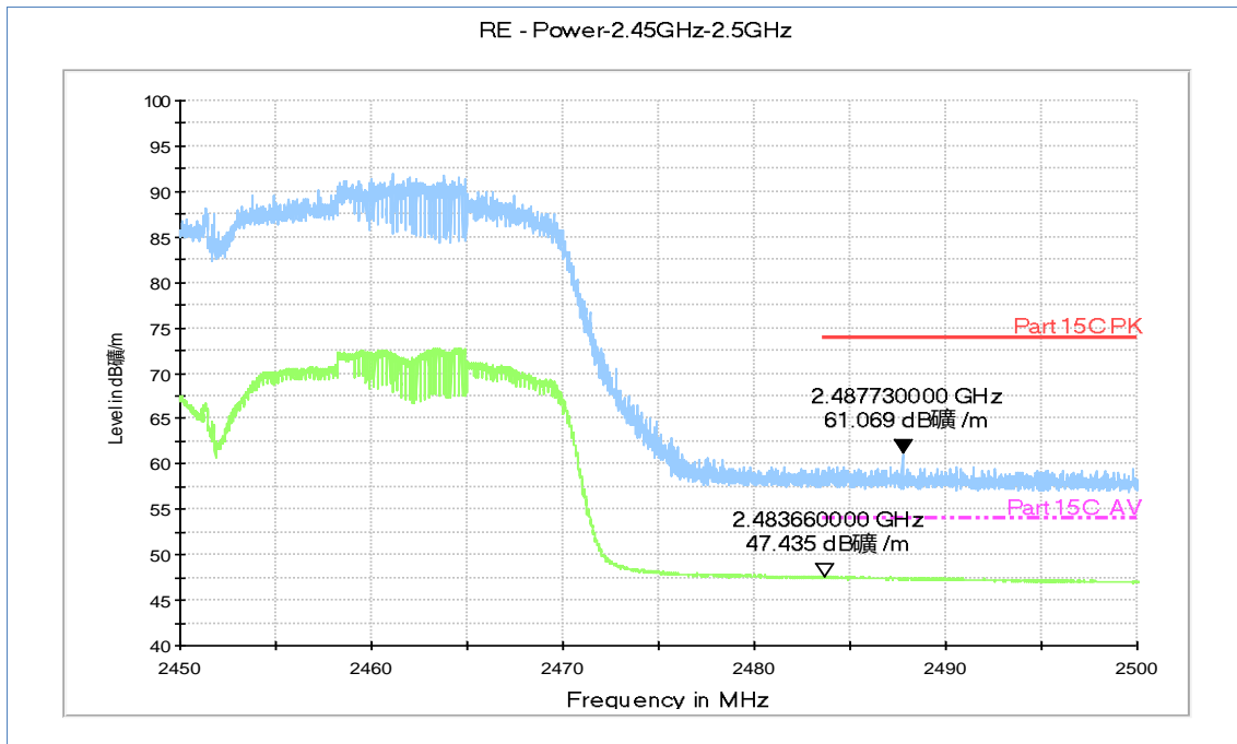
Fig.A.6.2.38 Transmitter Spurious Emission - Radiated (Power): 802.11n-HT40, ch9, 2.45 GHz - 2.50GHz
