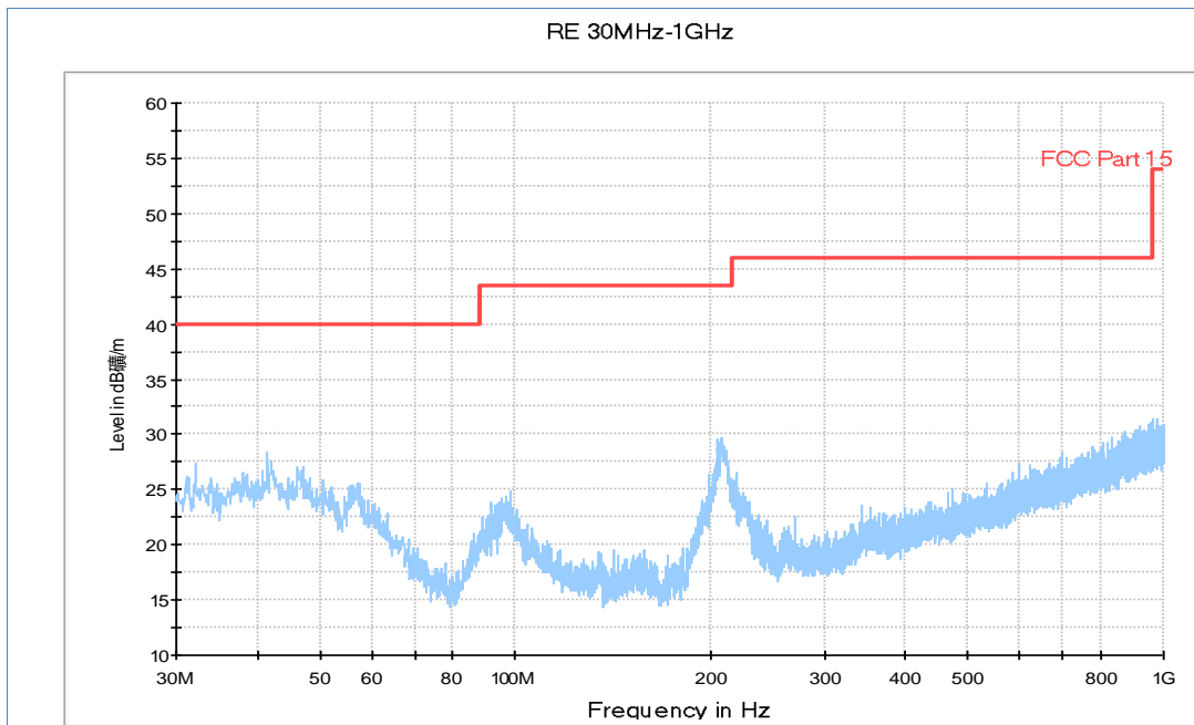
Fig.A.6.2.24 Transmitter Spurious Emission - Radiated (802.11n-HT20, Ch6, 30 MHz-1 GHz)
