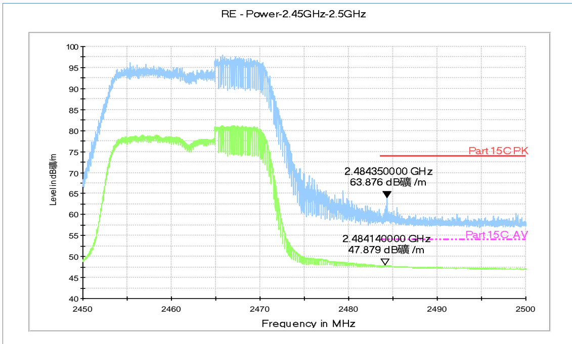
Fig.A.6.2.28 Transmitter Spurious Emission - Radiated (Power): 802.11n-HT20, ch11, 2.45 GHz - 2.50GHz
