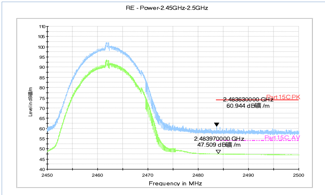
Fig.A.6.2.8 Transmitter Spurious Emission - Radiated (Power): 802.11b, ch11, 2.45 GHz - 2.50GHz
