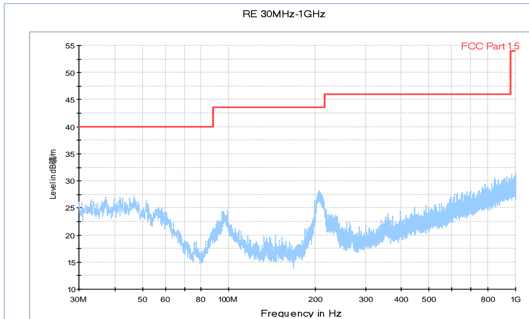
Fig.A.6.2.34 Transmitter Spurious Emission - Radiated (802.11n-HT40, Ch6, 30 MHz-1 GHz)
