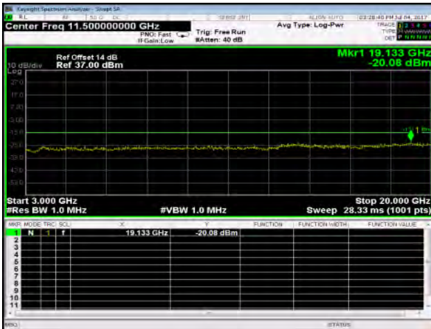
Out of Band Emission Low_WCDMA_B5_LowCH4132-826.4
