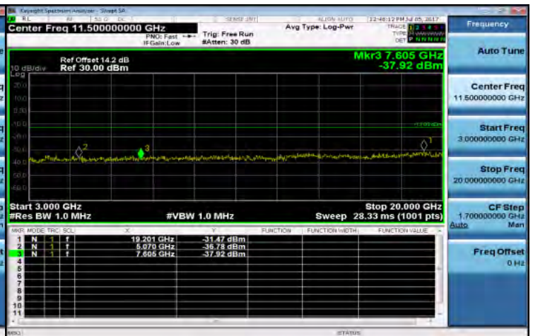
Out of Band Emission High_Band7 20MHz_QPSK 1_0_HighCH21350-2560
