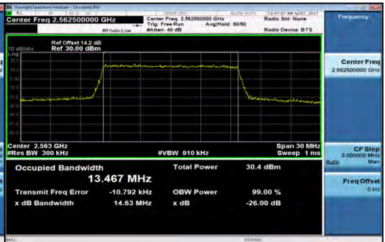
Band7 15MHz_16-QAM 75 0_HighCH21375-2562.5
