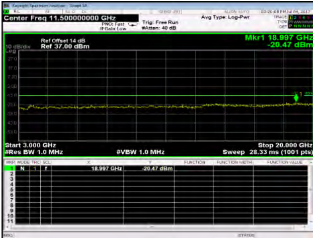
Out of Band Emission Low_WCDMA_B2_HighCH9538-1907.6
