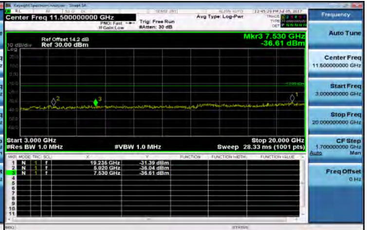
Out of Band Emission High_Band7 20MHz_QPSK 1_0_MidCH21100-2535
