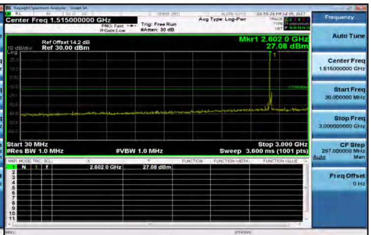
Out of Band Emission Low_Band38 20MHz_QPSK 1 0_HighCH38150-2610
