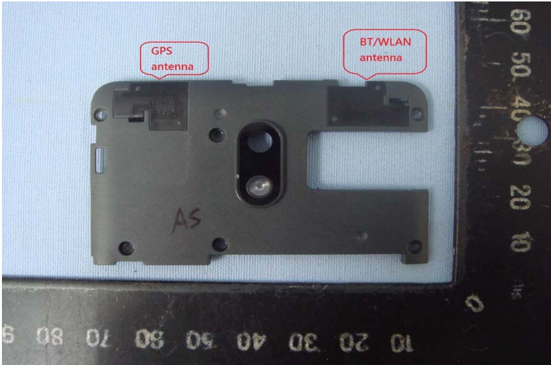
BT/WLAN/GPS Antenna
