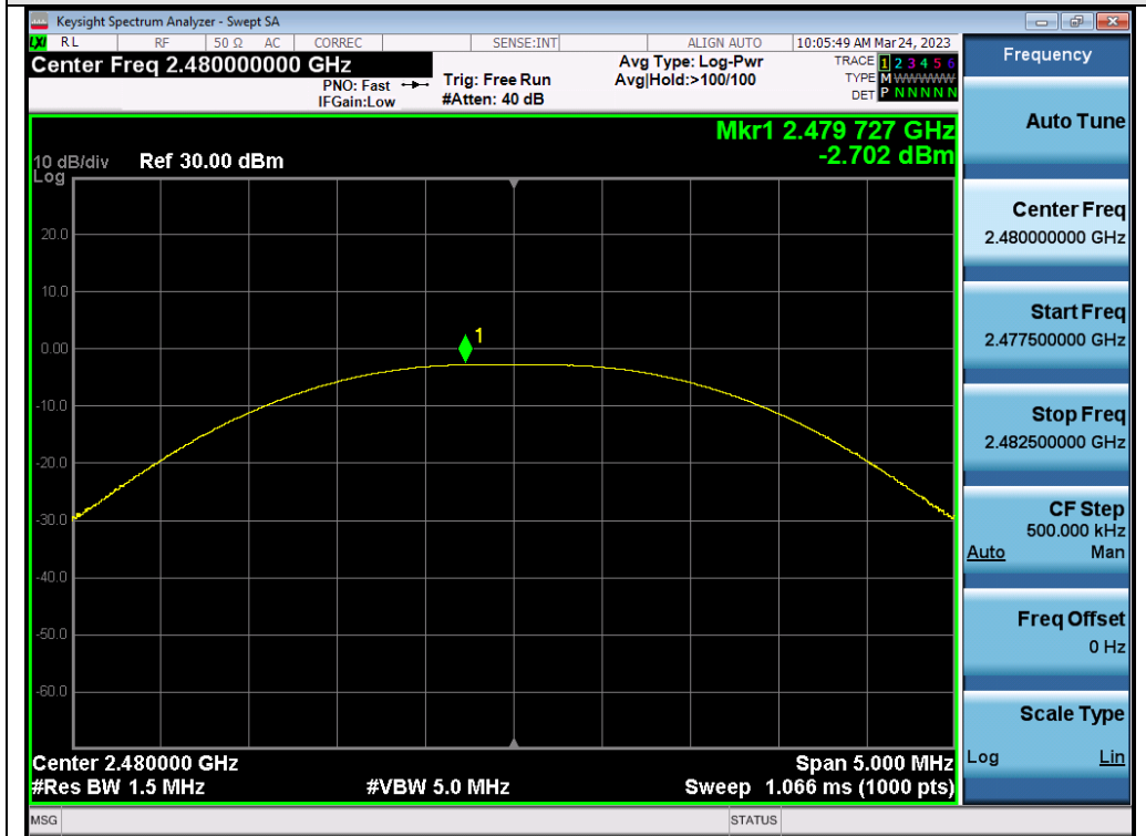
Test_Graph_LE1M_ANT1_2480_1Mbps_Peak Power
