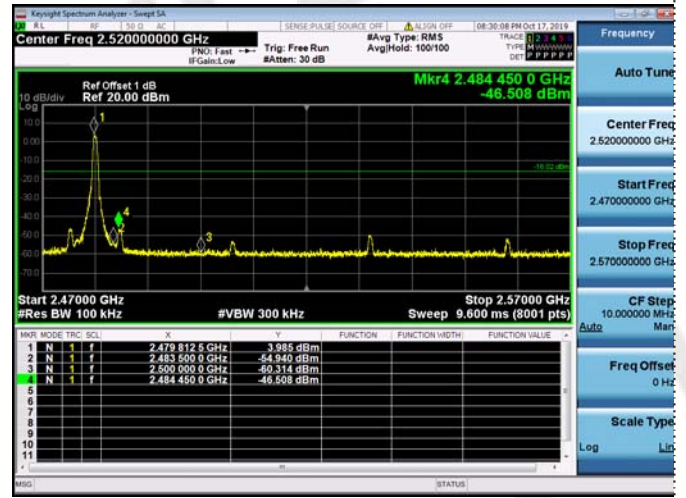
Right bandedge
