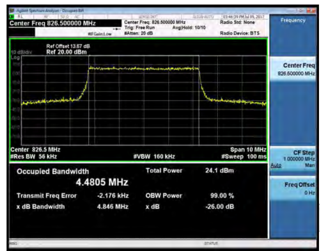
LTE band 5 - Low CH 16QAM-5
