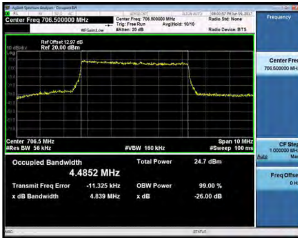
LTE band 17 - Low CH QPSK-5
