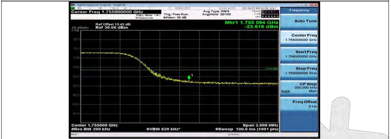
Channel Bandwidth: 10 MHz_HCH_16QAM_50RB#0
