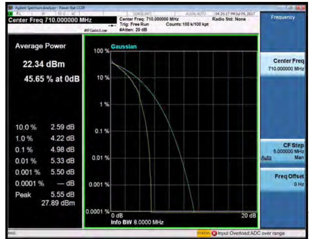
Band 17(Channel Bandwidth: 5MHz)-16QAM
