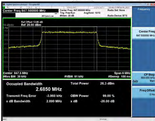
LTE band 5 - High CH QPSK-3
