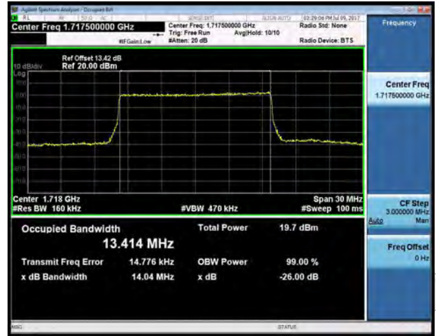
LTE band 4 - Low CH 16QAM-15
