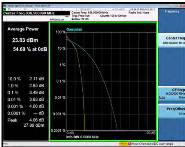
Band 5(Channel Bandwidth: 10 MHz)-QPSK
