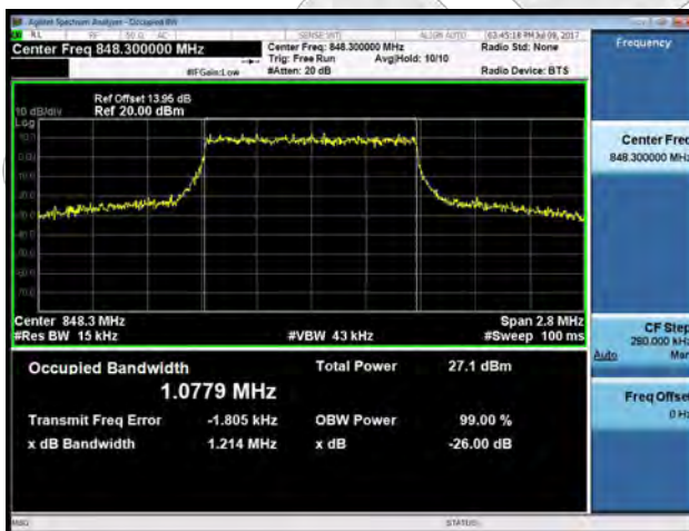
LTE band 5 - High CH QPSK-1.4
