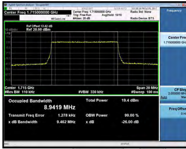
LTE band 4 - Low CH 16QAM-10
