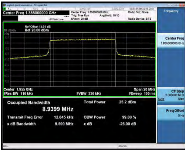
LTE band 2 - Low CH QPSK-10
