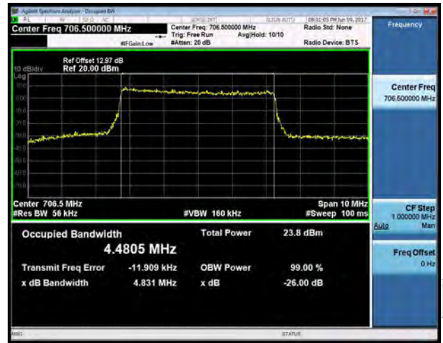
LTE band 17 - Low CH 16QAM-5
