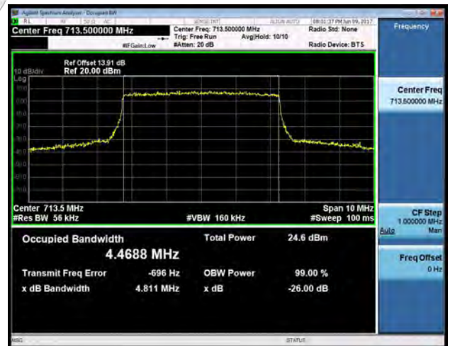
LTE band 17 - High CH 16QAM-5
