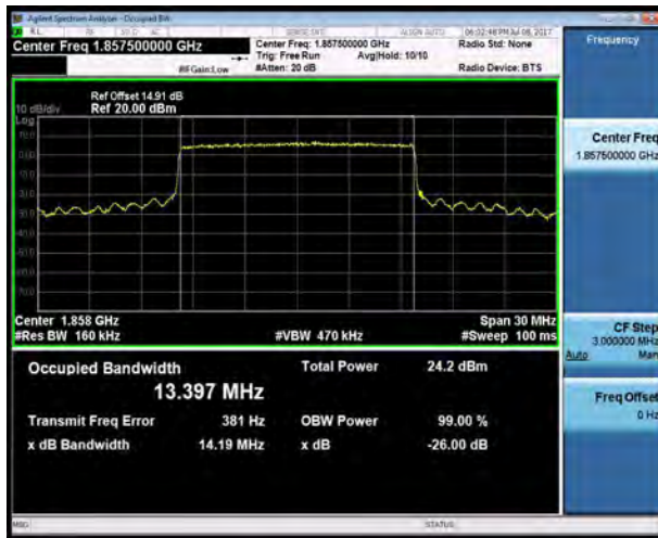
LTE band 2 - Low CH QPSK-15
