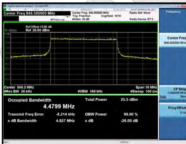
LTE band 5 - High CH QPSK-5
