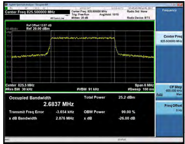
LTE band 5 - Low CH 16QAM-3
