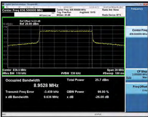
LTE band 5 - Middle CH QPSK-10
