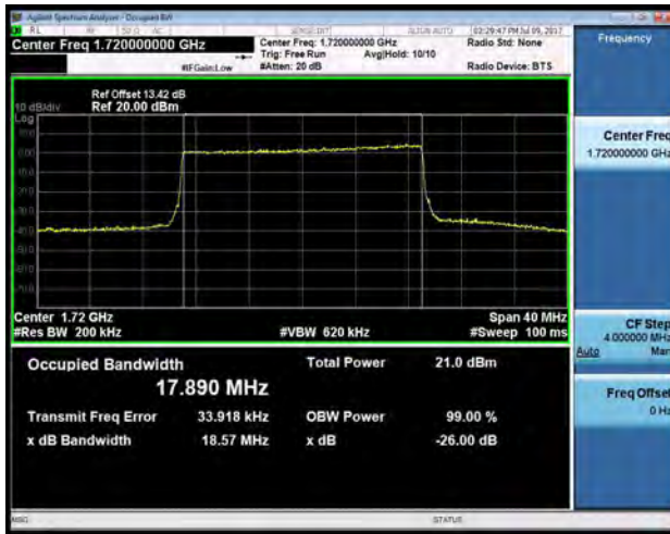
LTE band 4 - Low CH QPSK-20
