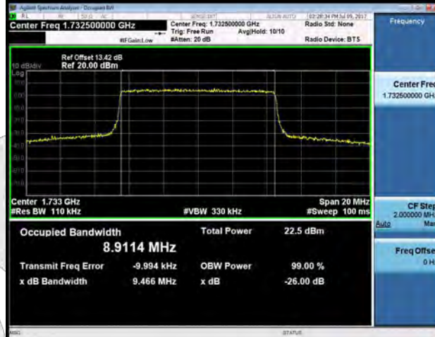
LTE band 4 - Middle CH 16QAM-10
