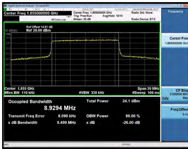
LTE band 2 - Low CH 16QAM-10
