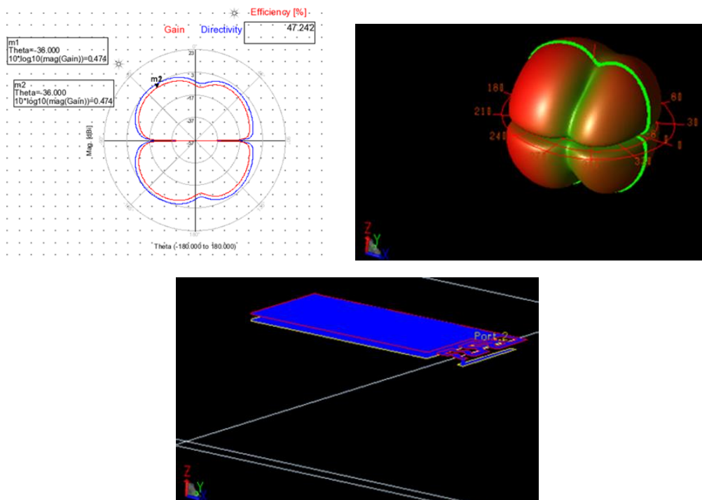
Figure 2-2: Radiation Pattern
