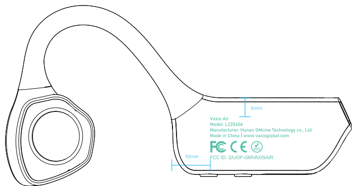
logo丝印白色, 尺寸5*5mm
