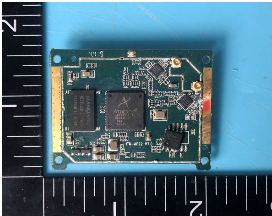
Photo 16(Receiver)
