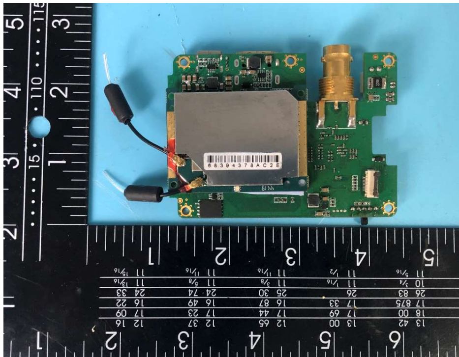
Photo 6(Receiver)
