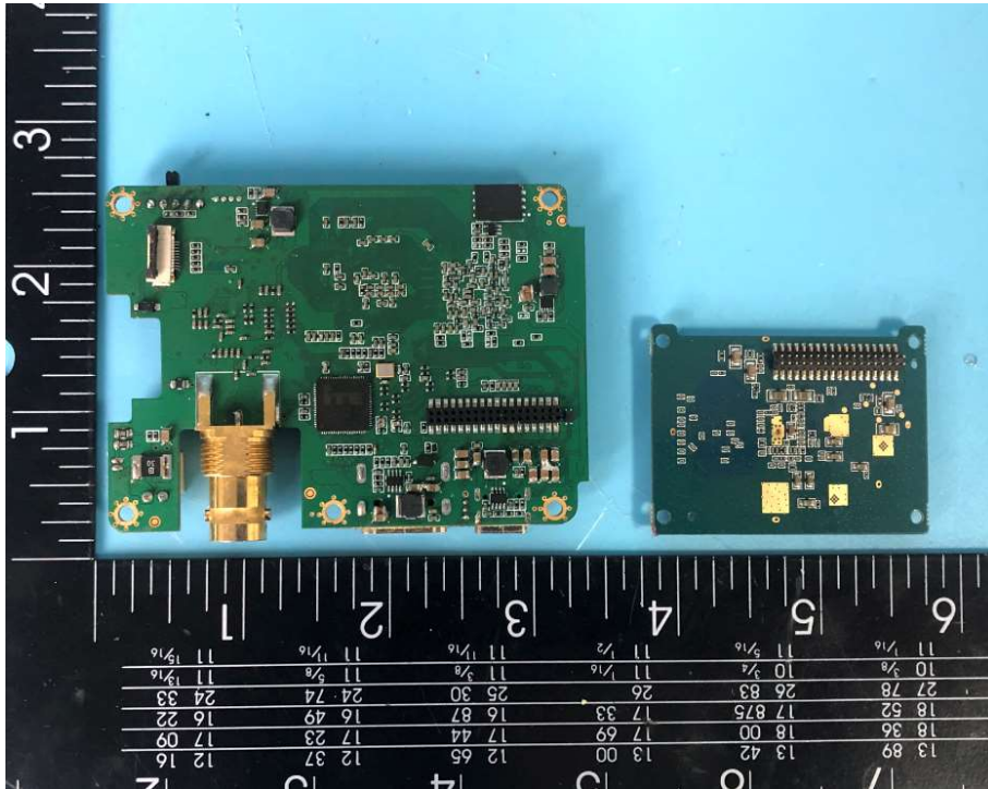
Photo 7(Receiver)
