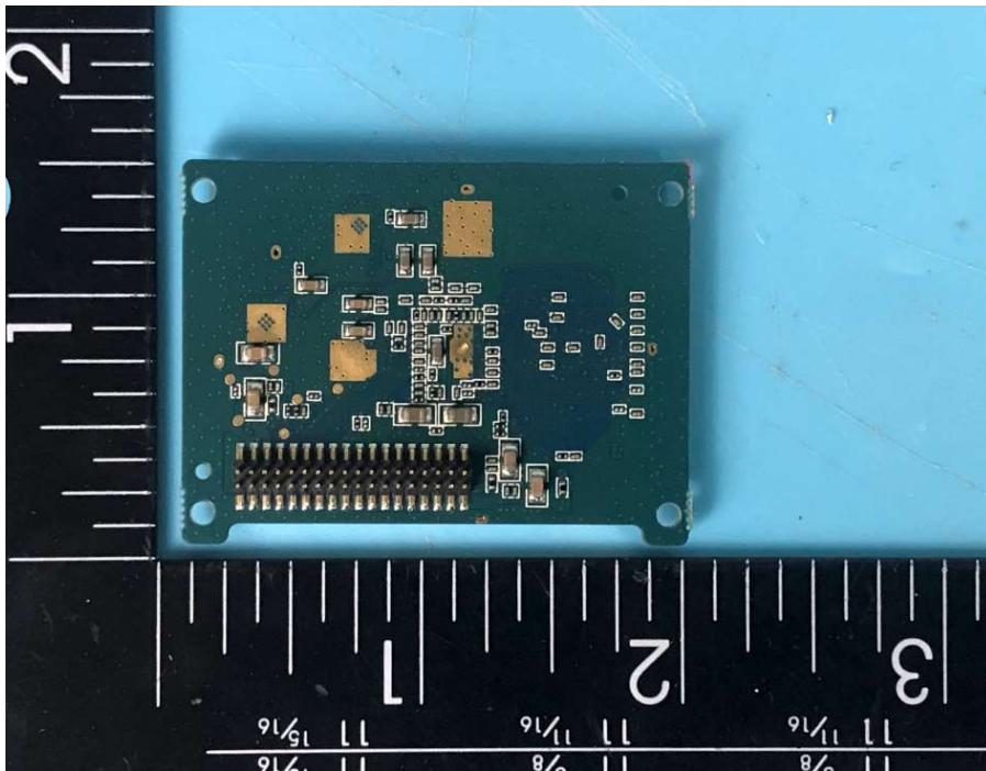
Photo 14(Receiver)
