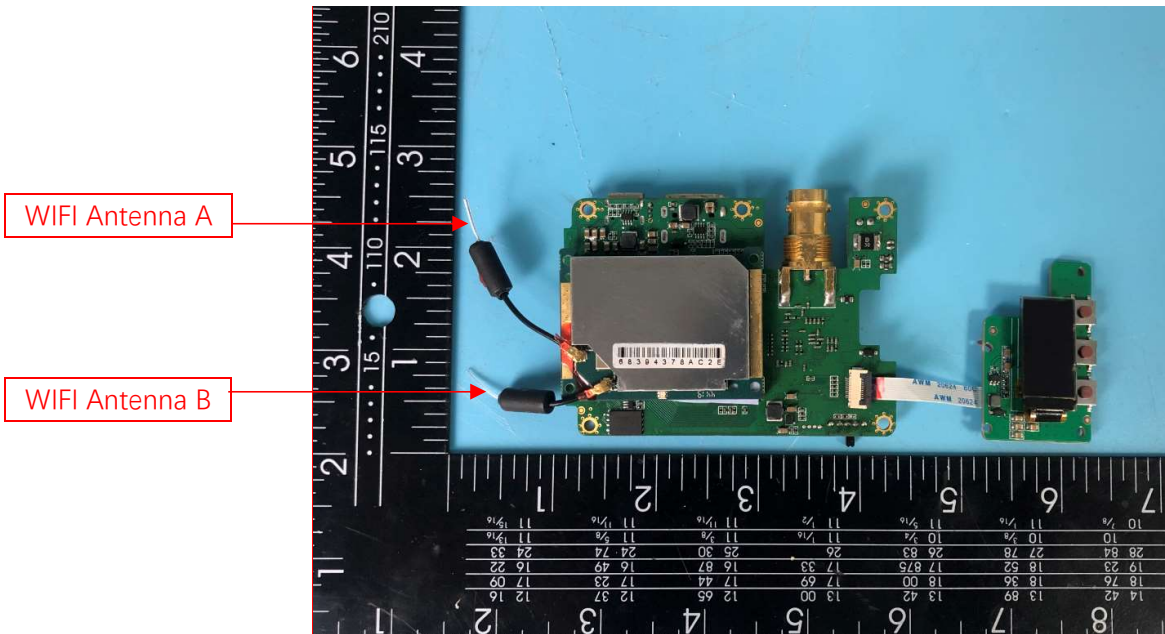
Photo 2(Receiver)
