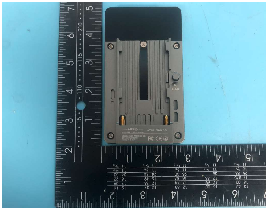
Photo 8(Receiver)
