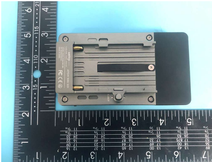
Photo 2(Receiver)
