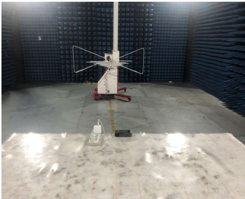
Transmitter Radiation Measurement below 1GHz
