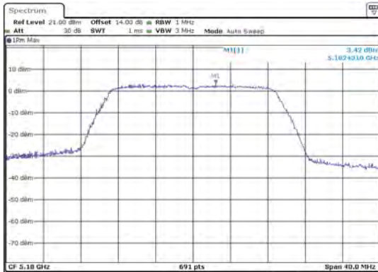
ANT 1(11N20)
