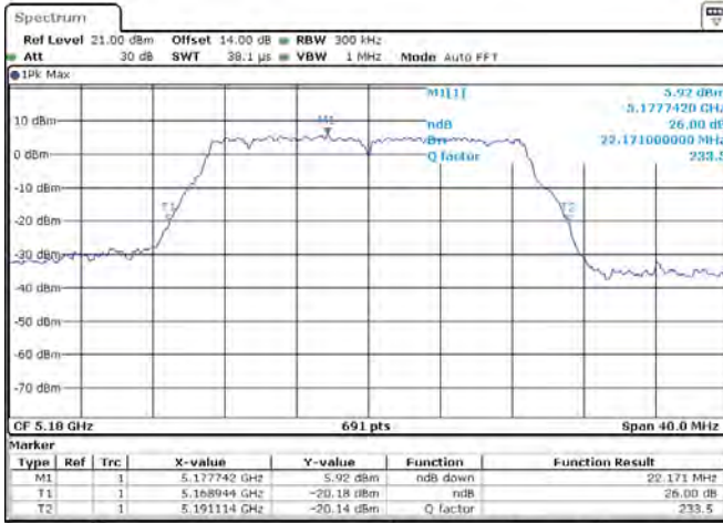
ANT 1(11N20)
