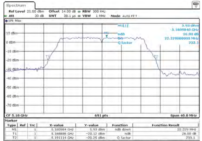
ANT 2(11N20)
