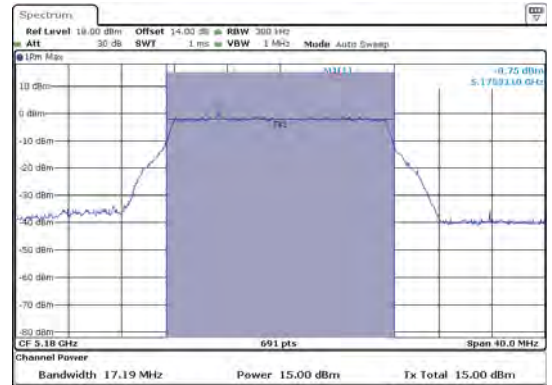
ANT 2(802.11A)
