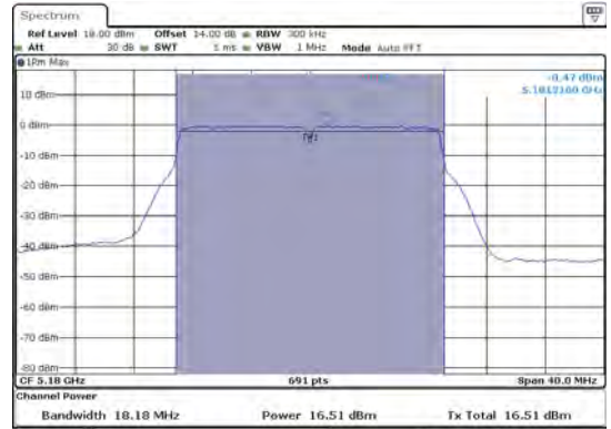
ANT 2(802.11 N20)
