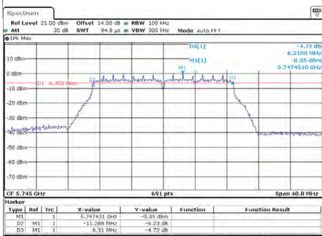
ANT 1(802.11N20)
