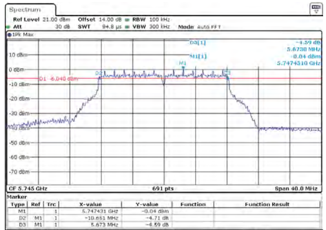
ANT 2(802.11A)
