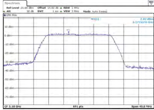
ANT 2(11N20)
