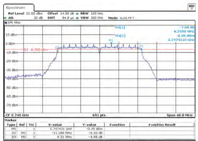
ANT 2(802.11N20)
