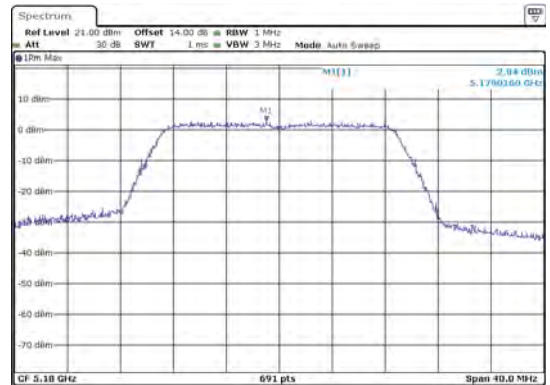
ANT 2(11N20)
