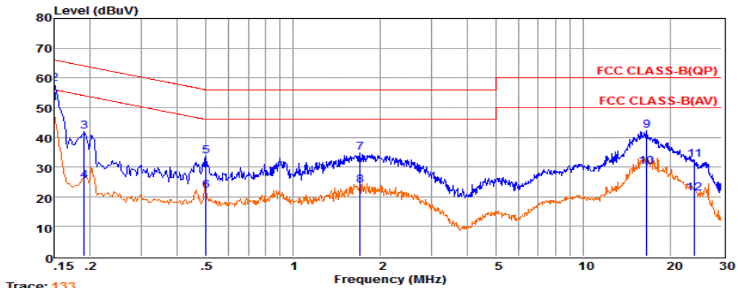
Trace: 133
