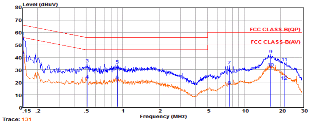
Trace: 131
