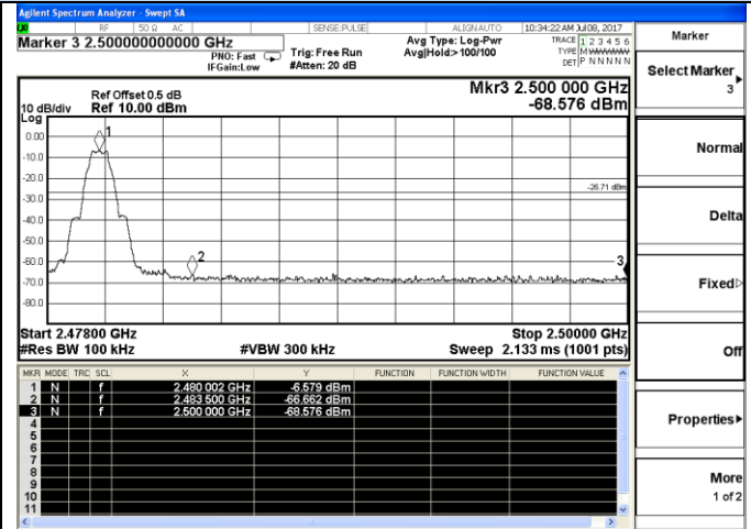
Channel 39 / 2480 MHz
