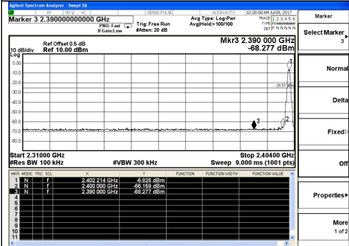
Channel 0 / 2402 MHz
