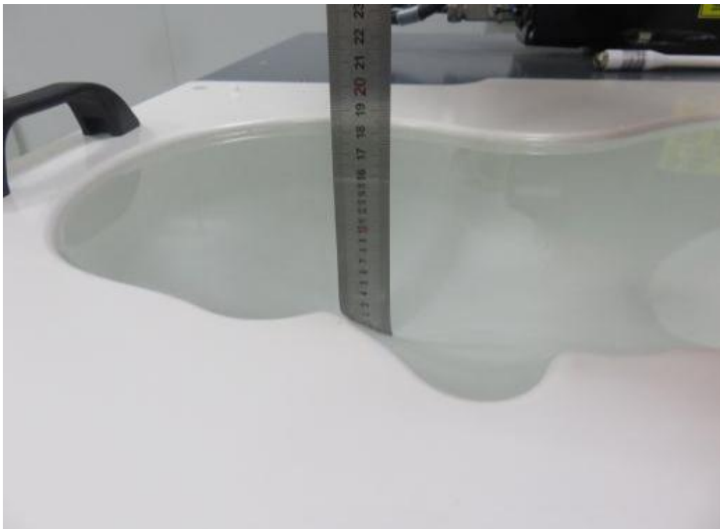
Photograph of the depth in the Head Phantom (5000-6000MHz, 15.3cm depth)
