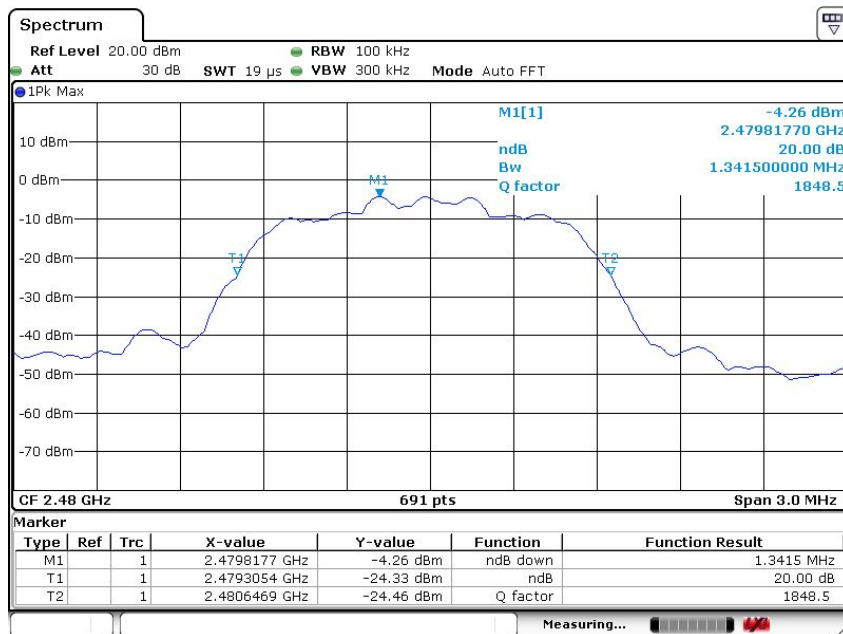
(Plot 4.4.2 C: Channel 78: 2480MHz @ 8DPSK)
