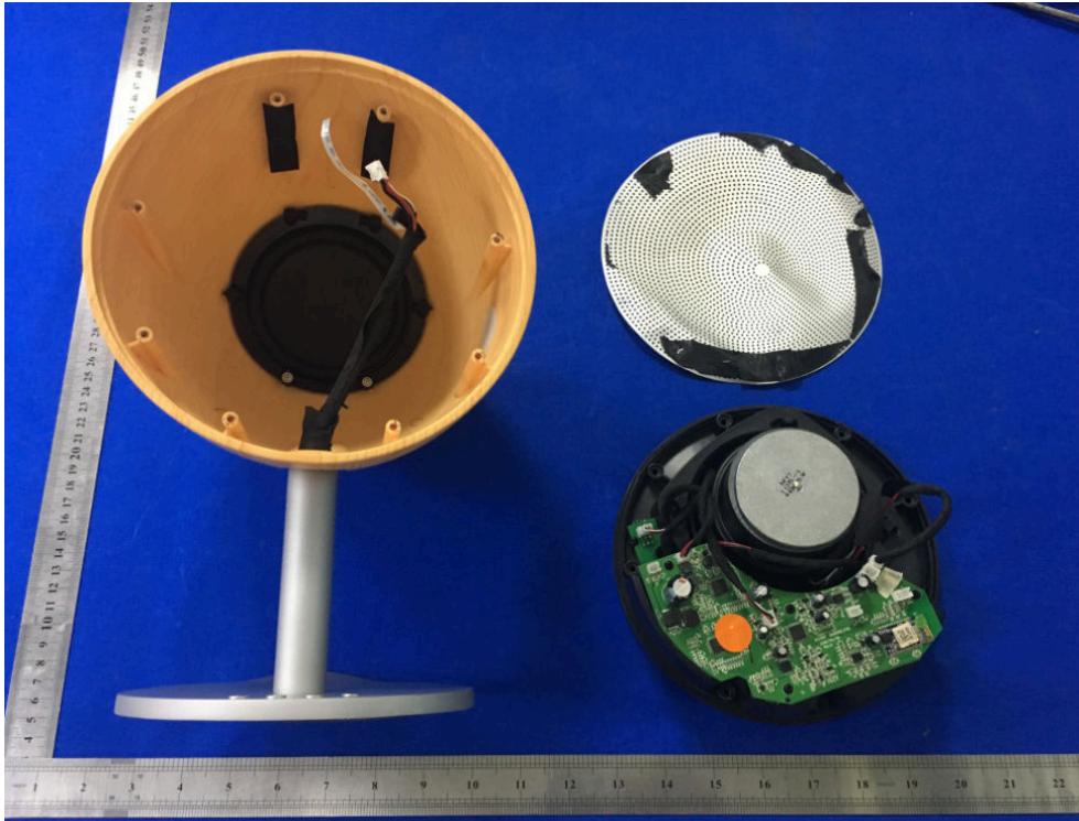
EUT –Top Open View
