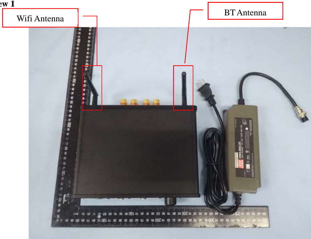
EUT View 1
