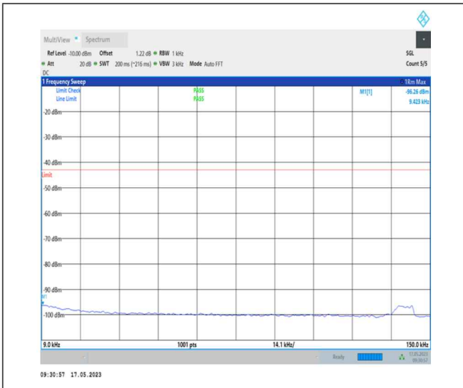
1-N78-3700-3800-PC1-30-100-H-1-DFT-PI2BPSK- Inner_1RB_Left-1@1-0.009-0.15-Ant0-0.01--96.26-- 43-PASS
