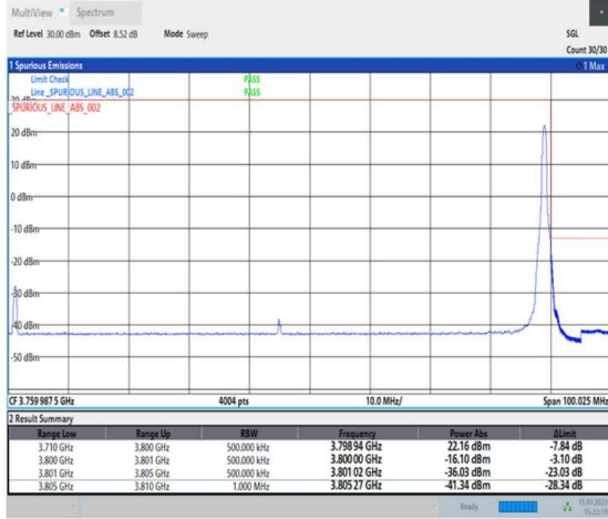
1-N78-3700-3800-PC1-30-90-H-2-DFT-PI2BPSK-Edge_1RB_Right-1@244-Ant0-1--PASS-see graph
