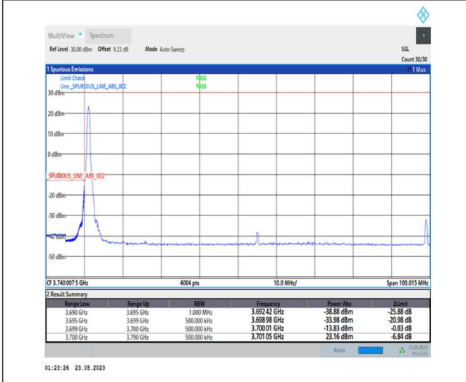
1-N78-3700-3800-PC1-30-90-L-4-CP-QPSK-Edge_1RB_Left-1@0-Ant0-1--PASS-see graph
