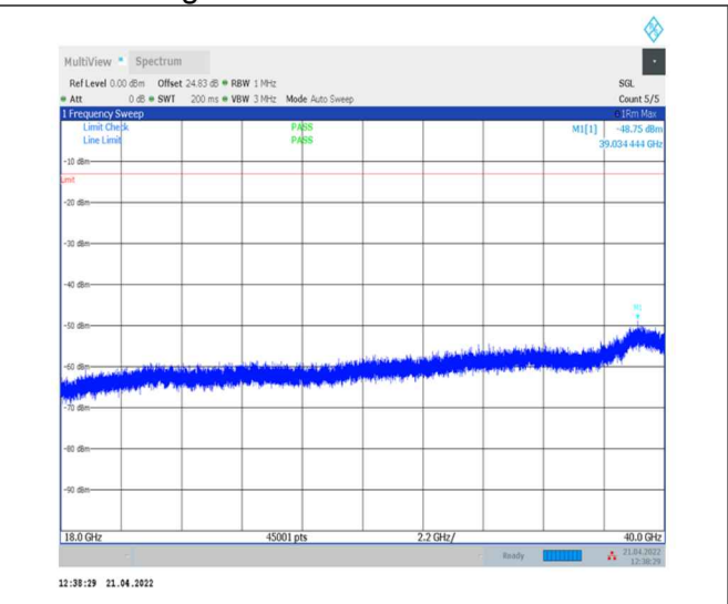
1-N78-3700-3800--30-100-L-1-DFT-PI2BPSK- Inner_1RB_Left-1@1-18000-40000-Ant0--48.75--13- PASS
