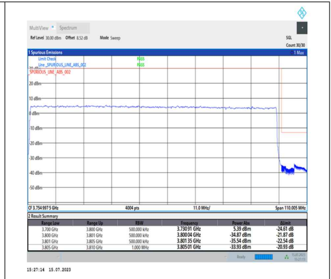
1-N78-3700-3800-PC1-30-100-H-3-DFT-PI2BPSK-Outer_Full-270@0-Ant0-1--PASS-see graph
