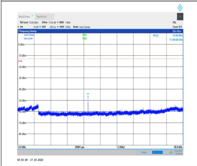
1-N78-3700-3800-PC1-30-100-M-1-DFT-PI2BPSK- Inner_1RB_Left-1@1-6000-18000-Ant0-11104.32-- 47.69--13-PASS
