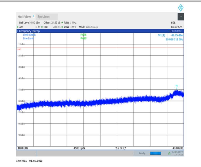
1-N78-3700-3800--30-100-M-1-DFT-PI2BPSK- Inner_1RB_Left-1@1-18000-40000-Ant0--49.75--13- PASS
