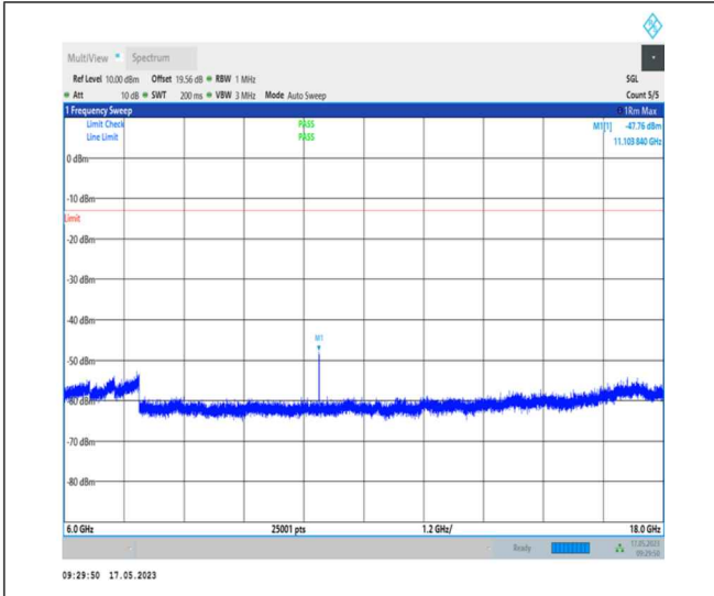
1-N78-3700-3800-PC1-30-100-L-1-DFT-PI2BPSK- Inner_1RB_Left-1@1-6000-18000-Ant0-11103.84-- 47.76--13-PASS
