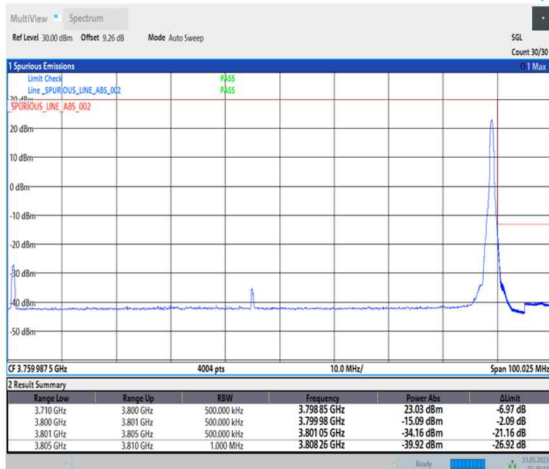
1-N78-3700-3800-PC1-30-90-H-5-CP-QPSK-Edge_1RB_Right-1@244-Ant0-1--PASS-see graph
