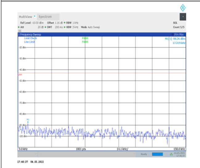
1-N78-3700-3800--30-100-M-1-DFT-PI2BPSK- Inner_1RB_Left-1@1-0.009-0.15-Ant0--88.26--43- PASS
