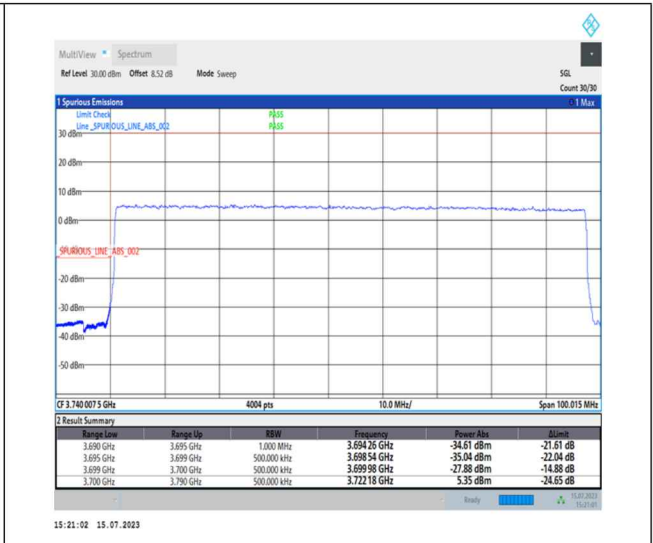
1-N78-3700-3800-PC1-30-90-L-3-DFT-PI2BPSK-Outer_Full-240@0-Ant0-1--PASS-see graph
