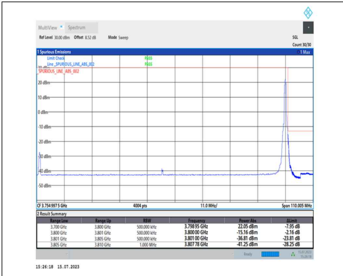
1-N78-3700-3800-PC1-30-100-H-2-DFT-PI2BPSK-Edge_1RB_Right-1@272-Ant0-1--PASS-see graph
