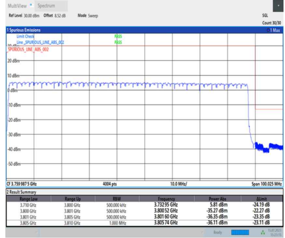
1-N78-3700-3800-PC1-30-90-H-3-DFT-PI2BPSK-Outer_Full-240@0-Ant0-1--PASS-see graph
