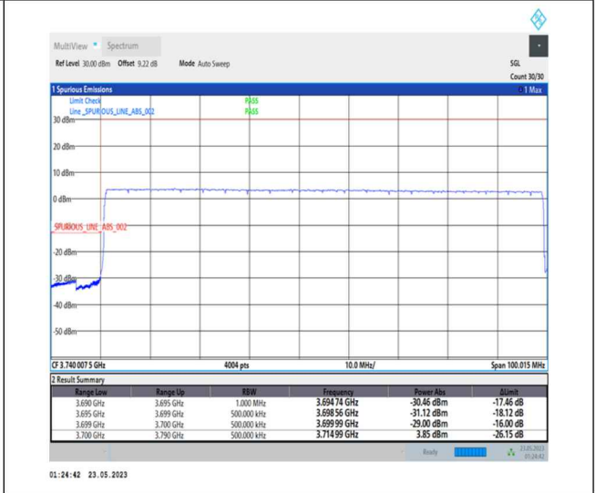
1-N78-3700-3800-PC1-30-90-L-6-CP-QPSK-Outer_Full-245@0-Ant0-1--PASS-see graph
