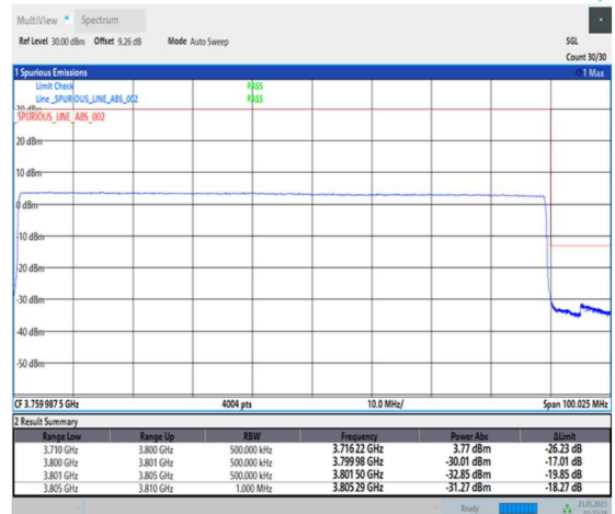
1-N78-3700-3800-PC1-30-90-H-6-CP-QPSK-Outer_Full-245@0-Ant0-1--PASS-see graph
