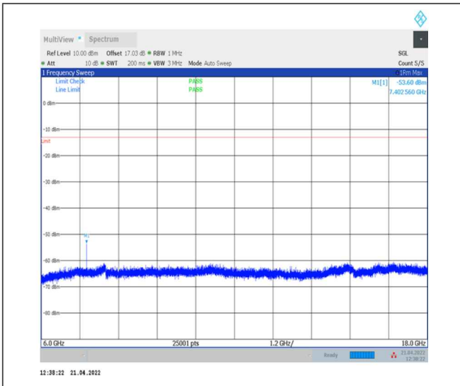
1-N78-3700-3800--30-100-L-1-DFT-PI2BPSK- Inner_1RB_Left-1@1-6000-18000-Ant0--53.60--13- PASS
