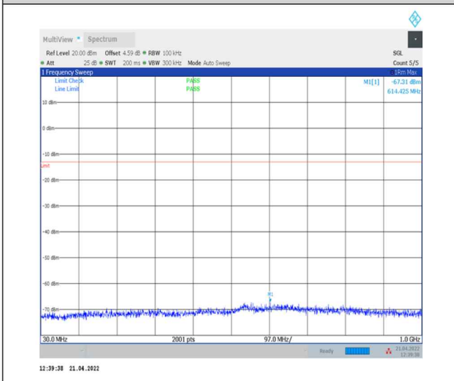
1-N78-3700-3800--30-100-H-1-DFT-PI2BPSK- Inner_1RB_Left-1@1-30-1000-Ant0--67.31--13- PASS
