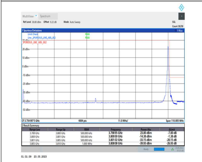
1-N78-3700-3800-PC1-30-100-H-5-CP-QPSK-Edge_1RB_Right-1@272-Ant0-1--PASS-see graph
