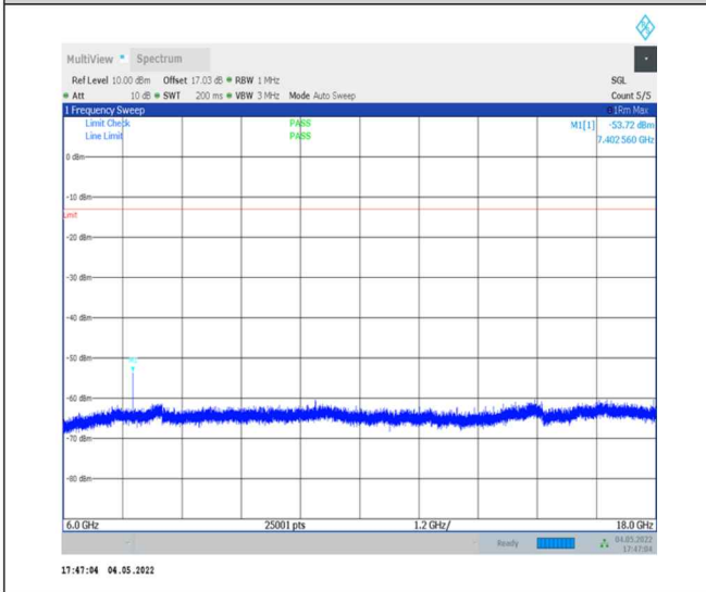
1-N78-3700-3800--30-100-M-1-DFT-PI2BPSK- Inner_1RB_Left-1@1-6000-18000-Ant0--53.72--13- PASS
