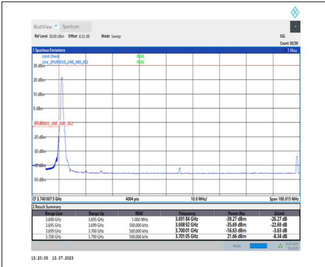
1-N78-3700-3800-PC1-30-90-L-1-DFT-PI2BPSK-Edge_1RB_Left-1@0-Ant0-1--PASS-see graph
