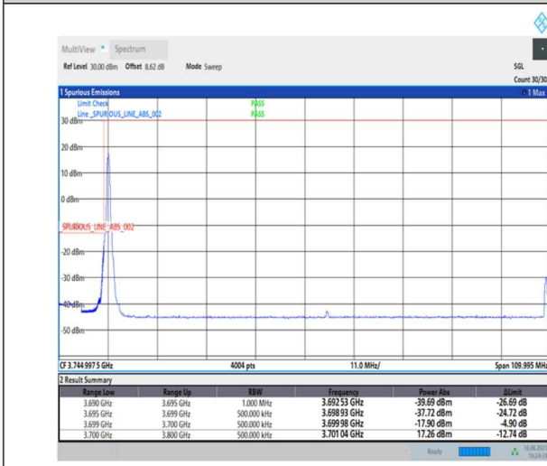
1-N78-3700-3800-PC1-30-100-L-1-DFT-PI2BPSK-Edge_1RB_Left-1@0-Ant0-1--PASS-see graph
