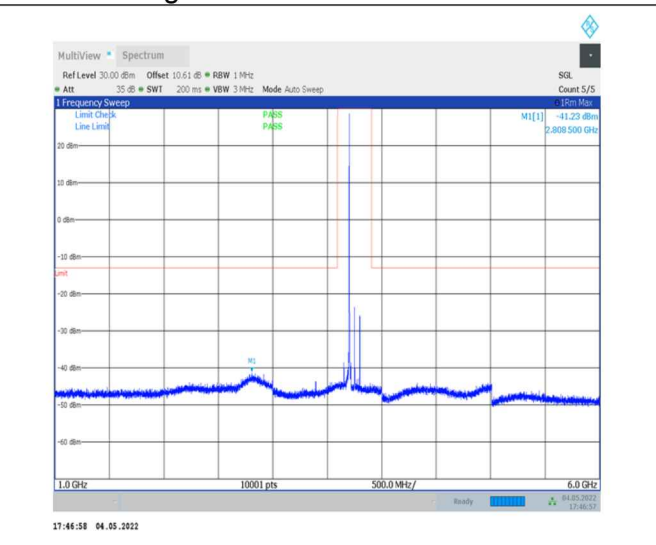
1-N78-3700-3800--30-100-M-1-DFT-PI2BPSK- Inner_1RB_Left-1@1-1000-6000-Ant0--41.23--13- PASS
