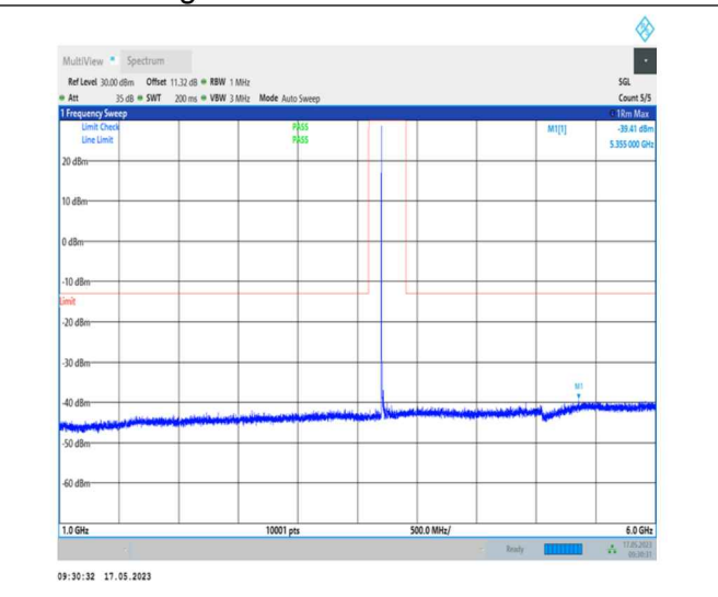
1-N78-3700-3800-PC1-30-100-M-1-DFT-PI2BPSK- Inner_1RB_Left-1@1-1000-6000-Ant0-5355.00-- 39.41--13-PASS
