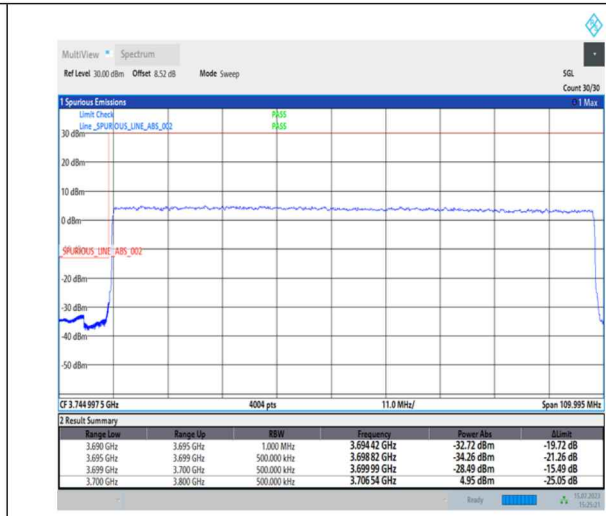
1-N78-3700-3800-PC1-30-100-L-3-DFT-PI2BPSK-Outer_Full-270@0-Ant0-1--PASS-see graph
