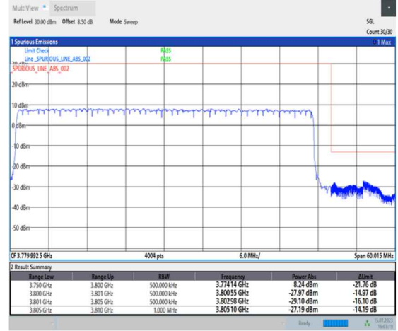
1-N78-3700-3800-PC1-30-50-H-3-DFT-PI2BPSK-Outer_Full-128@0-Ant0-1--PASS-see graph
