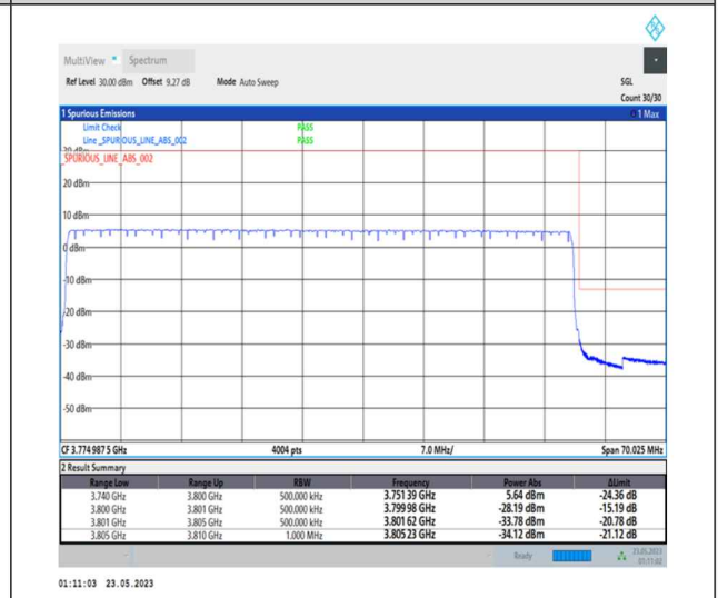
1-N78-3700-3800-PC1-30-60-H-6-CP-QPSK-Outer_Full-162@0-Ant0-1--PASS-see graph
