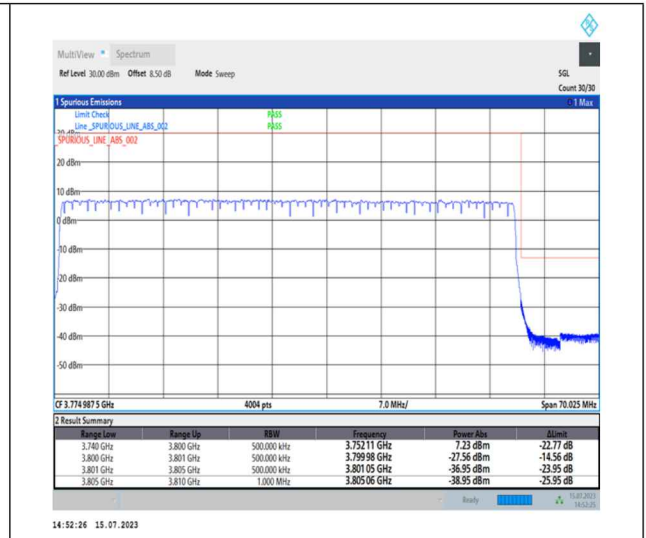
1-N78-3700-3800-PC1-30-60-H-3-DFT-PI2BPSK-Outer_Full-162@0-Ant0-1--PASS-see graph
