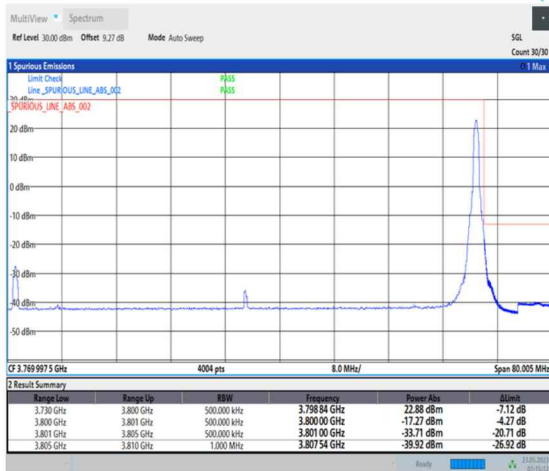
1-N78-3700-3800-PC1-30-70-H-5-CP-QPSK-Edge_1RB_Right-1@188-Ant0-1--PASS-see graph
