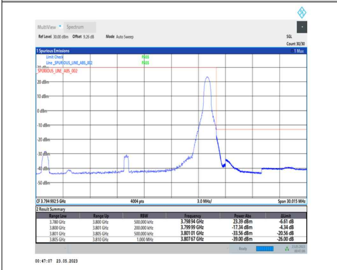
1-N78-3700-3800-PC1-30-20-H-5-CP-QPSK-Edge_1RB_Right-1@50-Ant0-1--PASS-see graph
