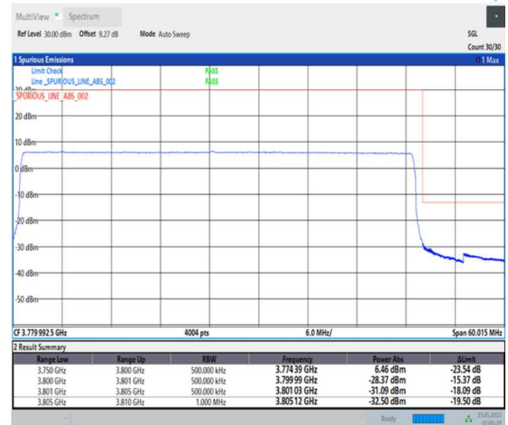
1-N78-3700-3800-PC1-30-50-H-6-CP-QPSK-Outer_Full-133@0-Ant0-1--PASS-see graph
