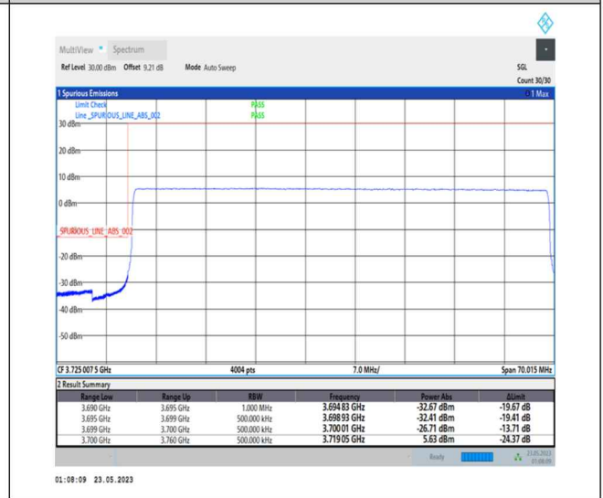
1-N78-3700-3800-PC1-30-60-L-6-CP-QPSK-Outer_Full-162@0-Ant0-1--PASS-see graph
