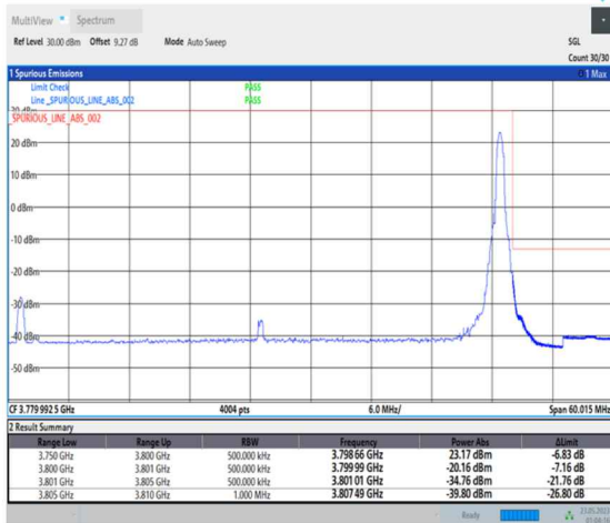
1-N78-3700-3800-PC1-30-50-H-5-CP-QPSK-Edge_1RB_Right-1@132-Ant0-1--PASS-see graph
