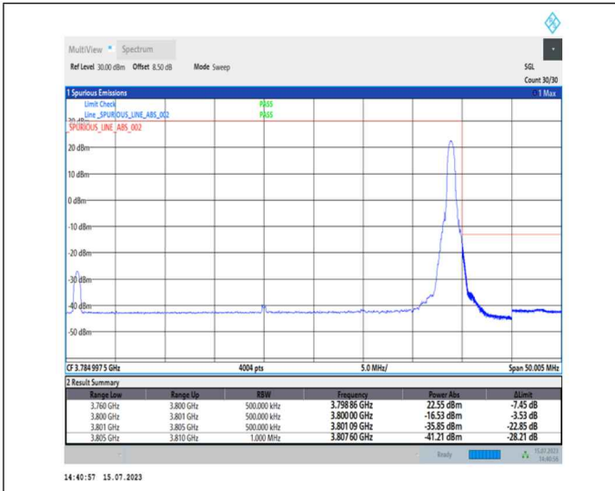
1-N78-3700-3800-PC1-30-40-H-2-DFT-PI2BPSK-Edge_1RB_Right-1@105-Ant0-1--PASS-see graph
