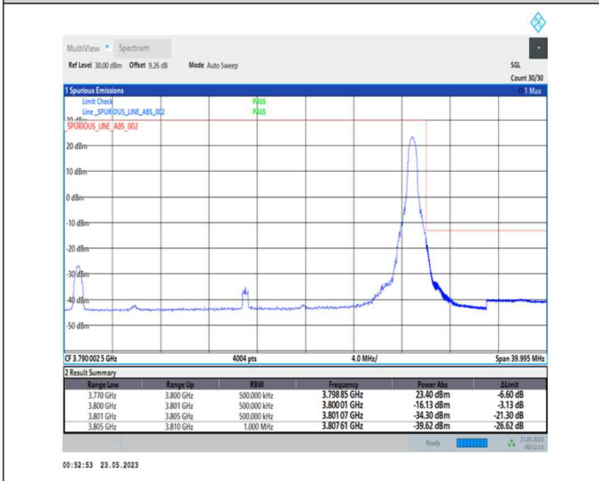
1-N78-3700-3800-PC1-30-30-H-5-CP-QPSK-Edge_1RB_Right-1@77-Ant0-1--PASS-see graph
