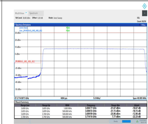
1-N78-3700-3800-PC1-30-40-L-3-DFT-PI2BPSK-Outer_Full-100@0-Ant0-1--PASS-see graph
