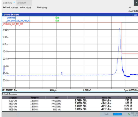
1-N78-3700-3800-PC1-30-70-H-2-DFT-PI2BPSK-Edge_1RB_Right-1@188-Ant0-1--PASS-see graph
