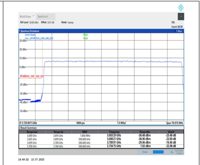
1-N78-3700-3800-PC1-30-60-L-3-DFT-PI2BPSK-Outer_Full-162@0-Ant0-1--PASS-see graph
