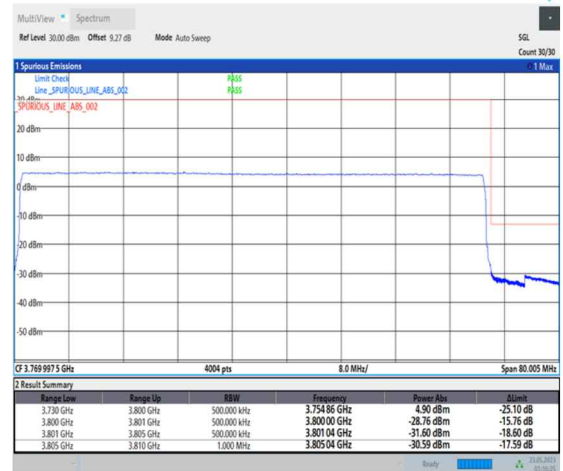
1-N78-3700-3800-PC1-30-70-H-6-CP-QPSK-Outer_Full-189@0-Ant0-1--PASS-see graph
