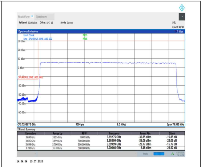
1-N78-3700-3800-PC1-30-70-L-3-DFT-PI2BPSK-Outer_Full-180@0-Ant0-1--PASS-see graph
