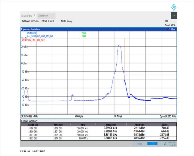
1-N78-3700-3800-PC1-30-20-H-2-DFT-PI2BPSK-Edge_1RB_Right-1@50-Ant0-1--PASS-see graph
