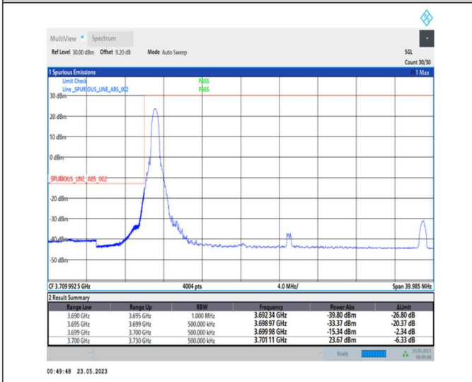
1-N78-3700-3800-PC1-30-30-L-4-CP-QPSK-Edge_1RB_Left-1@0-Ant0-1--PASS-see graph
