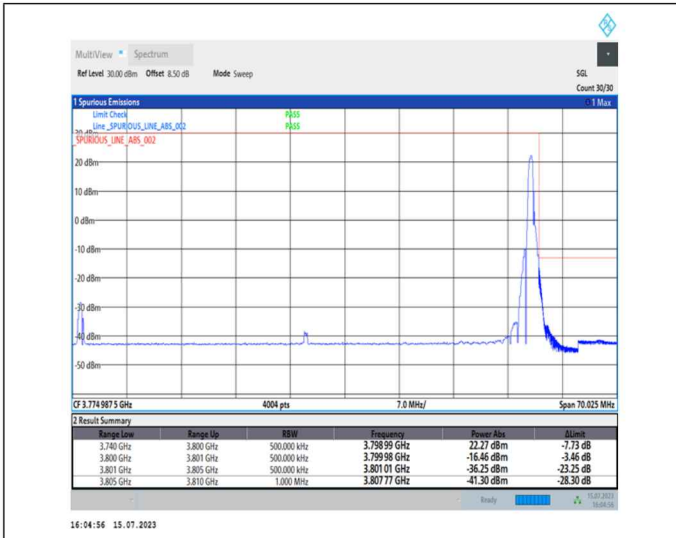
1-N78-3700-3800-PC1-30-60-H-2-DFT-PI2BPSK-Edge_1RB_Right-1@161-Ant0-1--PASS-see graph
