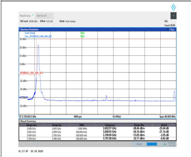
1-N78-3700-3800-PC1-30-80-L-4-CP-QPSK-Edge_1RB_Left-1@0-Ant0-1--PASS-see graph
