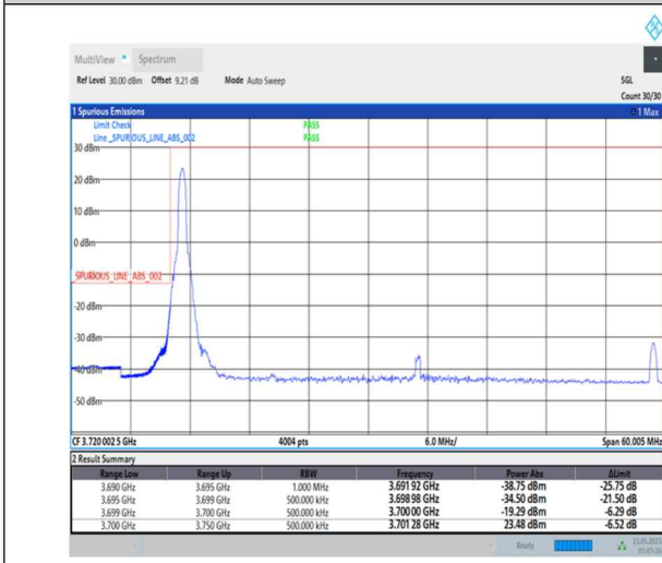
1-N78-3700-3800-PC1-30-50-L-1-DFT-PI2BPSK-Edge_1RB_Left-1@0-Ant0-1--PASS-see graph
