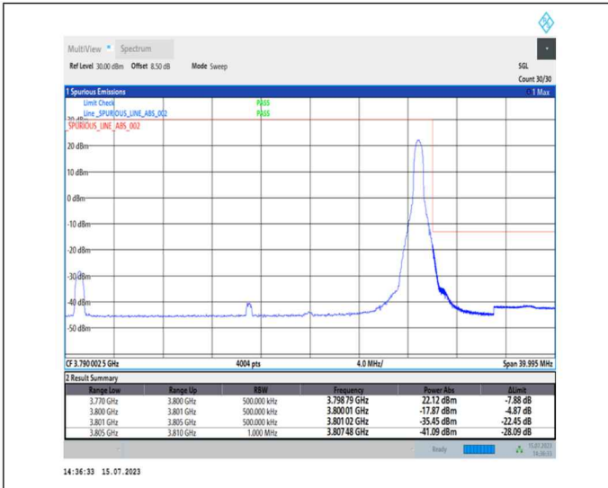
1-N78-3700-3800-PC1-30-30-H-2-DFT-PI2BPSK-Edge_1RB_Right-1@77-Ant0-1--PASS-see graph
