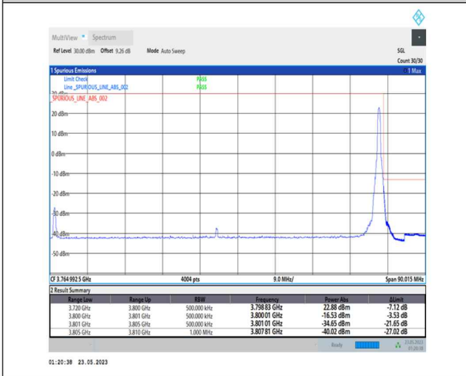
1-N78-3700-3800-PC1-30-80-H-5-CP-QPSK-Edge_1RB_Right-1@216-Ant0-1--PASS-see graph
