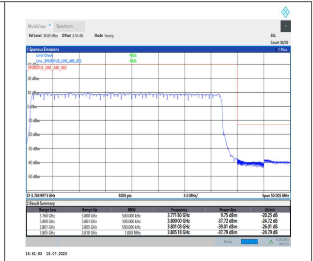
1-N78-3700-3800-PC1-30-40-H-3-DFT-PI2BPSK-Outer_Full-100@0-Ant0-1--PASS-see graph
