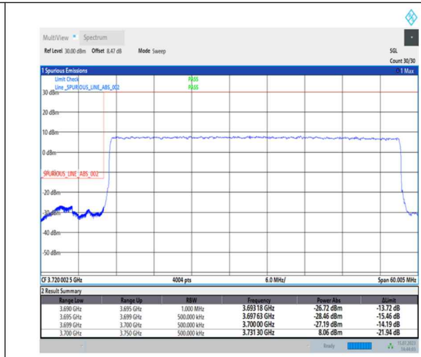
1-N78-3700-3800-PC1-30-50-L-3-DFT-PI2BPSK-Outer_Full-128@0-Ant0-1--PASS-see graph
