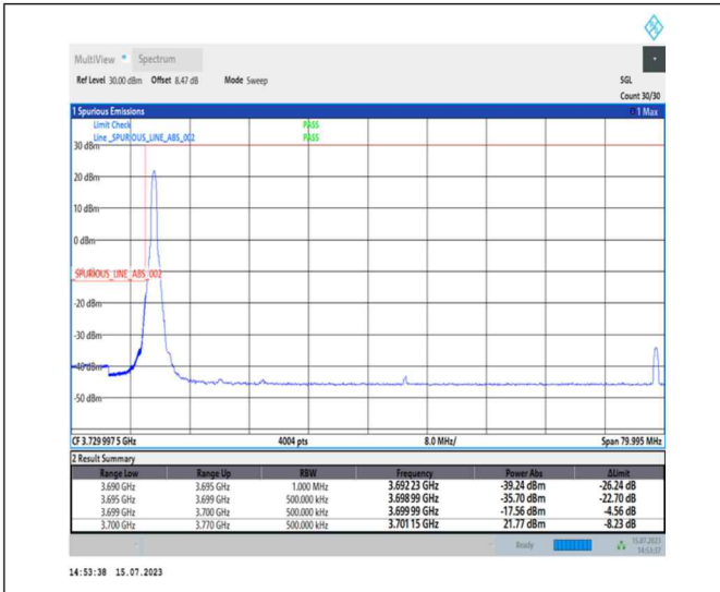
1-N78-3700-3800-PC1-30-70-L-1-DFT-PI2BPSK-Edge_1RB_Left-1@0-Ant0-1--PASS-see graph
