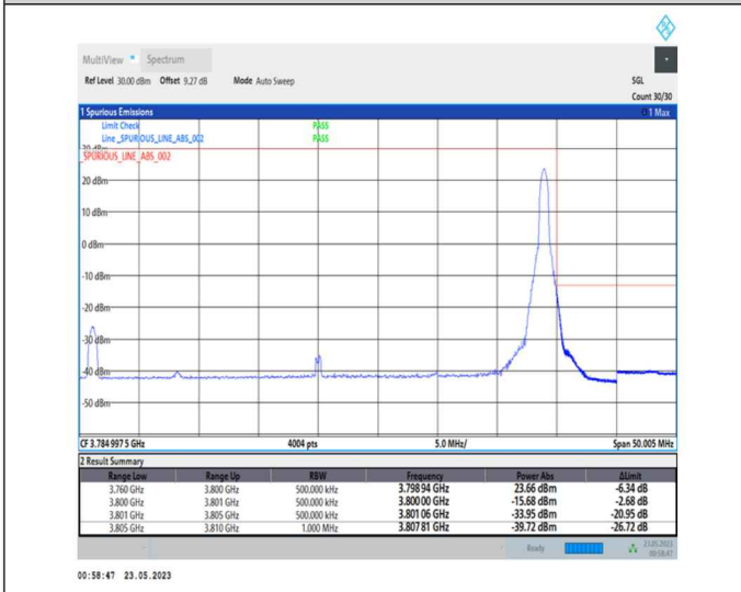
1-N78-3700-3800-PC1-30-40-H-5-CP-QPSK-Edge_1RB_Right-1@105-Ant0-1--PASS-see graph
