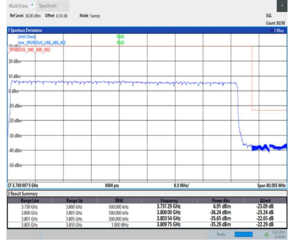
1-N78-3700-3800-PC1-30-70-H-3-DFT-PI2BPSK-Outer_Full-180@0-Ant0-1--PASS-see graph
