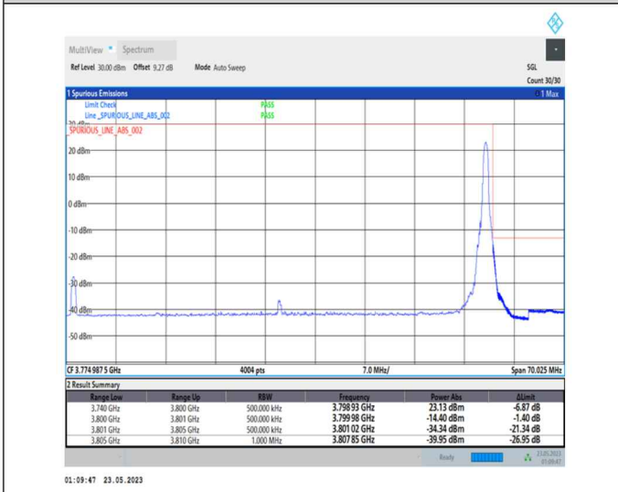
1-N78-3700-3800-PC1-30-60-H-5-CP-QPSK-Edge_1RB_Right-1@161-Ant0-1--PASS-see graph
