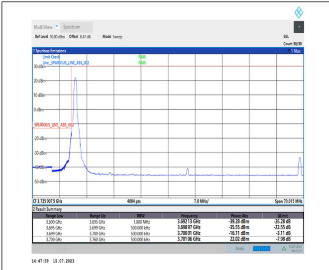
1-N78-3700-3800-PC1-30-60-L-1-DFT-PI2BPSK-Edge_1RB_Left-1@0-Ant0-1--PASS-see graph
