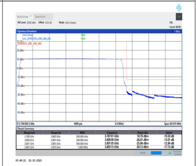
1-N78-3700-3800-PC1-30-20-H-6-CP-QPSK-Outer_Full-51@0-Ant0-1--PASS-see graph
