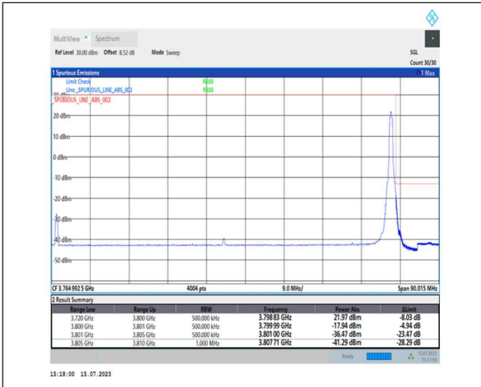
1-N78-3700-3800-PC1-30-80-H-2-DFT-PI2BPSK-Edge_1RB_Right-1@216-Ant0-1--PASS-see graph
