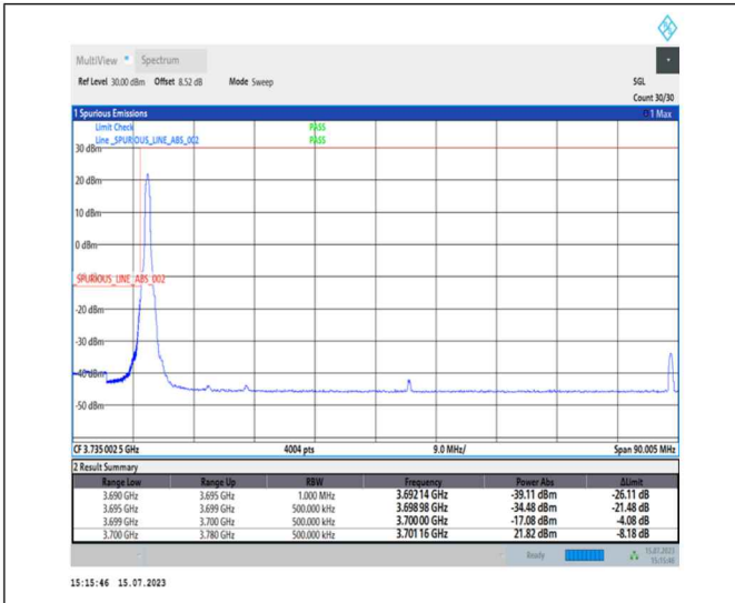
1-N78-3700-3800-PC1-30-80-L-1-DFT-PI2BPSK-Edge_1RB_Left-1@0-Ant0-1--PASS-see graph
