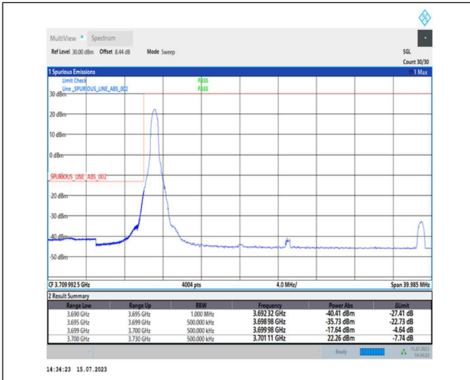
1-N78-3700-3800-PC1-30-30-L-1-DFT-PI2BPSK-Edge_1RB_Left-1@0-Ant0-1--PASS-see graph
