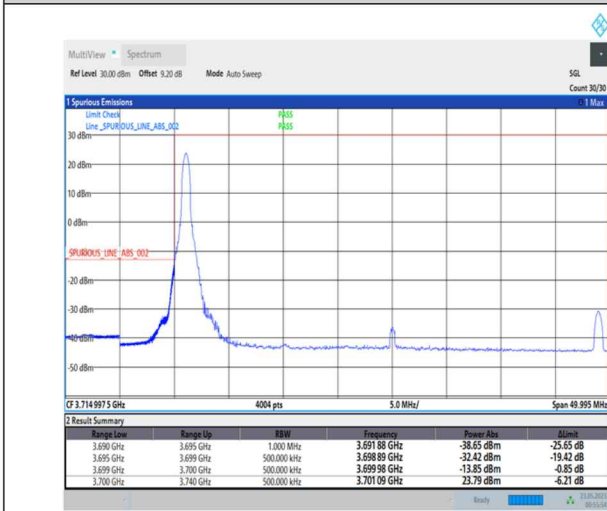
1-N78-3700-3800-PC1-30-40-L-1-DFT-PI2BPSK-Edge_1RB_Left-1@0-Ant0-1--PASS-see graph
