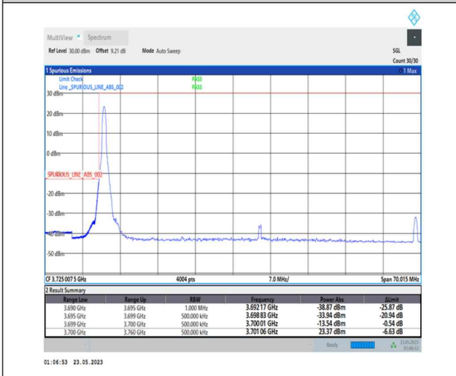
1-N78-3700-3800-PC1-30-60-L-4-CP-QPSK-Edge_1RB_Left-1@0-Ant0-1--PASS-see graph
