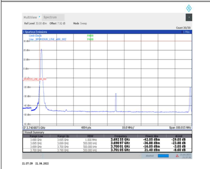
1-N78-3700-3800--30-90-L-4-CP-QPSK-Edge_1RB_Left-1@0-Ant0-PASS-see graph
