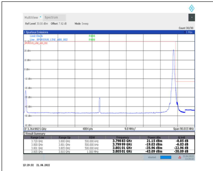
1-N78-3700-3800-30-80-H-2-DFT-PI2BPSK-Edge_1RB_Right-1@216-Ant0-PASS-see graph
