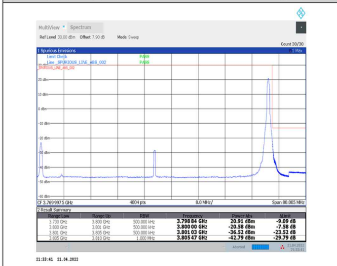
1-N78-3700-3800-30-70-H-5-CP-QPSK-Edge_1RB_Right-1@188-Ant0-PASS-see graph
