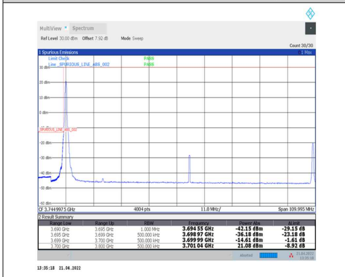
1-N78-3700-3800--30-100-L-4-CP-QPSK-Edge_1RB_Left-1@0-Ant0-PASS-see graph
