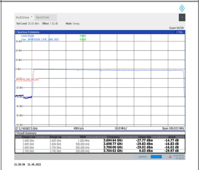
1-N78-3700-3800--30-90-L-6-CP-QPSK-Outer_Full-245@0-Ant0-PASS-see graph
