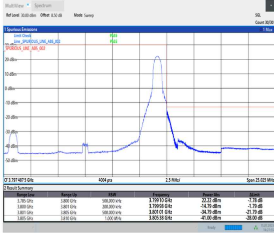
1-N78-3700-3800-PC1-30-15-H-2-DFT-PI2BPSK-Edge_1RB_Right-1@37-Ant0-1--PASS-see graph
