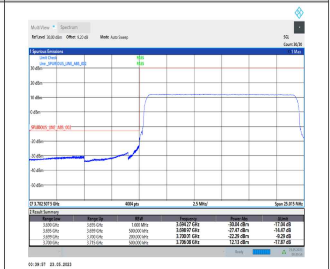
1-N78-3700-3800-PC1-30-15-L-6-CP-QPSK-Outer_Full-38@0-Ant0-1--PASS-see graph
