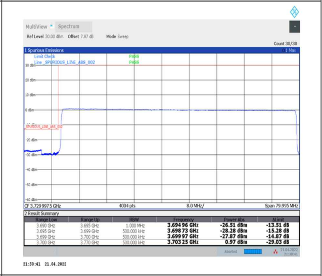
1-N78-3700-3800--30-70-L-6-CP-QPSK-Outer_Full-189@0-Ant0-PASS-see graph
