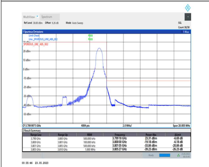
1-N78-3700-3800-PC1-30-10-H-5-CP-QPSK-Edge_1RB_Right-1@23-Ant0-1--PASS-see graph
