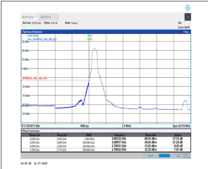
1-N78-3700-3800-PC1-30-15-L-1-DFT-PI2BPSK-Edge_1RB_Left-1@0-Ant0-1--PASS-see graph
