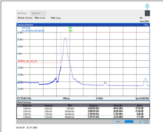
1-N78-3700-3800-PC1-30-20-L-1-DFT-PI2BPSK-Edge_1RB_Left-1@0-Ant0-1--PASS-see graph
