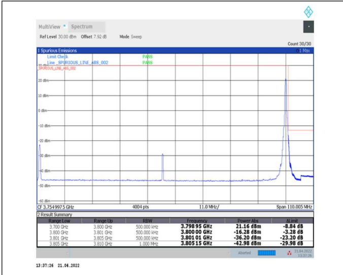
1-N78-3700-3800--30-100-H-2-DFT-PI2BPSK-Edge_1RB_Right-1@272-Ant0-PASS-see graph
