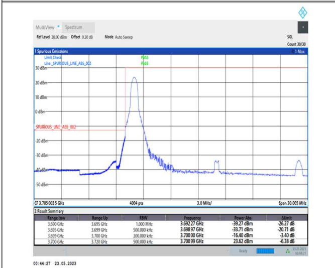
1-N78-3700-3800-PC1-30-20-L-4-CP-QPSK-Edge_1RB_Left-1@0-Ant0-1--PASS-see graph
