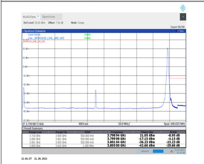
1-N78-3700-3800--30-90-H-5-CP-QPSK-Edge_1RB_Right-1@244-Ant0-PASS-see graph
