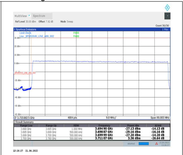
1-N78-3700-3800--30-80-L-3-DFT-PI2BPSK-Outer_Full-216@0-Ant0-PASS-see graph
