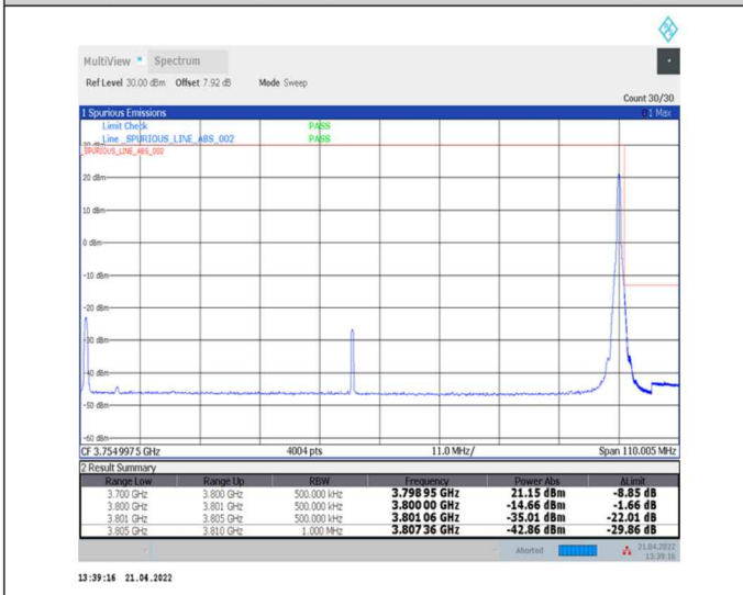
1-N78-3700-3800--30-100-H-5-CP-QPSK-Edge_1RB_Right-1@272-Ant0-PASS-see graph
