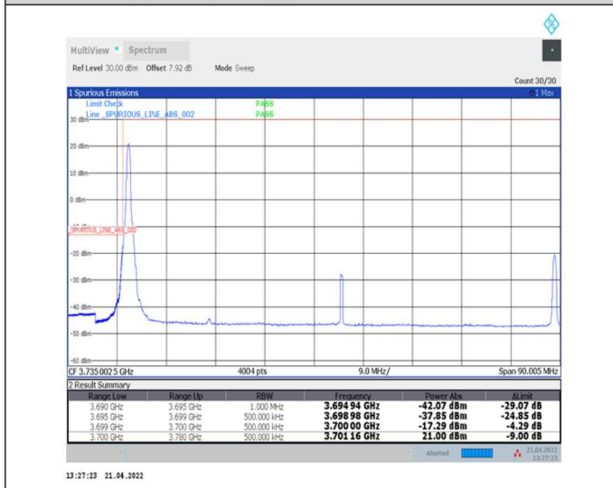
1-N78-3700-3800--30-80-L-4-CP-QPSK-Edge_1RB_Left-1@0-Ant0-PASS-see graph
