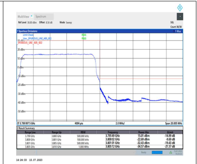
1-N78-3700-3800-PC1-30-10-H-3-DFT-PI2BPSK-Outer_Full-24@0-Ant0-1--PASS-see graph
