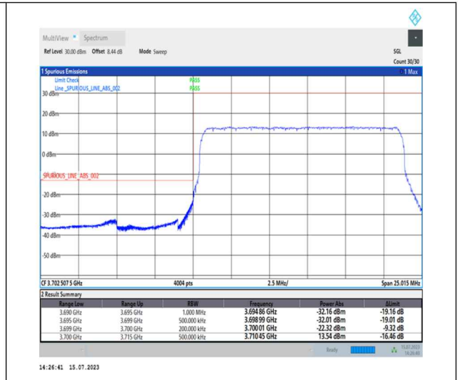
1-N78-3700-3800-PC1-30-15-L-3-DFT-PI2BPSK-Outer_Full-36@0-Ant0-1--PASS-see graph
