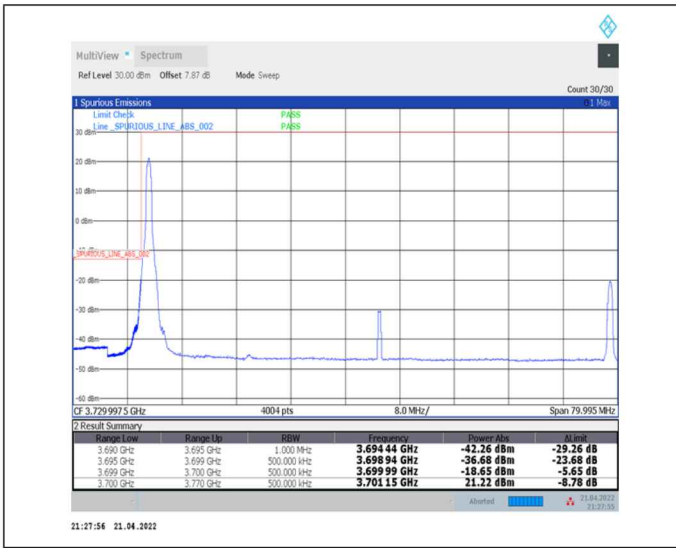
1-N78-3700-3800--30-70-L-1-DFT-PI2BPSK-Edge_1RB_Left-1@0-Ant0-PASS-see graph
