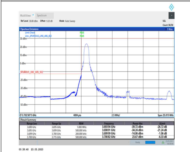
1-N78-3700-3800-PC1-30-15-L-4-CP-QPSK-Edge_1RB_Left-1@0-Ant0-1--PASS-see graph
