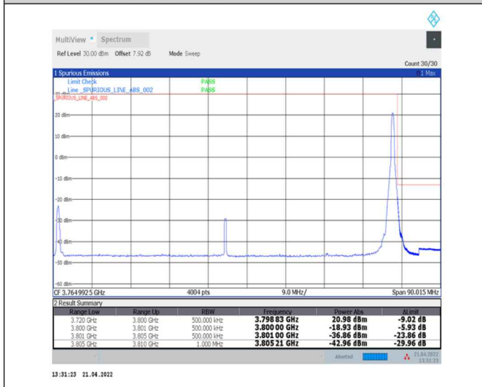
1-N78-3700-3800-30-80-H-5-CP-QPSK-Edge_1RB_Right-1@216-Ant0-PASS-see graph
