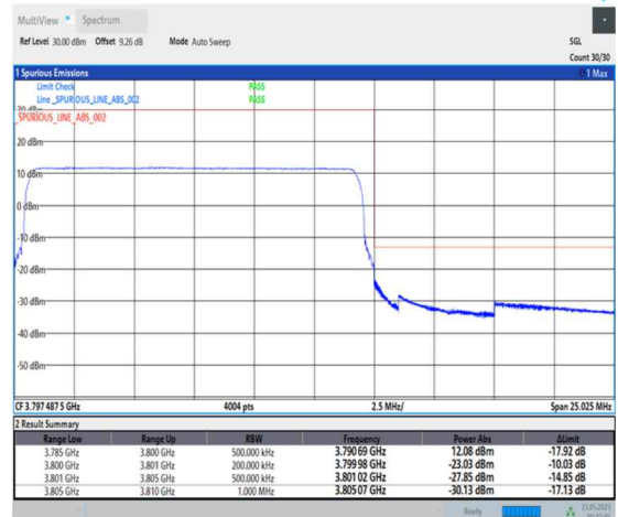
1-N78-3700-3800-PC1-30-15-H-6-CP-QPSK-Outer_Full-38@0-Ant0-1--PASS-see graph
