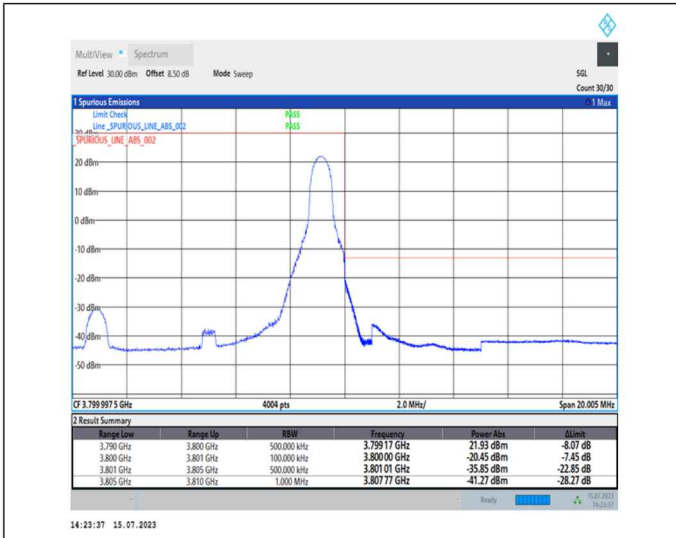
1-N78-3700-3800-PC1-30-10-H-2-DFT-PI2BPSK-Edge_1RB_Right-1@23-Ant0-1--PASS-see graph
