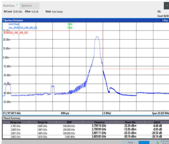
1-N78-3700-3800-PC1-30-15-H-5-CP-QPSK-Edge_1RB_Right-1@37-Ant0-1--PASS-see graph
