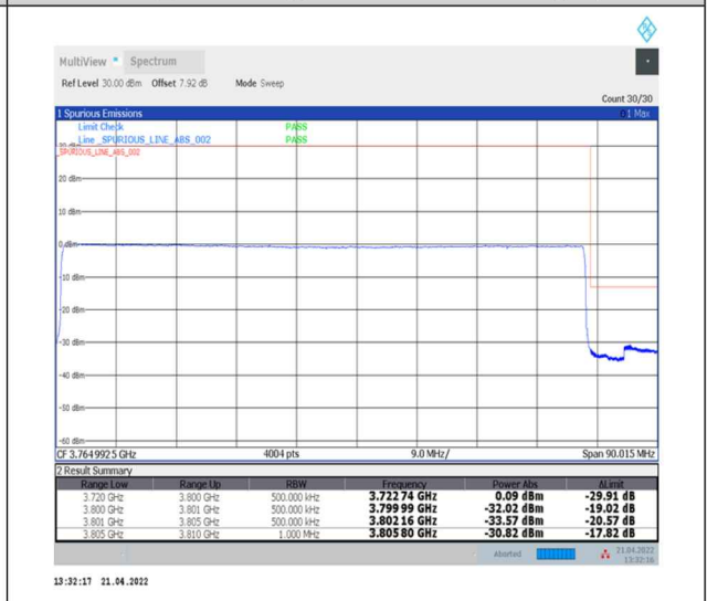
1-N78-3700-3800-30-80-H-6-CP-QPSK-Outer_Full-217@0-Ant0-PASS-see graph
