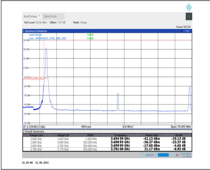
1-N78-3700-3800--30-70-L-4-CP-QPSK-Edge_1RB_Left-1@0-Ant0-PASS-see graph
