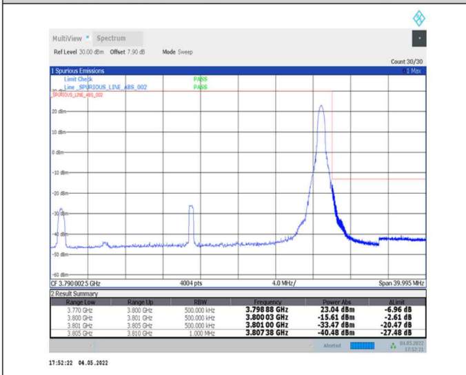
1-N78-3700-3800-30-30-H-5-CP-QPSK-Edge_1RB_Right-1@77-Ant0-PASS-see graph
