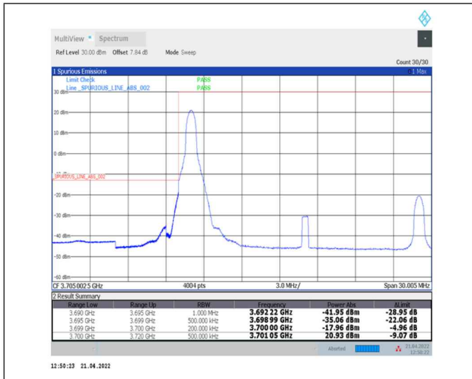
1-N78-3700-3800--30-20-L-1-DFT-PI2BPSK-Edge_1RB_Left-1@0-Ant0-PASS-see graph
