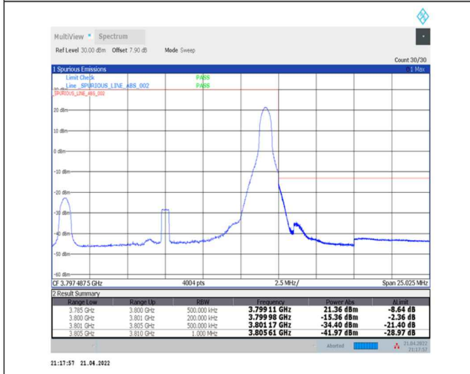
1-N78-3700-3800-30-15-H-5-CP-QPSK-Edge_1RB_Right-1@37-Ant0-PASS-see graph
