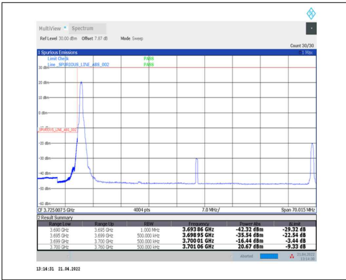
1-N78-3700-3800--30-60-L-1-DFT-PI2BPSK-Edge_1RB_Left-1@0-Ant0-PASS-see graph
