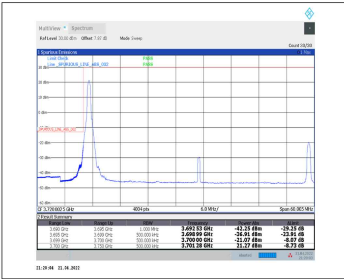
1-N78-3700-3800--30-50-L-1-DFT-PI2BPSK-Edge_1RB_Left-1@0-Ant0-PASS-see graph
