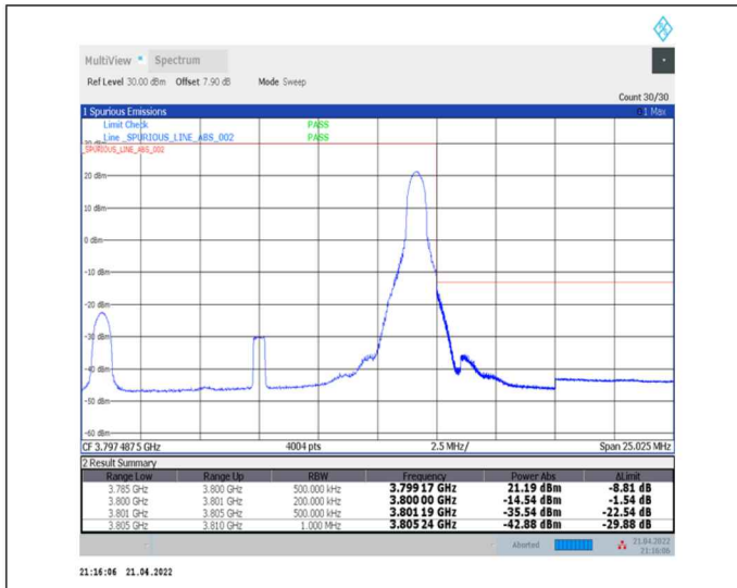
1-N78-3700-3800-30-15-H-2-DFT-PI2BPSK-Edge_1RB_Right-1@37-Ant0-PASS-see graph
