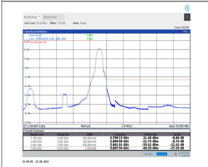
1-N78-3700-3800-30-10-H-5-CP-QPSK-Edge_1RB_Right-1@23-Ant0-PASS-see graph
