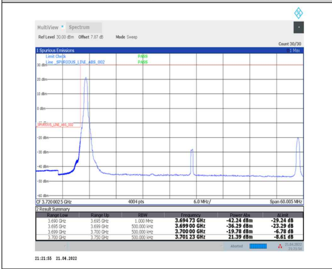
1-N78-3700-3800--30-50-L-4-CP-QPSK-Edge_1RB_Left-1@0-Ant0-PASS-see graph
