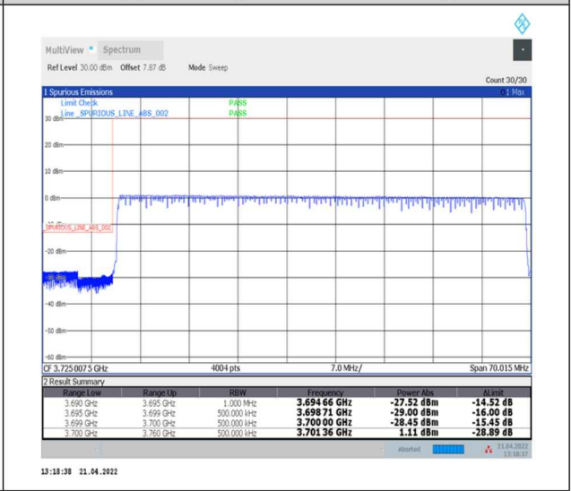
1-N78-3700-3800--30-60-L-6-CP-QPSK-Outer_Full-162@0-Ant0-PASS-see graph
