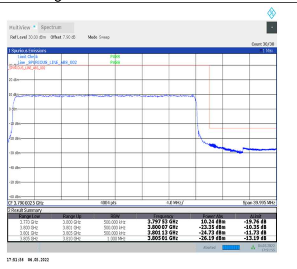
1-N78-3700-3800-30-30-H-3-DFT-PI2BPSK-Outer_Full-75@0-Ant0-PASS-see graph
