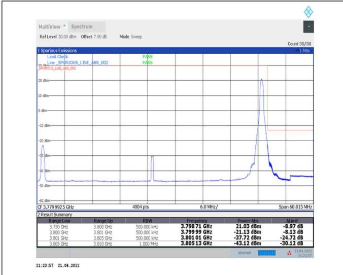
1-N78-3700-3800-30-50-H-2-DFT-PI2BPSK-Edge_1RB_Right-1@132-Ant0-PASS-see graph
