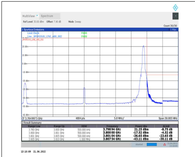
1-N78-3700-3800-30-40-H-2-DFT-PI2BPSK-Edge_1RB_Right-1@105-Ant0-PASS-see graph
