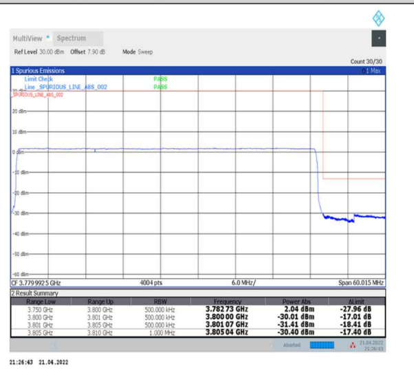
1-N78-3700-3800-30-50-H-6-CP-QPSK-Outer_Full-133@0-Ant0-PASS-see graph
