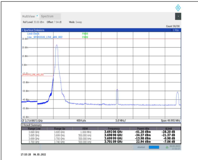
1-N78-3700-3800--30-40-L-1-DFT-PI2BPSK-Edge_1RB_Left-1@0-Ant0-PASS-see graph
