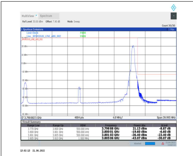
1-N78-3700-3800-30-30-H-2-DFT-PI2BPSK-Edge_1RB_Right-1@77-Ant0-PASS-see graph
