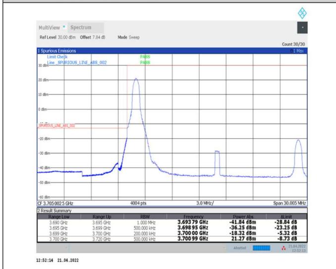
1-N78-3700-3800--30-20-L-4-CP-QPSK-Edge_1RB_Left-1@0-Ant0-PASS-see graph
