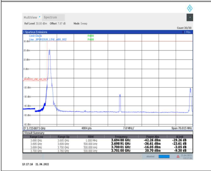
1-N78-3700-3800--30-60-L-4-CP-QPSK-Edge_1RB_Left-1@0-Ant0-PASS-see graph
