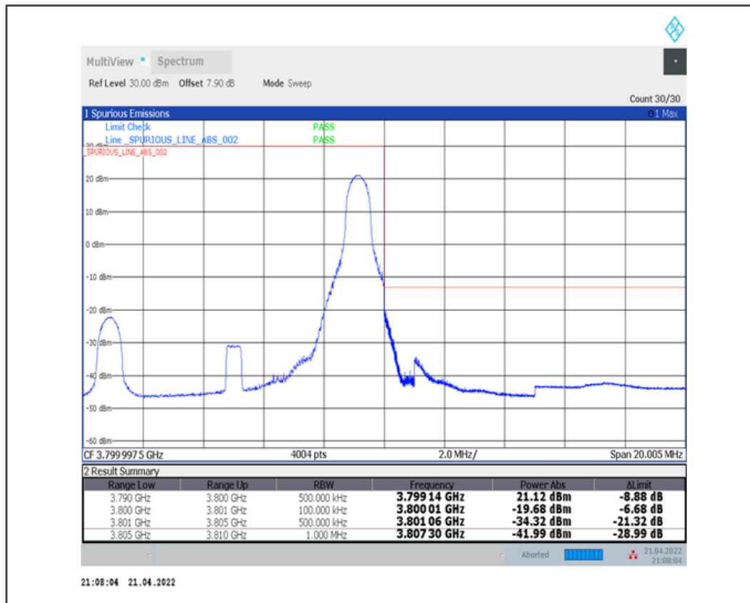
1-N78-3700-3800-30-10-H-2-DFT-PI2BPSK-Edge_1RB_Right-1@23-Ant0-PASS-see graph
