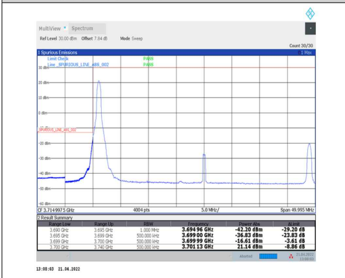
1-N78-3700-3800--30-40-L-4-CP-QPSK-Edge_1RB_Left-1@0-Ant0-PASS-see graph
