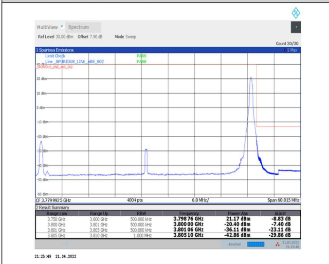
1-N78-3700-3800-30-50-H-5-CP-QPSK-Edge_1RB_Right-1@132-Ant0-PASS-see graph
