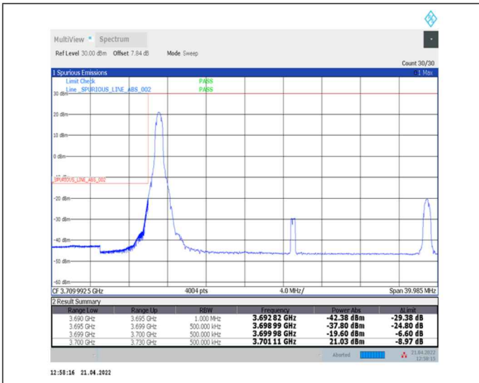
1-N78-3700-3800--30-30-L-1-DFT-PI2BPSK-Edge_1RB_Left-1@0-Ant0-PASS-see graph
