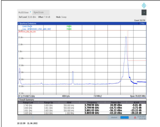
1-N78-3700-3800-30-60-H-5-CP-QPSK-Edge_1RB_Right-1@161-Ant0-PASS-see graph
