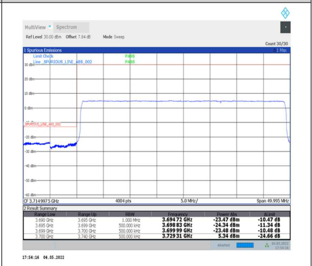
1-N78-3700-3800--30-40-L-6-CP-QPSK-Outer_Full-106@0-Ant0-PASS-see graph
