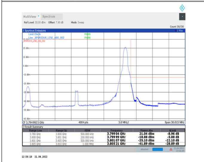
1-N78-3700-3800-30-20-H-5-CP-QPSK-Edge_1RB_Right-1@50-Ant0-PASS-see graph
