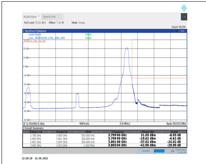
1-N78-3700-3800-30-20-H-2-DFT-PI2BPSK-Edge_1RB_Right-1@50-Ant0-PASS-see graph
