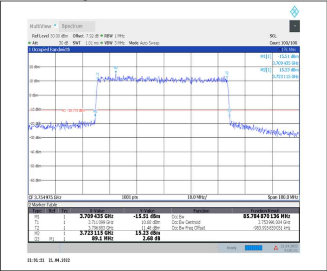
1-N78-3700-3800--30-90-H-1-DFT-QPSK-Outer_Full-240@0-Ant0-85.785-89.100-≤90-PASS
