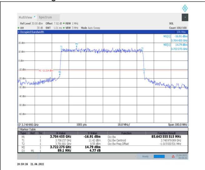
1-N78-3700-3800--30-90-M-2-DFT-PI2BPSK-Outer_Full-240@0-Ant0-85.644-89.100-≤90-PASS
