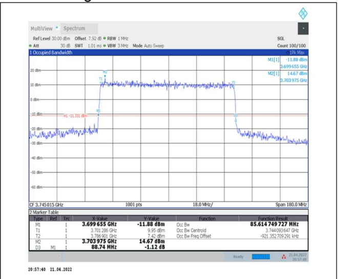
1-N78-3700-3800--30-90-L-3-DFT-16QAM- Outer_Full-240@0-Ant0-85.615-88.740-≤90-PASS
