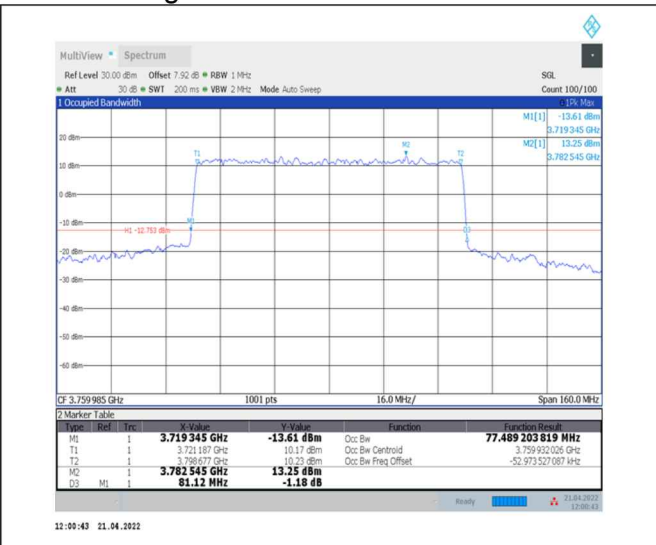
1-N78-3700-3800--30-80-H-8-CP-64QAM-Outer_Full-217@0-Ant0-77.489-81.120-<math>\leq 80</math>-PASS
