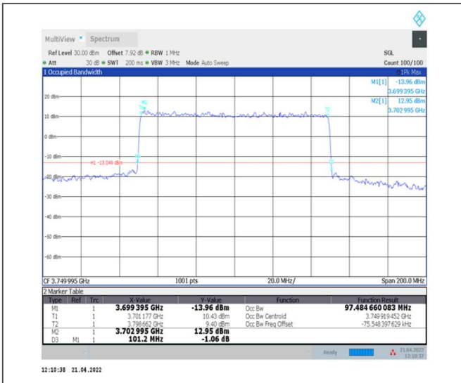
1-N78-3700-3800--30-100-M-6-CP-QPSK- Outer_Full-273@0-Ant0-97.485-101.200-≤100-PASS
