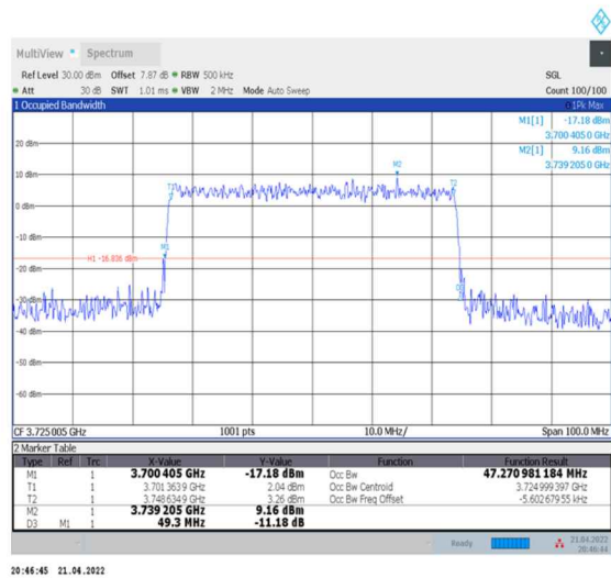
1-N78-3700-3800--30-50-L-9-CP-256QAM-Outer_Full-133@0-Ant0-47.271-49.300-≤50-PASS
