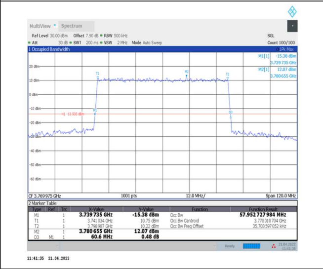
1-N78-3700-3800--30-60-H-4-DFT-64QAM- Outer_Full-162@0-Ant0-57.953-60.600-≤60-PASS
