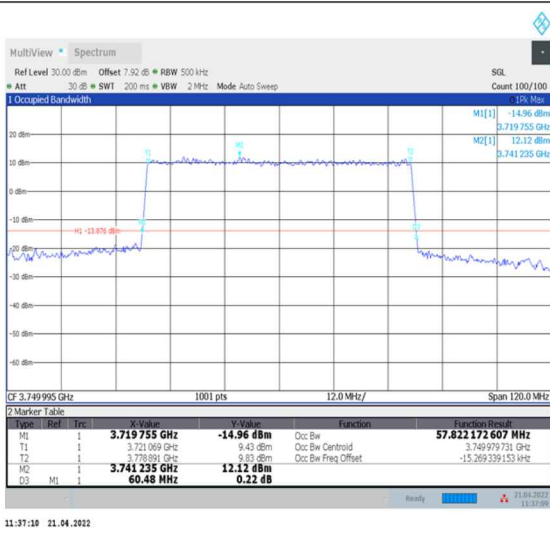
1-N78-3700-3800--30-60-M-6-CP-QPSK-Outer_Full-162@0-Ant0-57.822-60.480-≤60-PASS
