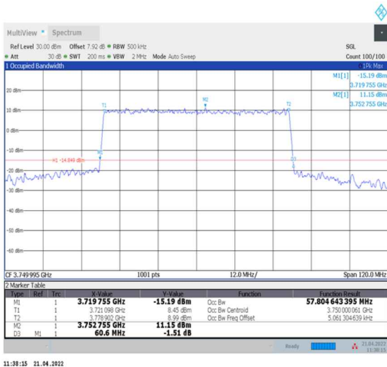
1-N78-3700-3800--30-60-M-8-CP-64QAM-Outer_Full-162@0-Ant0-57.805-60.600-≤60-PASS
