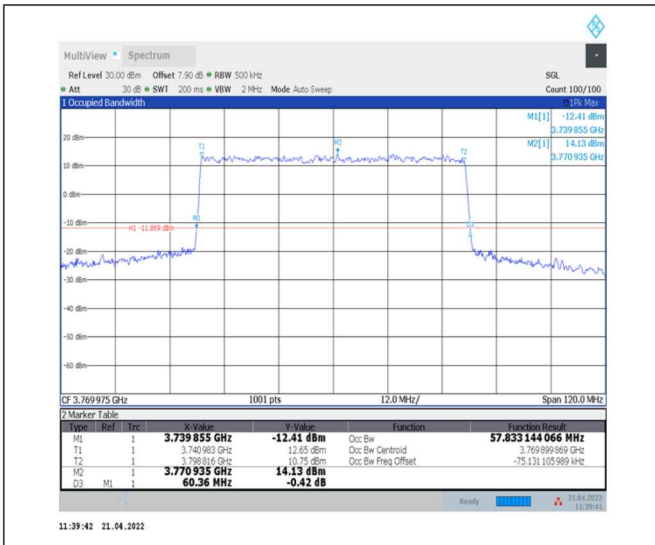
1-N78-3700-3800--30-60-H-1-DFT-QPSK- Outer_Full-162@0-Ant0-57.833-60.360-≤60-PASS
