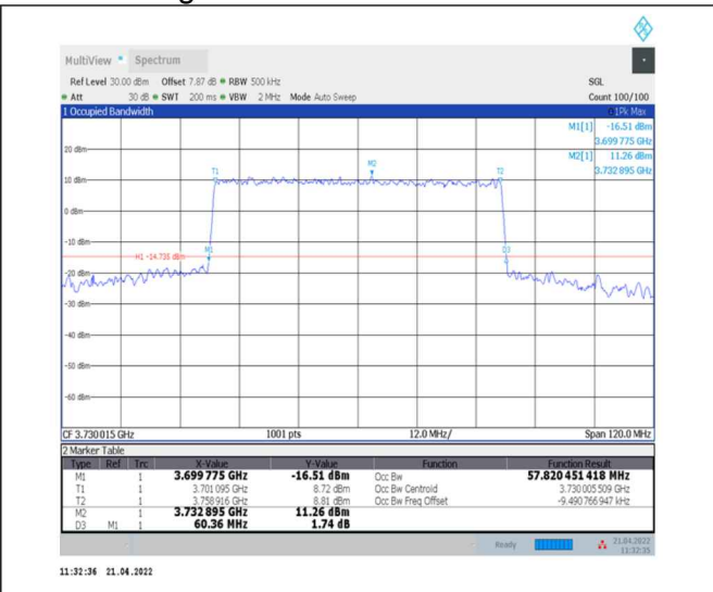
1-N78-3700-3800--30-60-L-8-CP-64QAM-Outer_Full-162@0-Ant0-57.82-60.360-≤60-PASS
