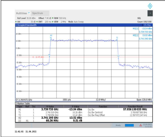
1-N78-3700-3800--30-60-H-3-DFT-16QAM- Outer_Full-162@0-Ant0-57.936-60.360-≤60-PASS
