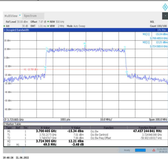
1-N78-3700-3800--30-50-L-7-CP-16QAM-Outer_Full-133@0-Ant0-47.457-49.500-≤50-PASS
