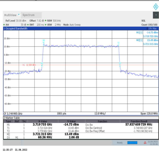
1-N78-3700-3800--30-60-M-3-DFT-16QAM-Outer_Full-162@0-Ant0-57.938-60.360-≤60-PASS
