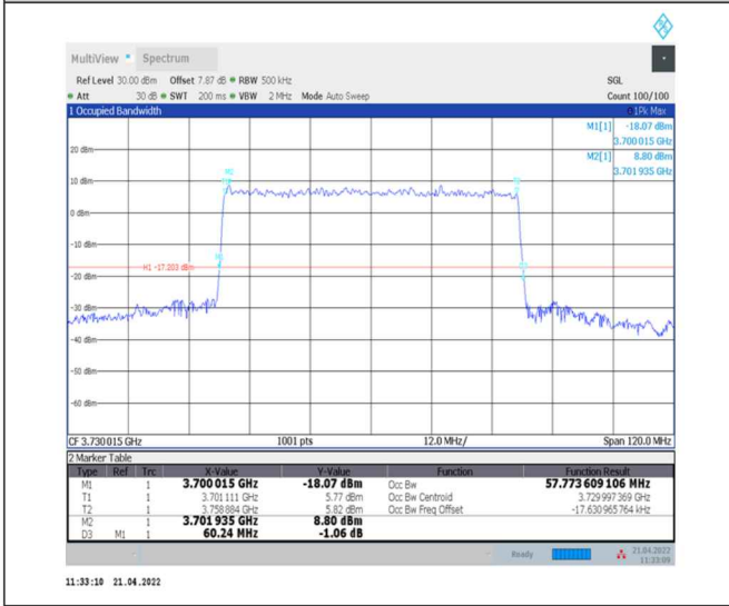
1-N78-3700-3800--30-60-L-9-CP-256QAM-Outer_Full-162@0-Ant0-57.774-60.240-≤60-PASS
