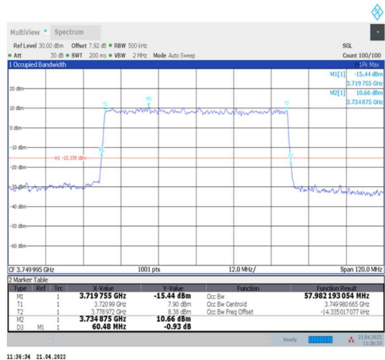
1-N78-3700-3800--30-60-M-5-DFT-256QAM-Outer_Full-162@0-Ant0-57.982-60.480-≤60-PASS
