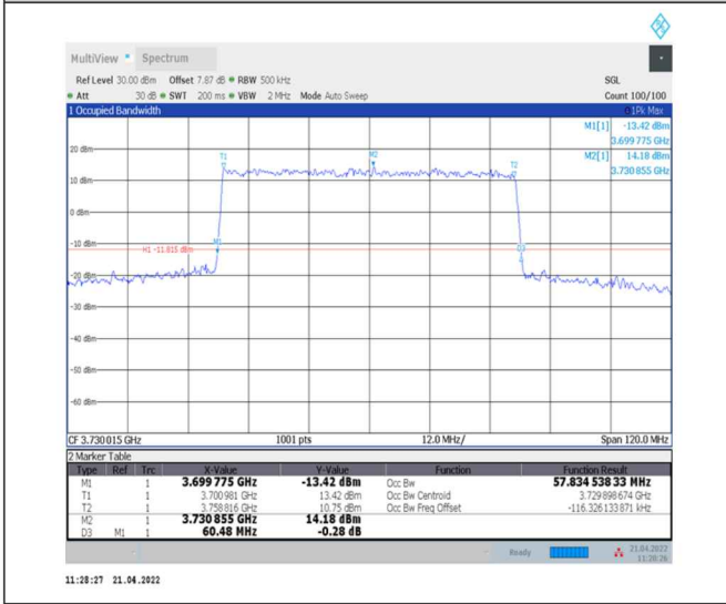
1-N78-3700-3800--30-60-L-1-DFT-QPSK-Outer_Full-162@0-Ant0-57.835-60.480-<math>\leq 60</math>-PASS
