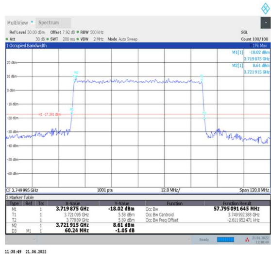
1-N78-3700-3800--30-60-M-9-CP-256QAM-Outer_Full-162@0-Ant0-57.795-60.240-≤60-PASS
