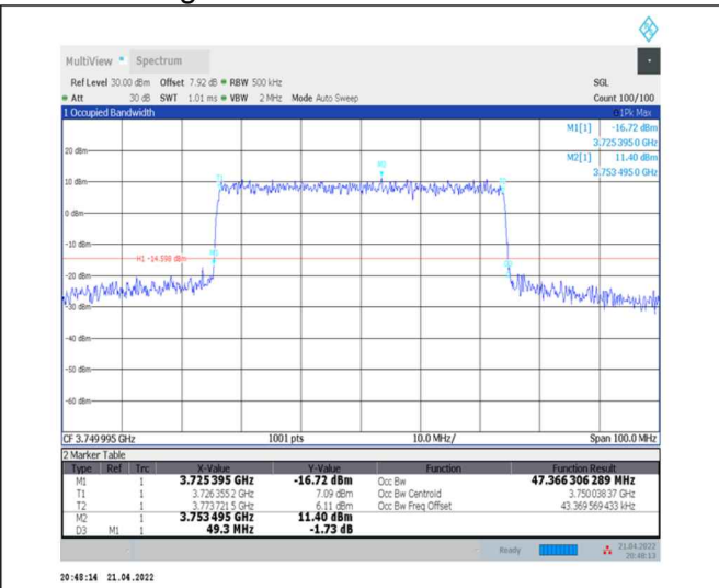
1-N78-3700-3800--30-50-M-6-CP-QPSK-Outer_Full-133@0-Ant0-47.366-49.300-<math>\leq 50</math>-PASS
