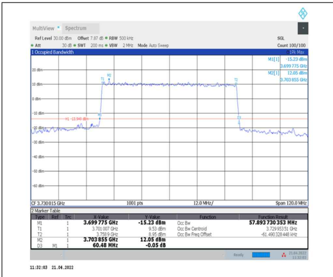
1-N78-3700-3800--30-60-L-7-CP-16QAM-Outer_Full-162@0-Ant0-57.894-60.480-≤60-PASS
