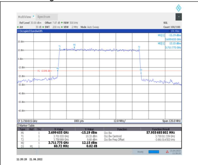
1-N78-3700-3800--30-60-L-4-DFT-64QAM-Outer_Full-162@0-Ant0-57.956-60.720-≤60-PASS
