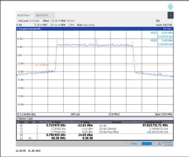
1-N78-3700-3800--30-60-M-1-DFT-QPSK-Outer_Full-162@0-Ant0-57.824-60.360-≤60-PASS
