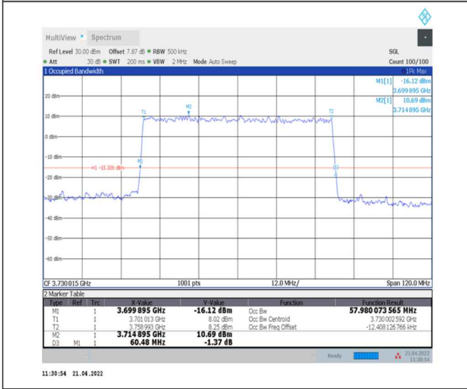
1-N78-3700-3800--30-60-L-5-DFT-256QAM-Outer_Full-162@0-Ant0-57.98-60.480-≤60-PASS
