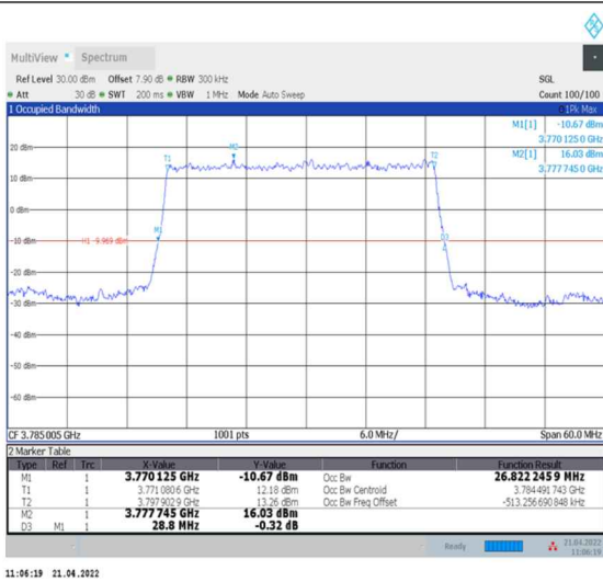
1-N78-3700-3800--30-30-H-2-DFT-PI2BPSK-Outer_Full-75@0-Ant0-26.822-28.800-≤30-PASS
