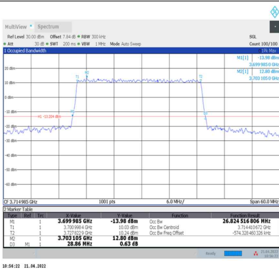
1-N78-3700-3800--30-30-L-4-DFT-64QAM-Outer_Full-75@0-Ant0-26.825-28.860-≤30-PASS
