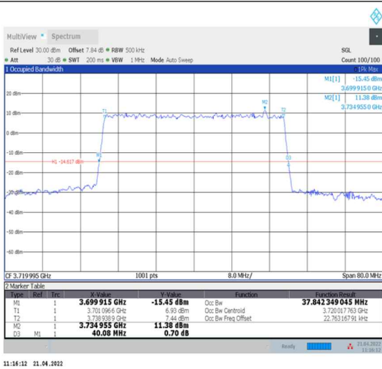
1-N78-3700-3800-30-40-L-9-CP-256QAM-Outer_Full-106@0-Ant0-37.842-40.080-≤40-PASS
