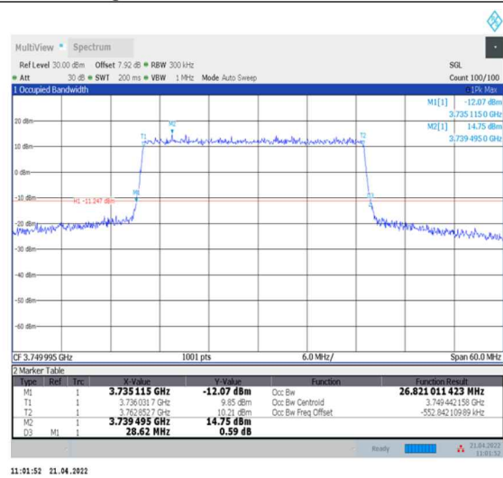
1-N78-3700-3800--30-30-M-4-DFT-64QAM-Outer_Full-75@0-Ant0-26.821-28.620-≤30-PASS
