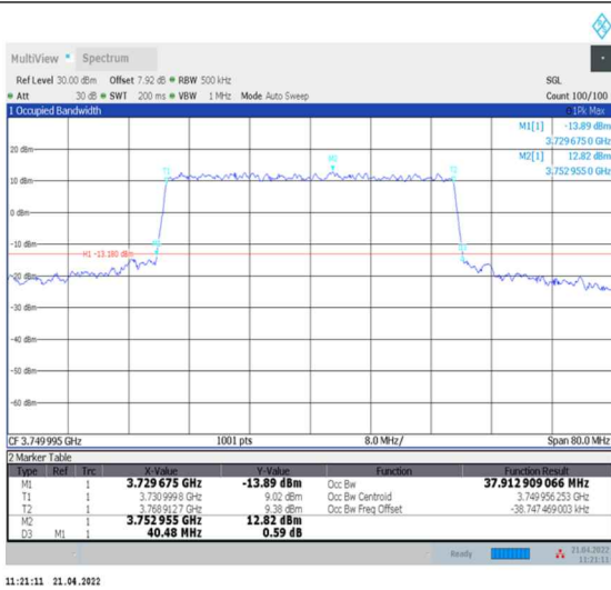
1-N78-3700-3800--30-40-M-8-CP-64QAM-Outer_Full-106@0-Ant0-37.913-40.480-≤40-PASS
