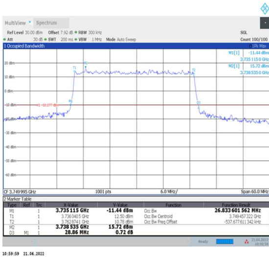
1-N78-3700-3800--30-30-M-1-DFT-QPSK-Outer_Full-75@0-Ant0-26.834-28.860-≤30-PASS
