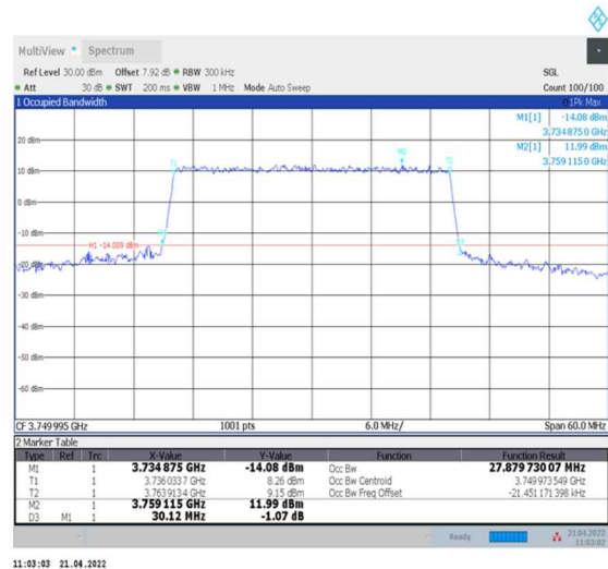
1-N78-3700-3800--30-30-M-6-CP-QPSK-Outer_Full-78@0-Ant0-27.88-30.120-≤30-PASS
