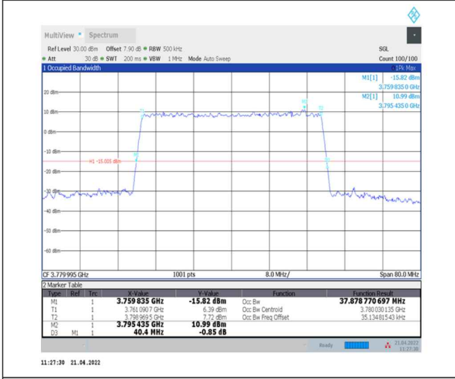
1-N78-3700-3800--30-40-H-9-CP-256QAM-Outer_Full-106@0-Ant0-37.879-40.400-≤40-PASS
