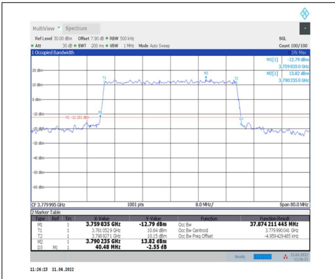
1-N78-3700-3800--30-40-H-7-CP-16QAM-Outer_Full-106@0-Ant0-37.874-40.480-≤40-PASS
