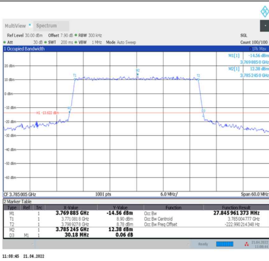
1-N78-3700-3800--30-30-H-6-CP-QPSK-Outer_Full-78@0-Ant0-27.846-30.180-≤30-PASS
