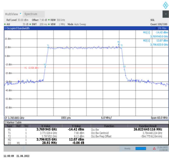
1-N78-3700-3800--30-30-H-5-DFT-256QAM-Outer_Full-75@0-Ant0-26.824-28.920-≤30-PASS
