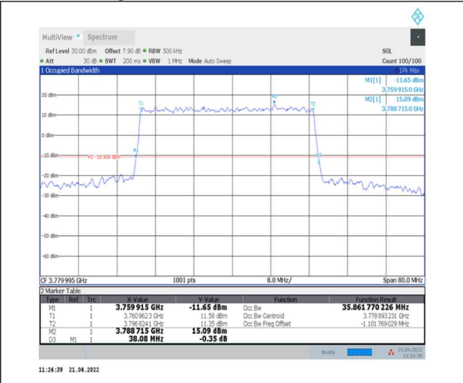
1-N78-3700-3800--30-40-H-4-DFT-64QAM-Outer_Full-100@0-Ant0-35.862-38.080-<math>\leq 40</math>-PASS
