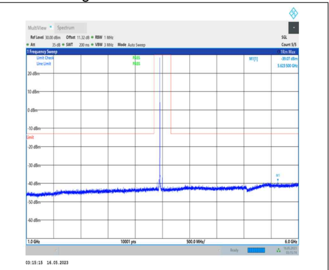
1-N78-3450-3550-PC1-30-100-M-1-DFT-PI2BPSK- Inner_1RB_Left-1@1-1000-6000-Ant0-5623.50--39.07--13-PASS
