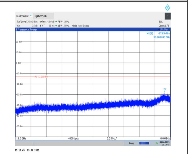
1-N78-3450-3550-PC1-30-100-M-1-DFT-PI2BPSK- Inner_1RB_Left-1@1-18000-40000-Ant0-18000.00--61.78--13-PASS
