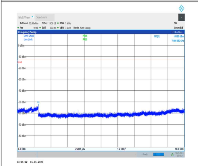
1-N78-3450-3550-PC1-30-100-M-1-DFT-PI2BPSK- Inner_1RB_Left-1@1-6000-18000-Ant0-7495.68--53.80--13-PASS
